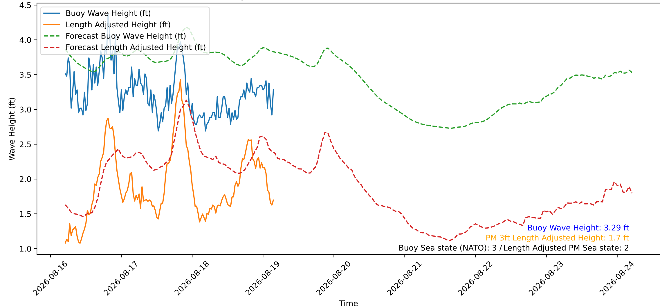
Wave Heights over Time for Green Beach at 2026-08-19 04:31:08
