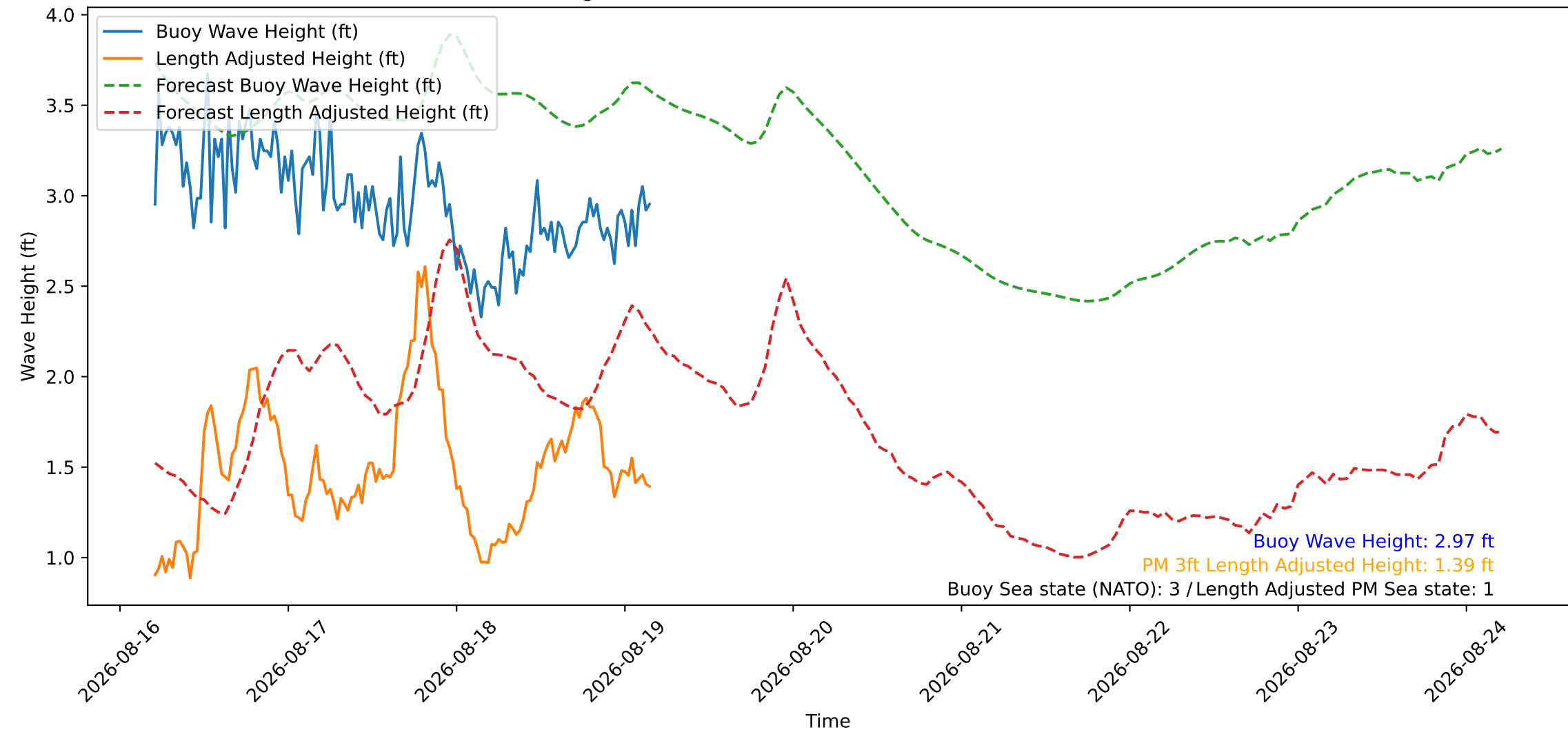
Wave Heights over Time for Red Beach at 2026-08-19 04:30:46
