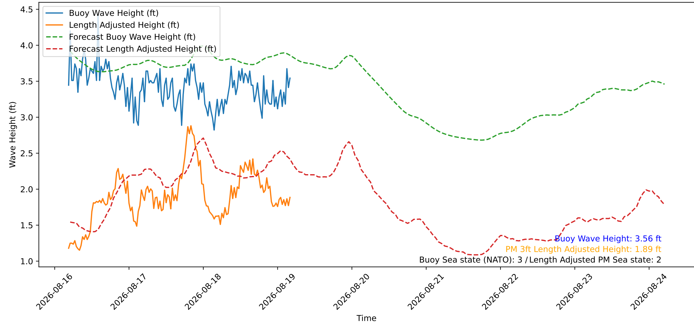
Wave Heights over Time for Oceanside Harbor at 2026-08-19 04:30:26
