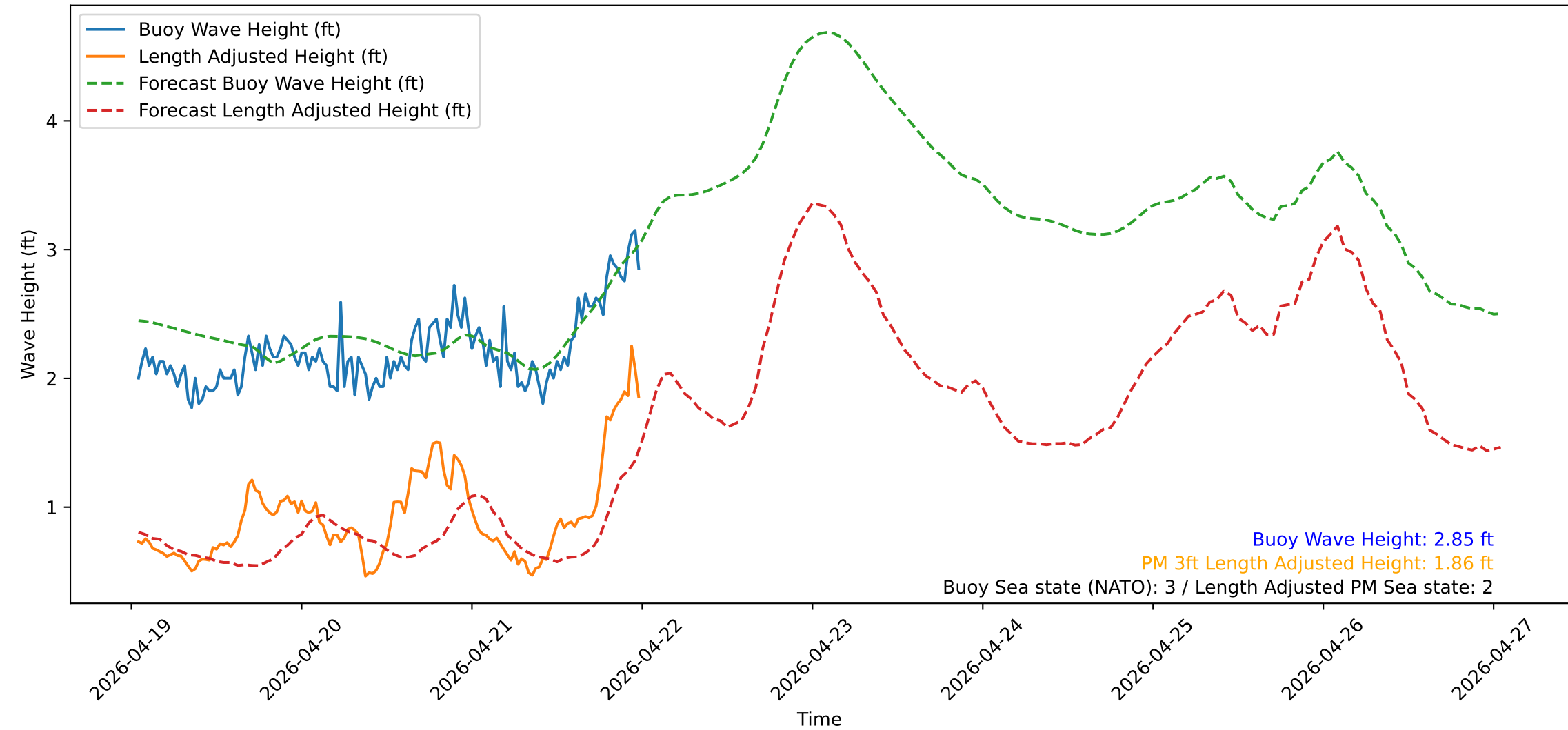
Wave Heights over Time for Red Beach at 2026-04-22 00:30:51
