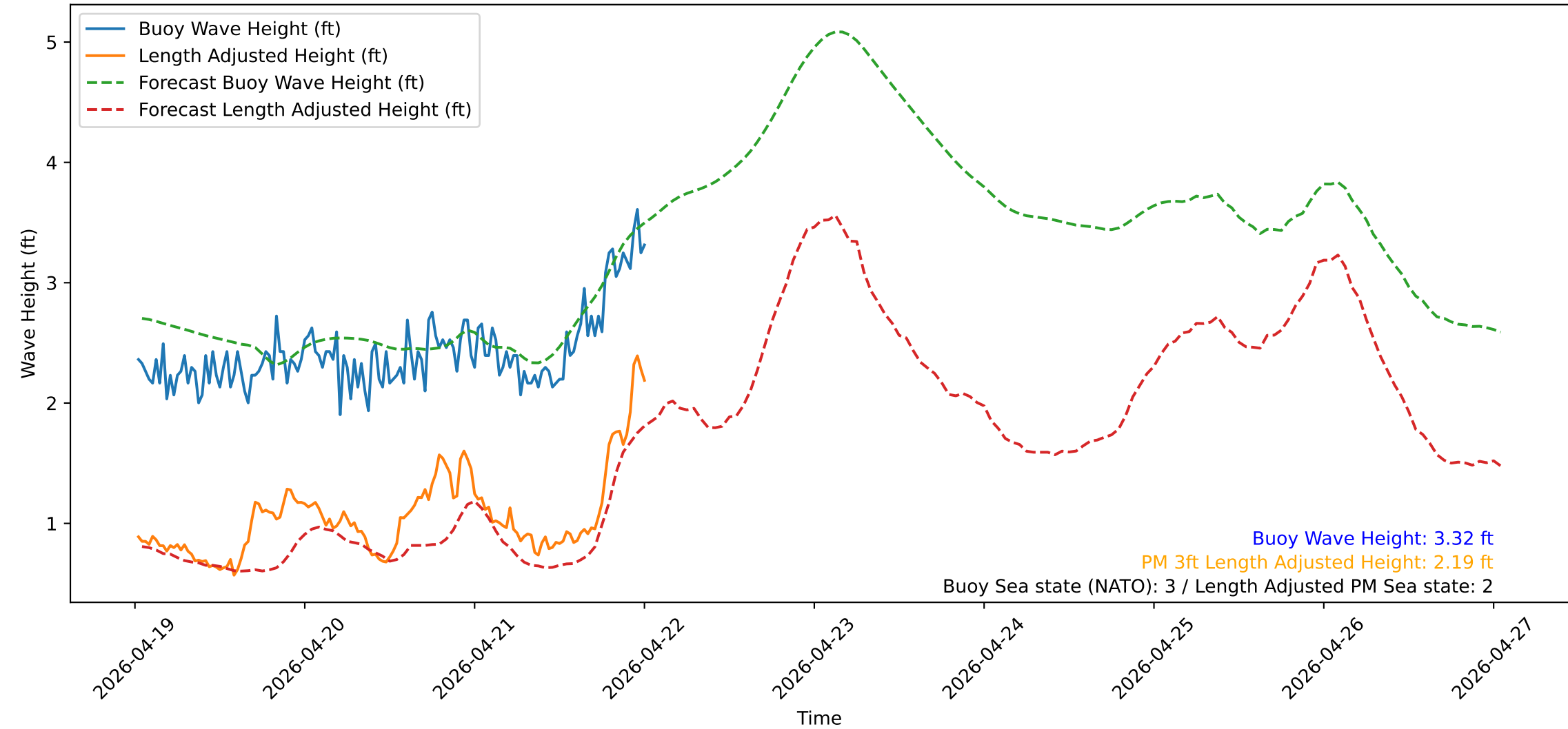
Wave Heights over Time for Oceanside Harbor at 2026-04-22 00:30:31
