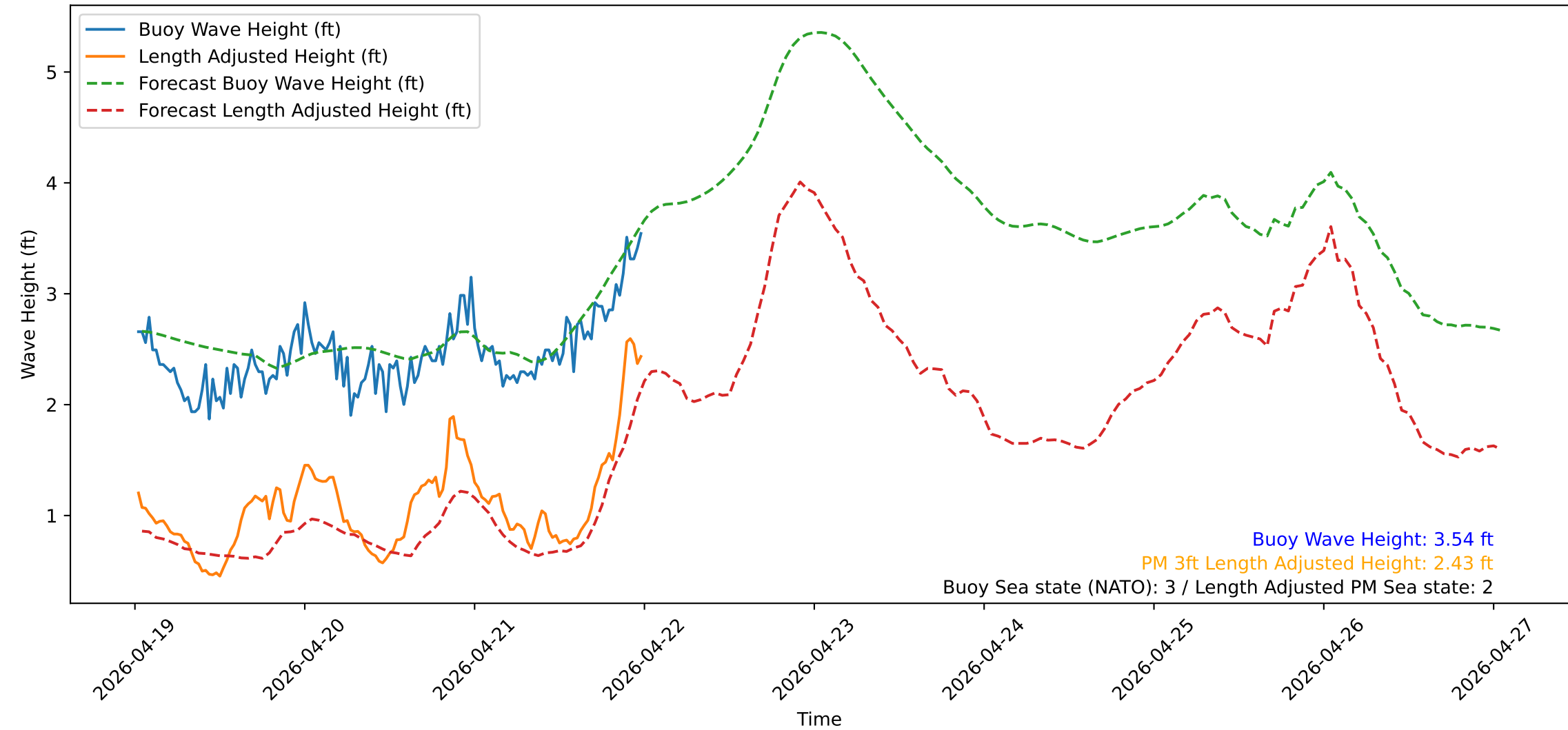
Wave Heights over Time for Green Beach at 2026-04-22 00:31:12
