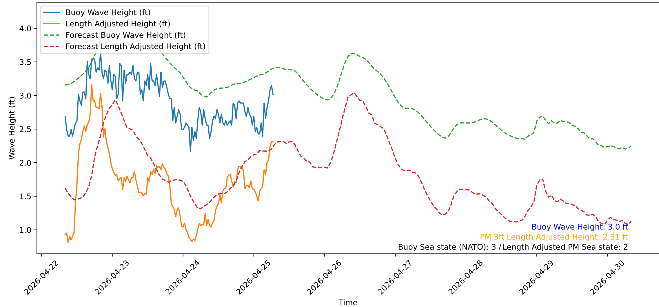
Wave Heights over Time for Red Beach at 2026-04-25 07:40:52
