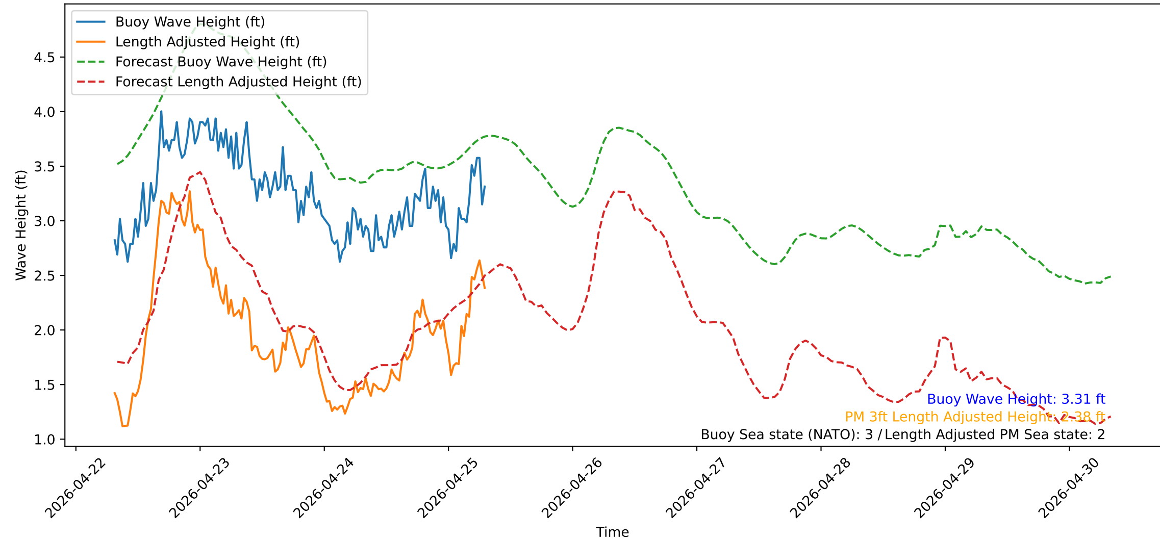
Wave Heights over Time for Green Beach at 2026-04-25 07:41:14
