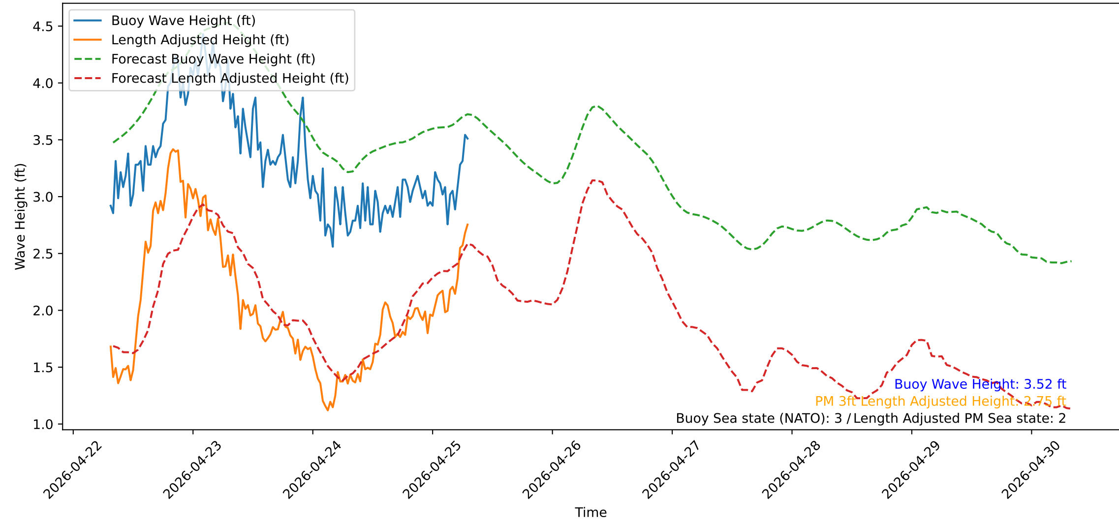
Wave Heights over Time for Oceanside Harbor at 2026-04-25 07:40:32
