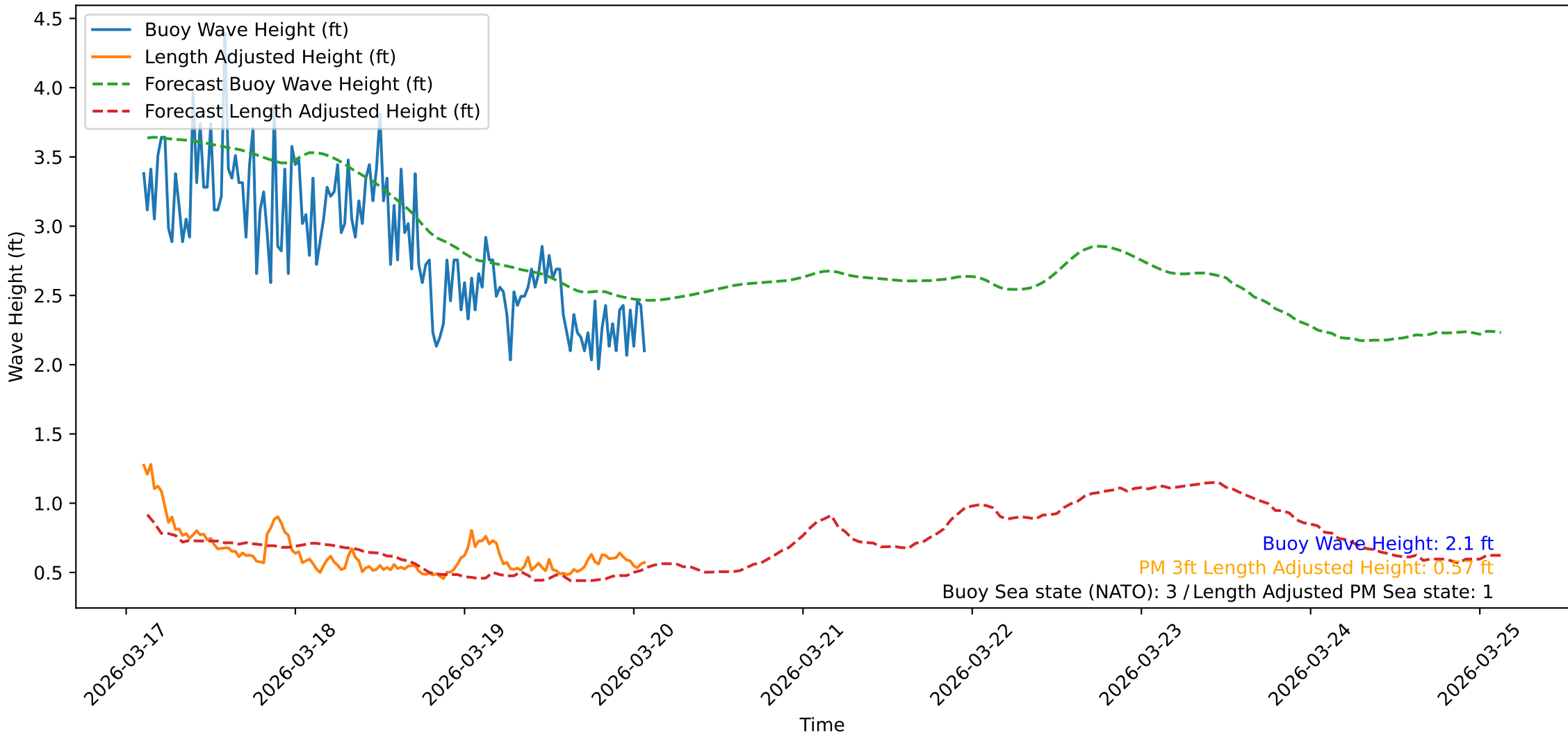
Wave Heights over Time for Oceanside Harbor at 2026-03-20 02:30:31
