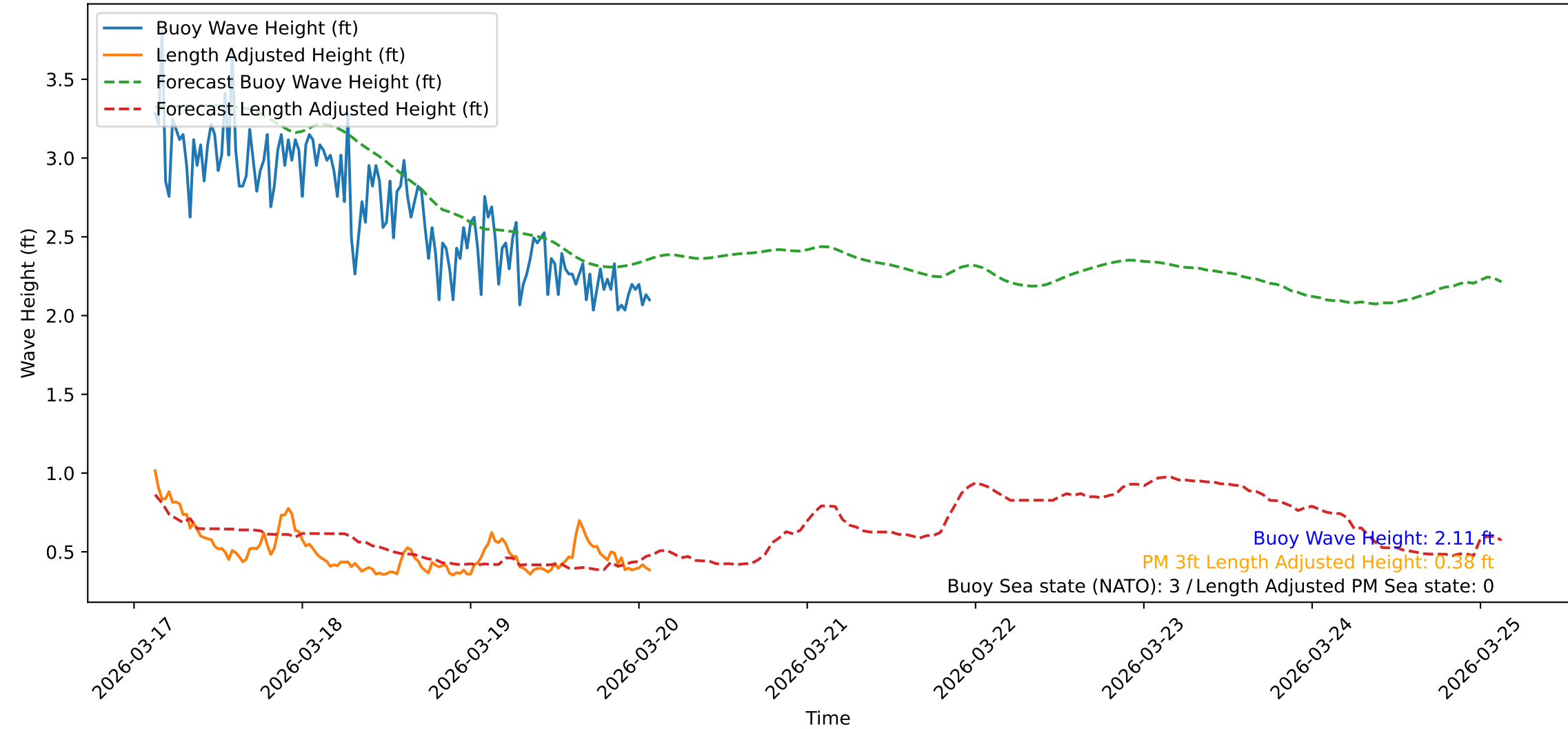
Wave Heights over Time for Red Beach at 2026-03-20 02:30:47
