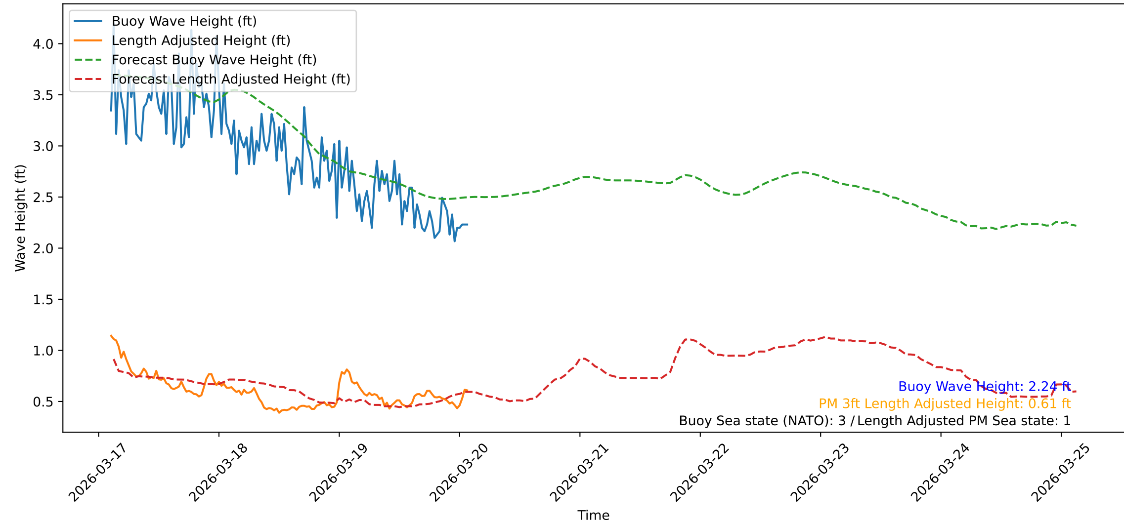
Wave Heights over Time for Green Beach at 2026-03-20 02:31:09
