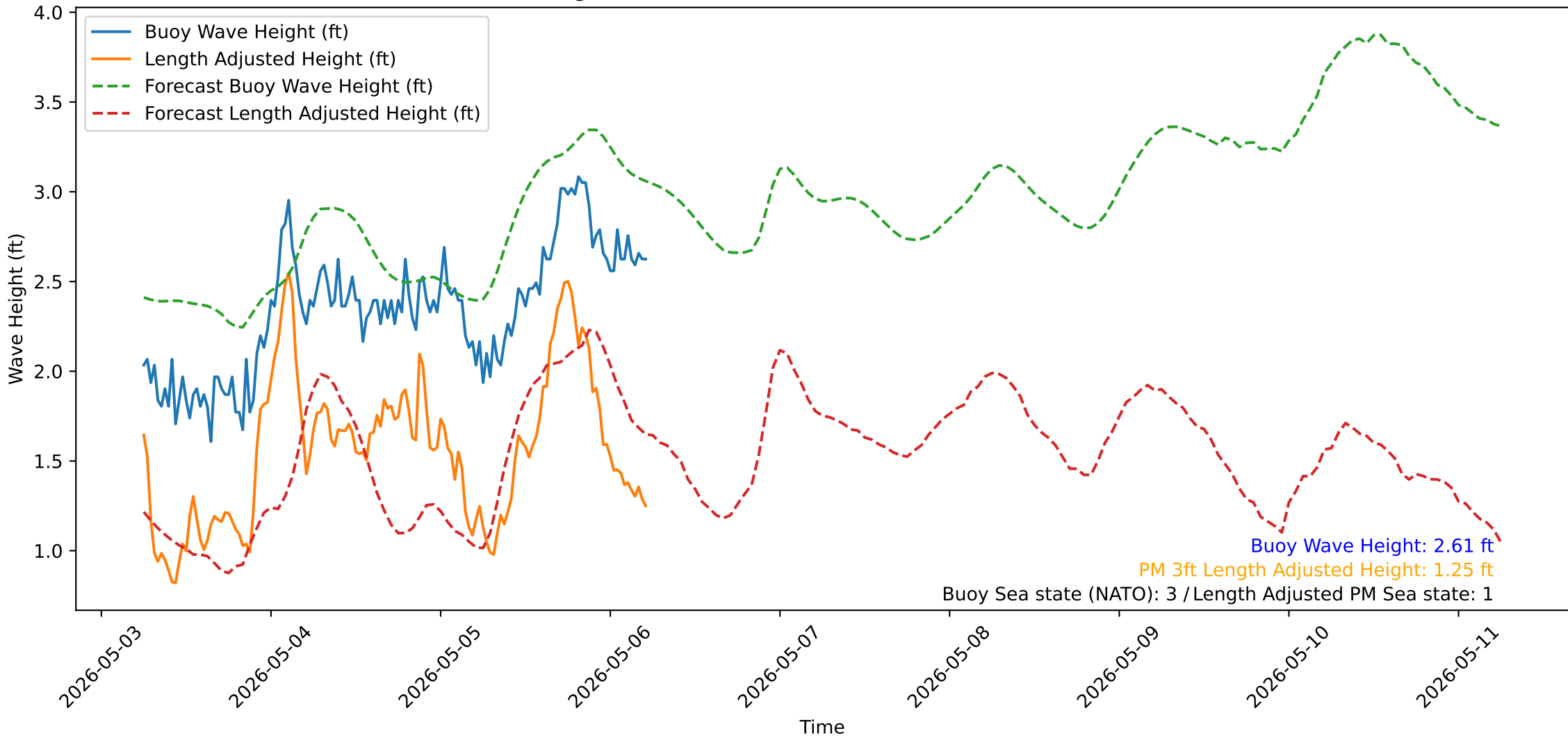
Wave Heights over Time for Red Beach at 2026-05-06 05:50:51
