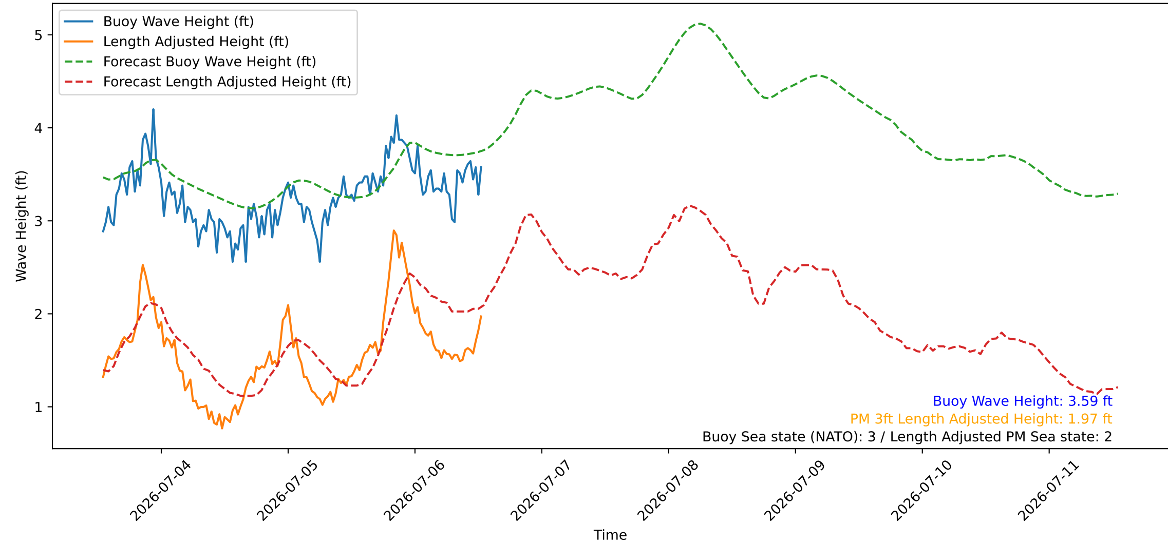
Wave Heights over Time for Green Beach at 2026-07-06 13:11:09
