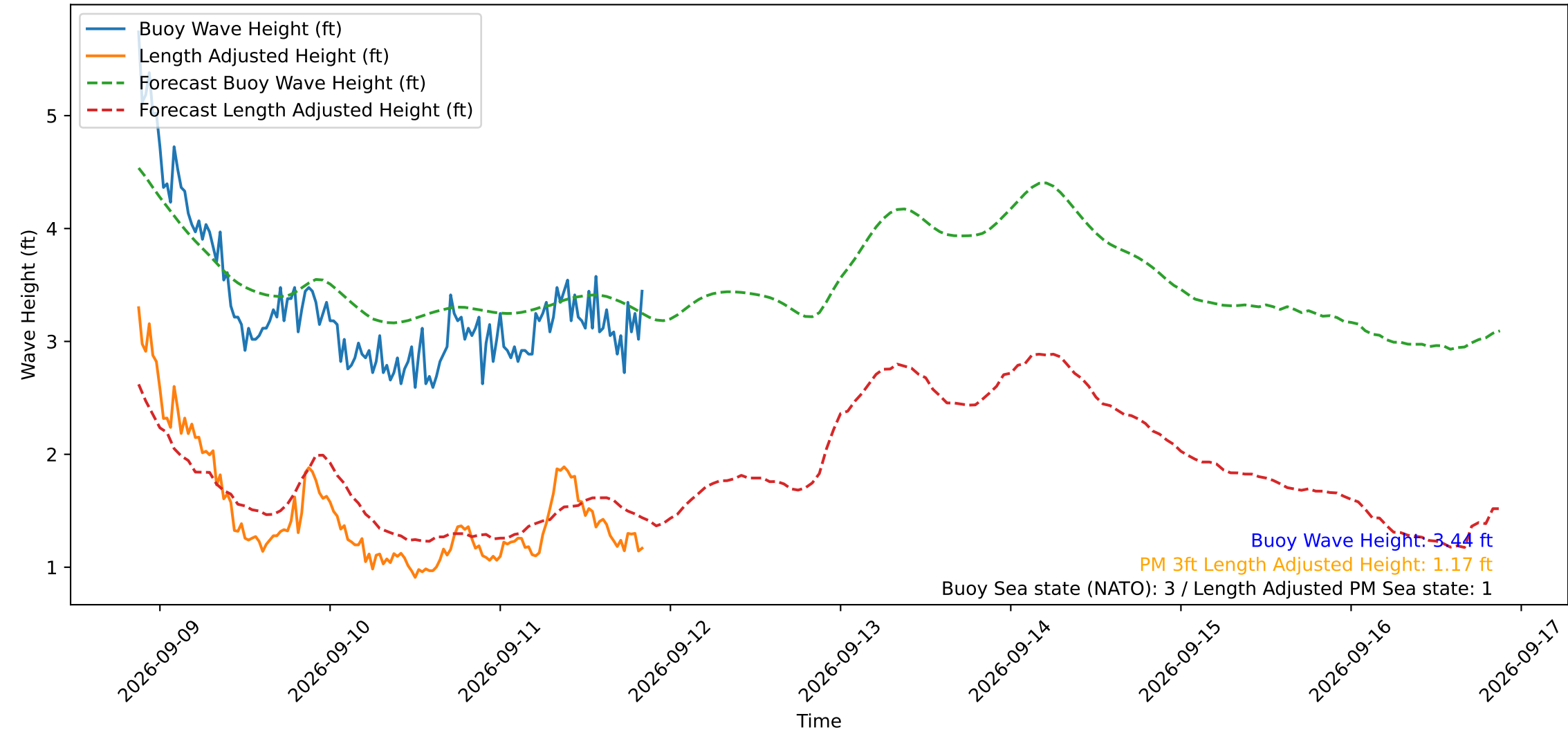
Wave Heights over Time for Green Beach at 2026-09-11 20:41:12
