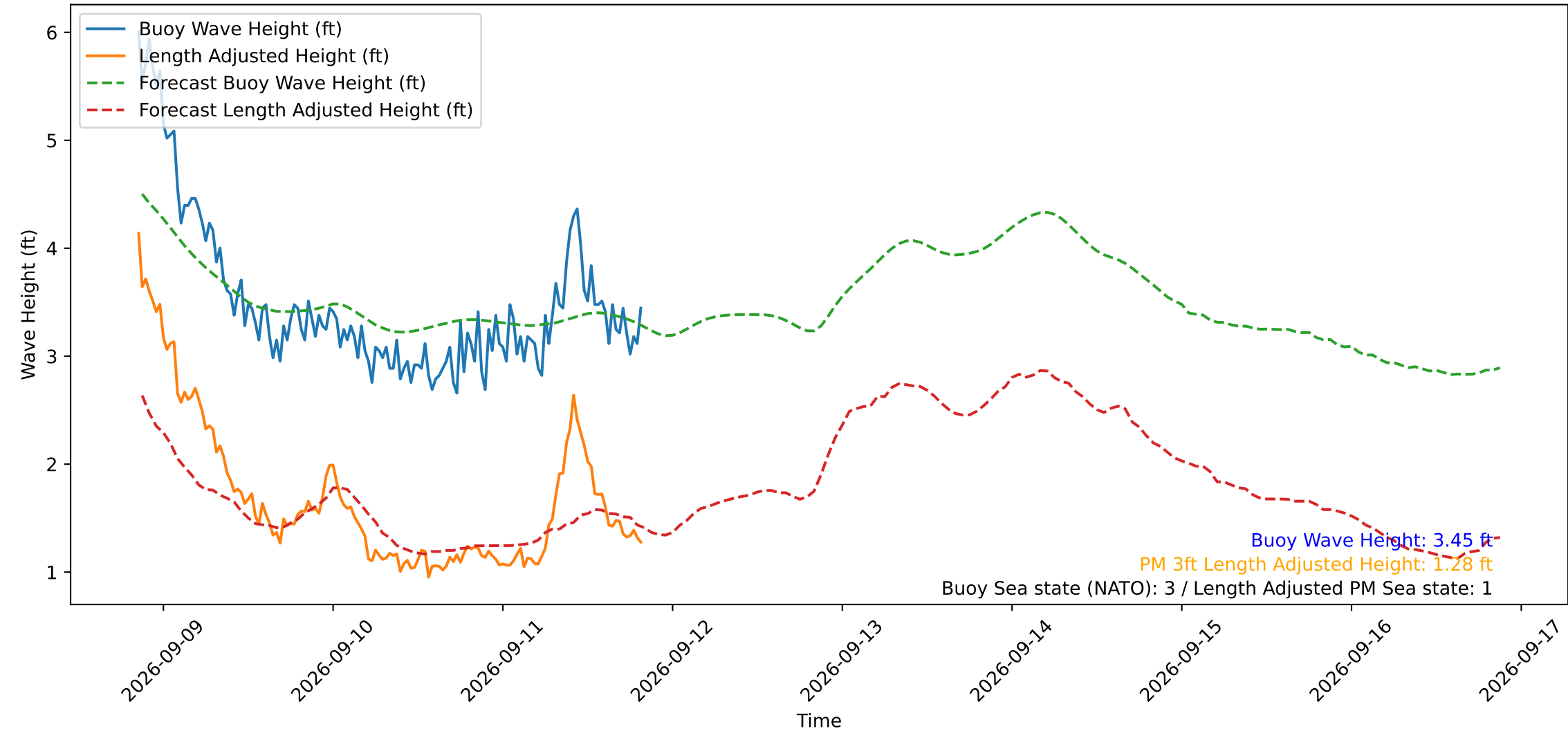
Wave Heights over Time for Oceanside Harbor at 2026-09-11 20:40:29
