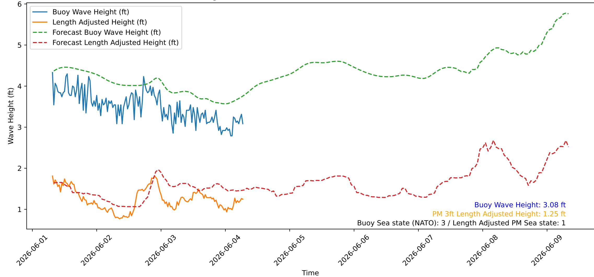
Wave Heights over Time for Green Beach at 2026-06-04 07:31:08
