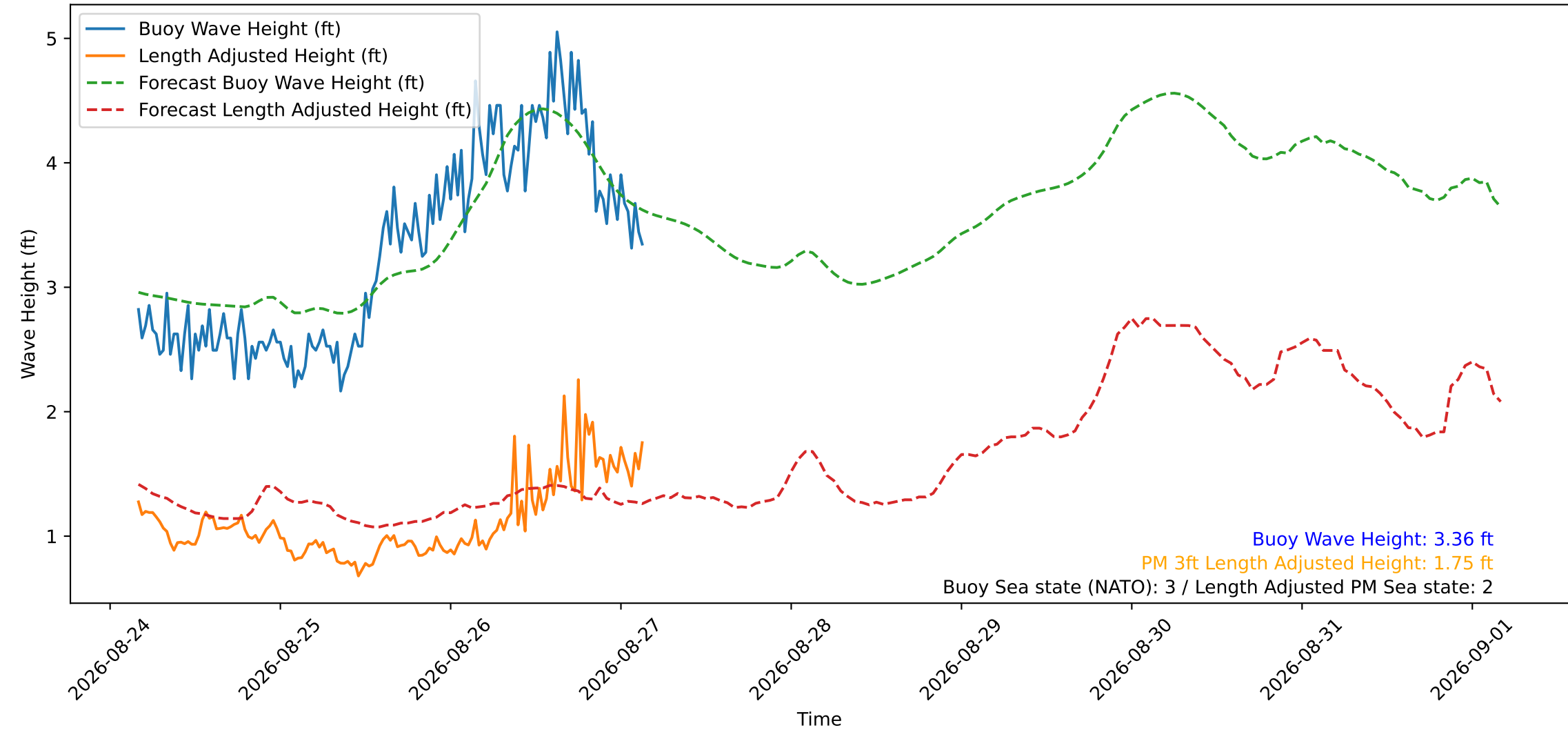
Wave Heights over Time for Red Beach at 2026-08-27 03:40:49
