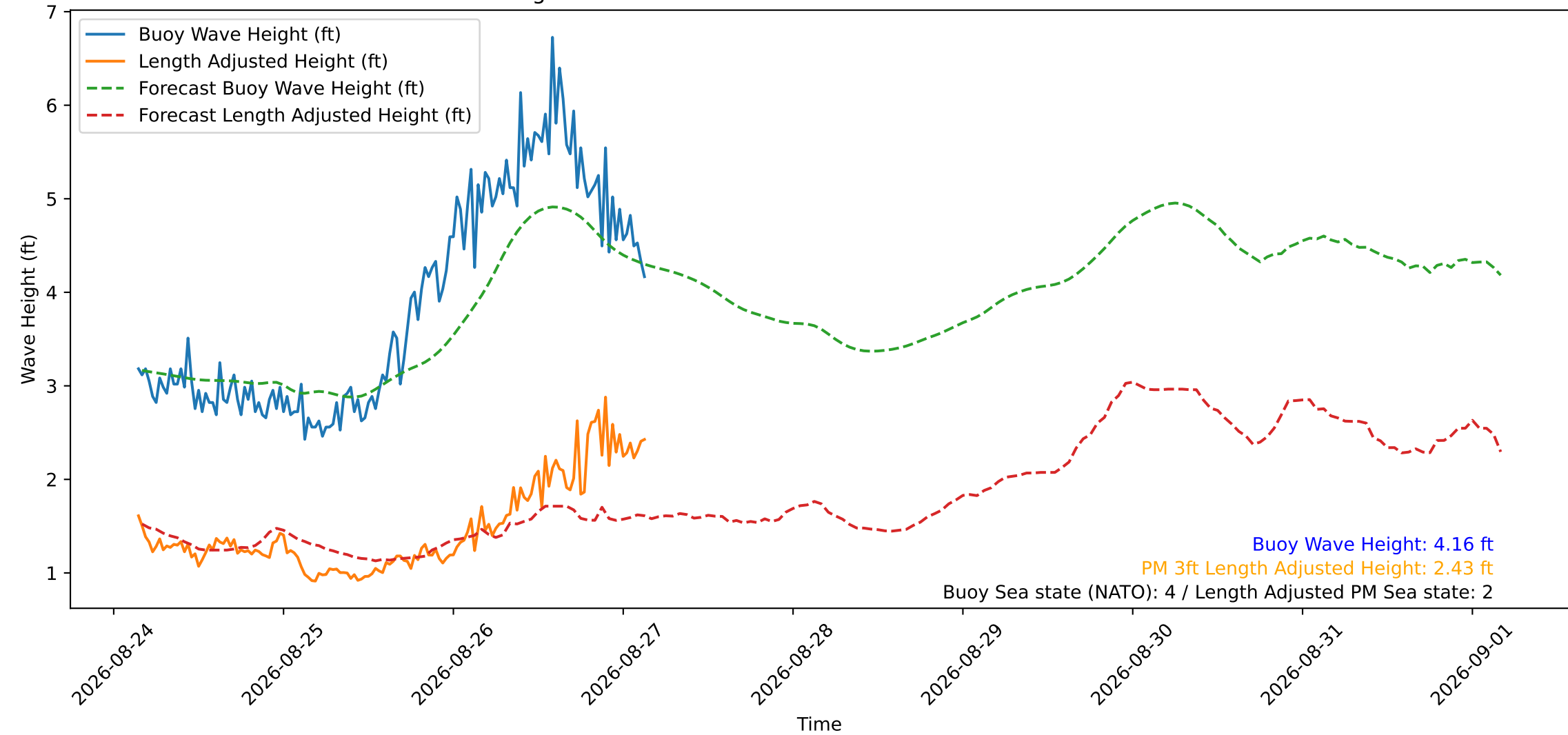
Wave Heights over Time for Oceanside Harbor at 2026-08-27 03:40:30
