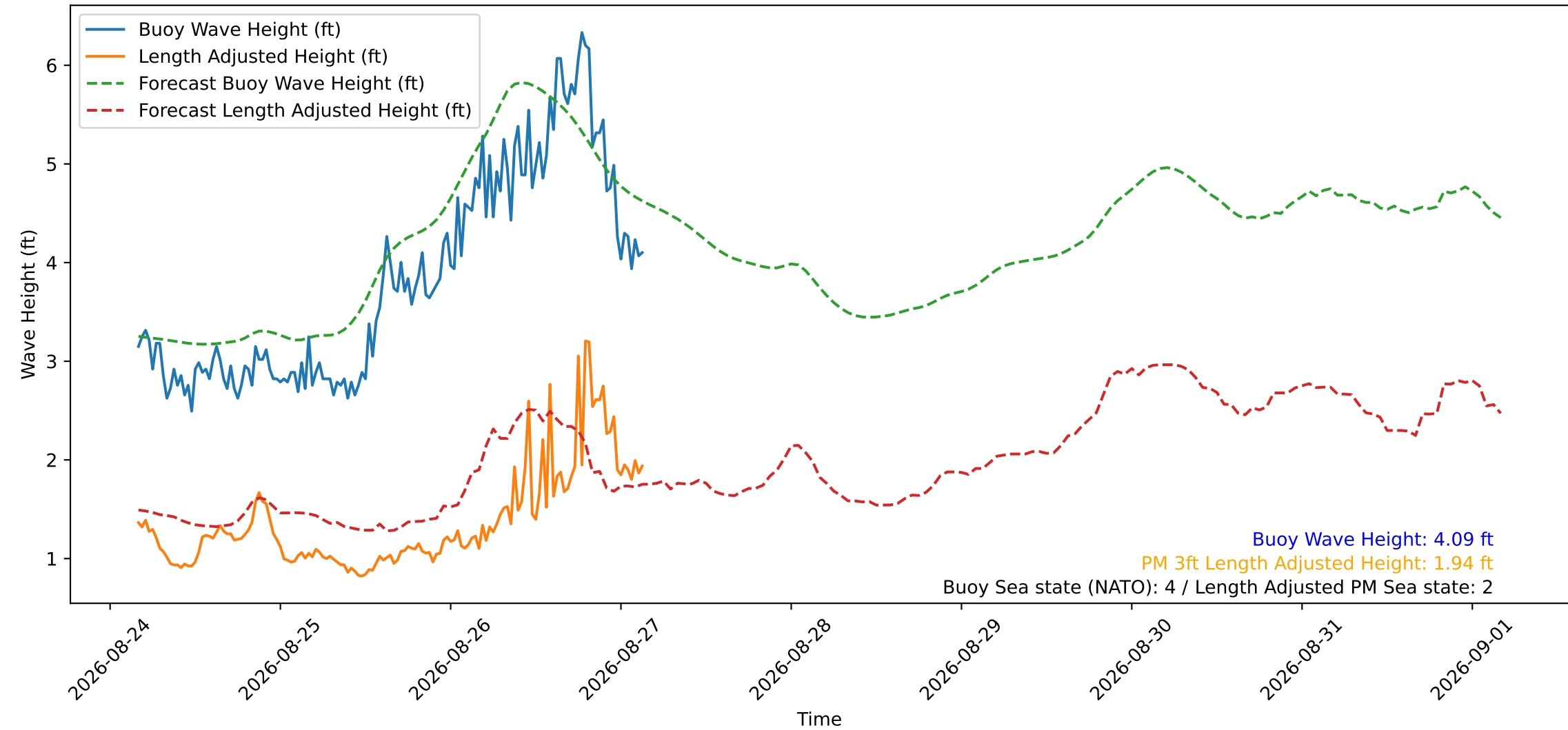
Wave Heights over Time for Green Beach at 2026-08-27 03:41:12
