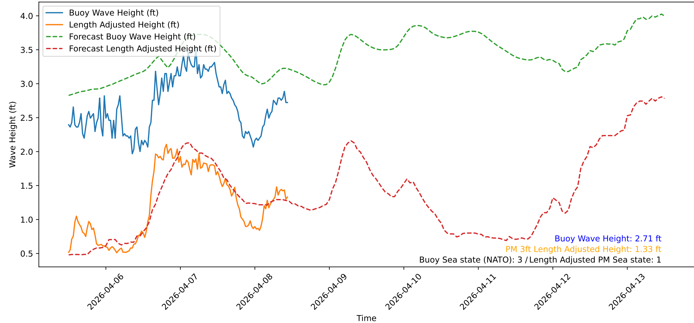
Wave Heights over Time for Red Beach at 2026-04-08 11:30:47
