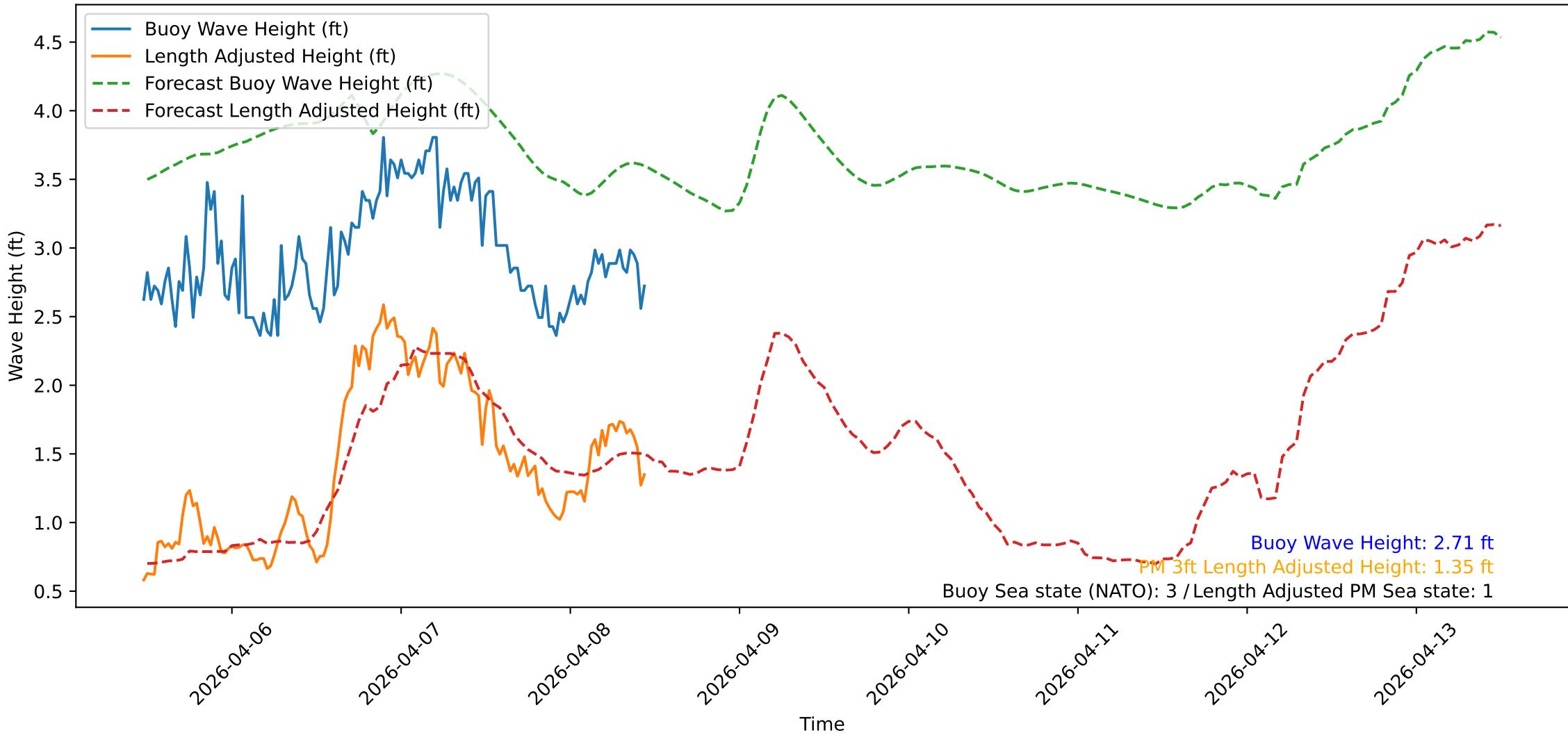
Wave Heights over Time for Green Beach at 2026-04-08 11:31:09
