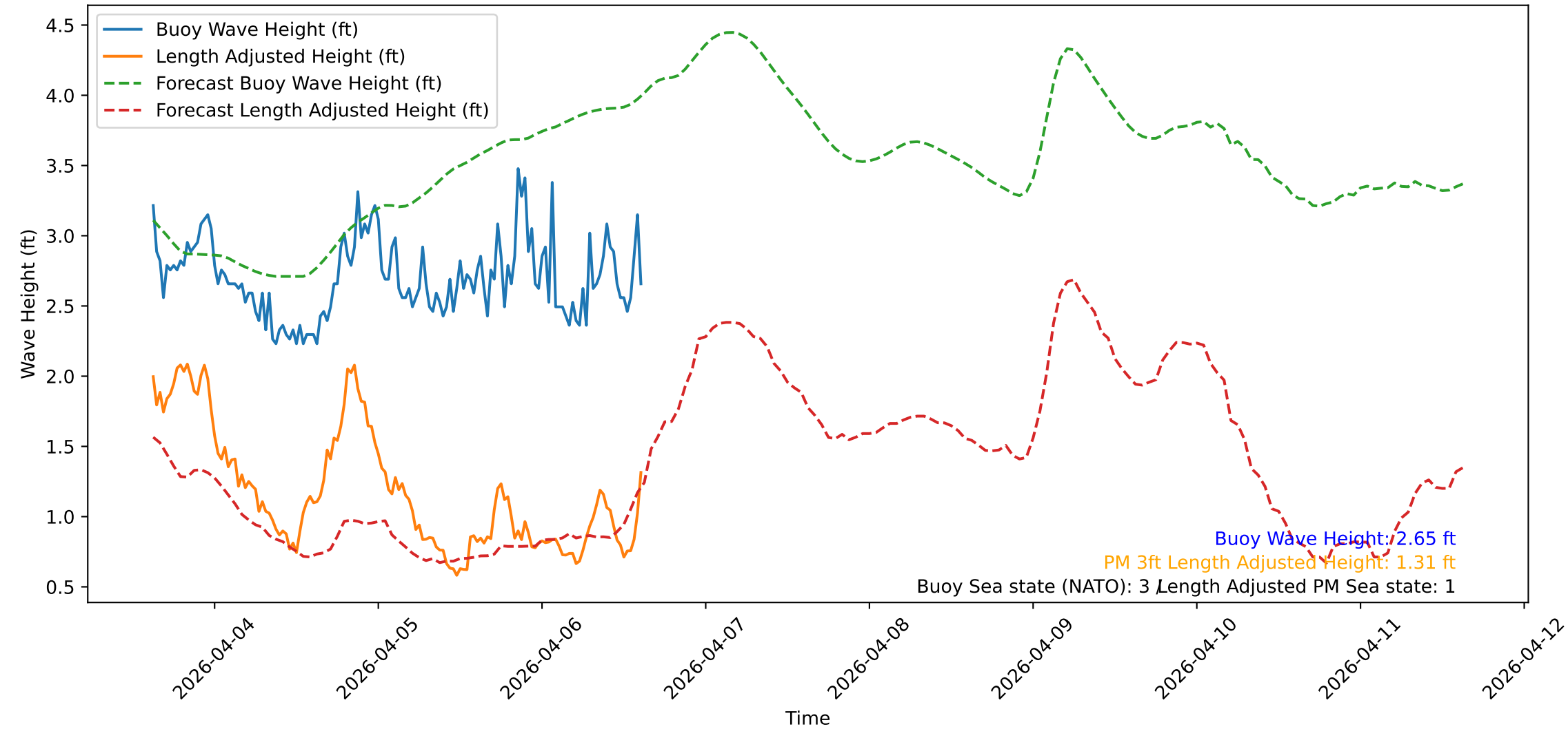
Wave Heights over Time for Green Beach at 2026-04-06 15:11:09
