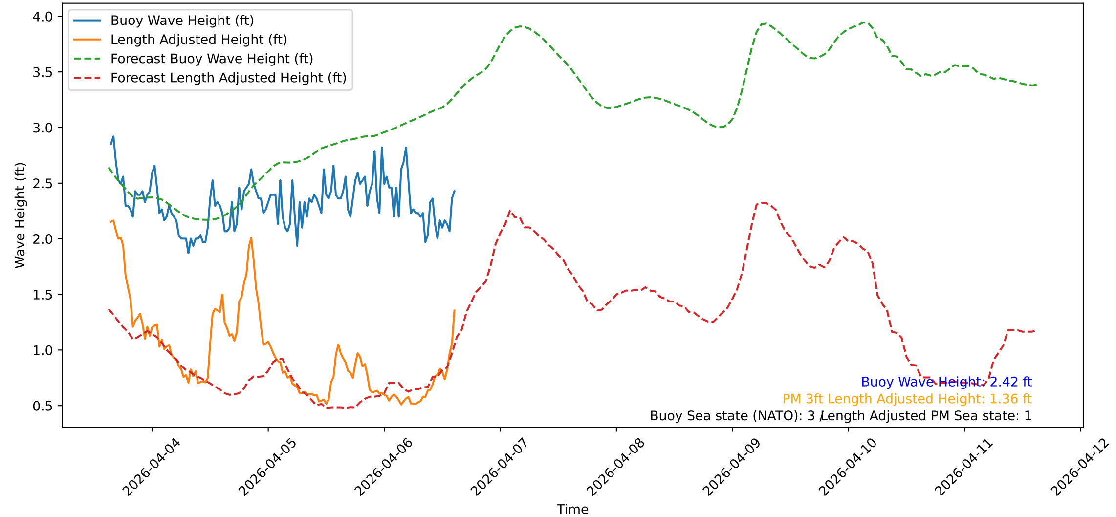
Wave Heights over Time for Red Beach at 2026-04-06 15:10:47
