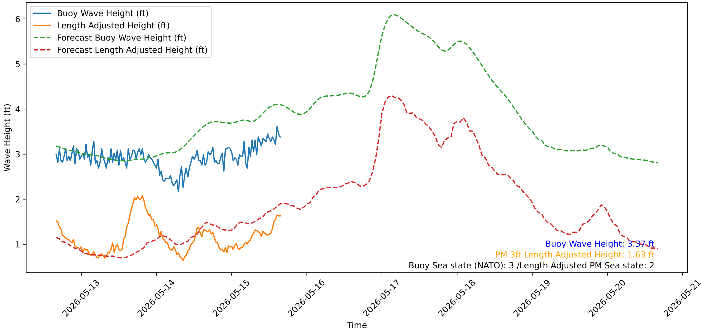
Wave Heights over Time for Oceanside Harbor at 2026-05-15 16:00:32
