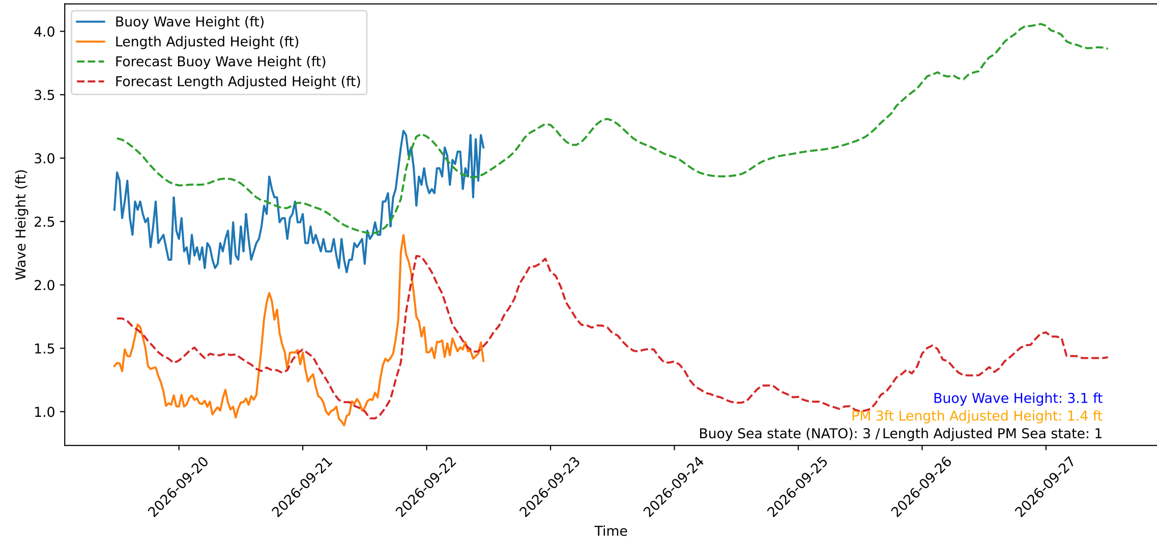
Wave Heights over Time for Oceanside Harbor at 2026-09-22 11:30:30
