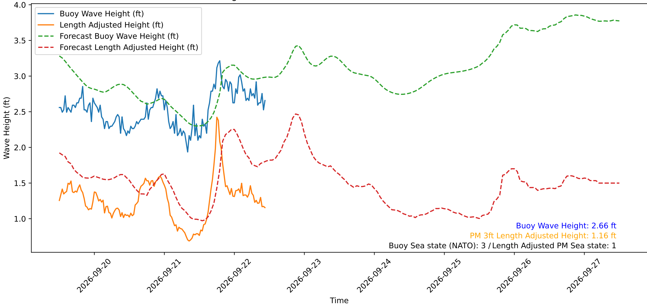
Wave Heights over Time for Green Beach at 2026-09-22 11:31:12
