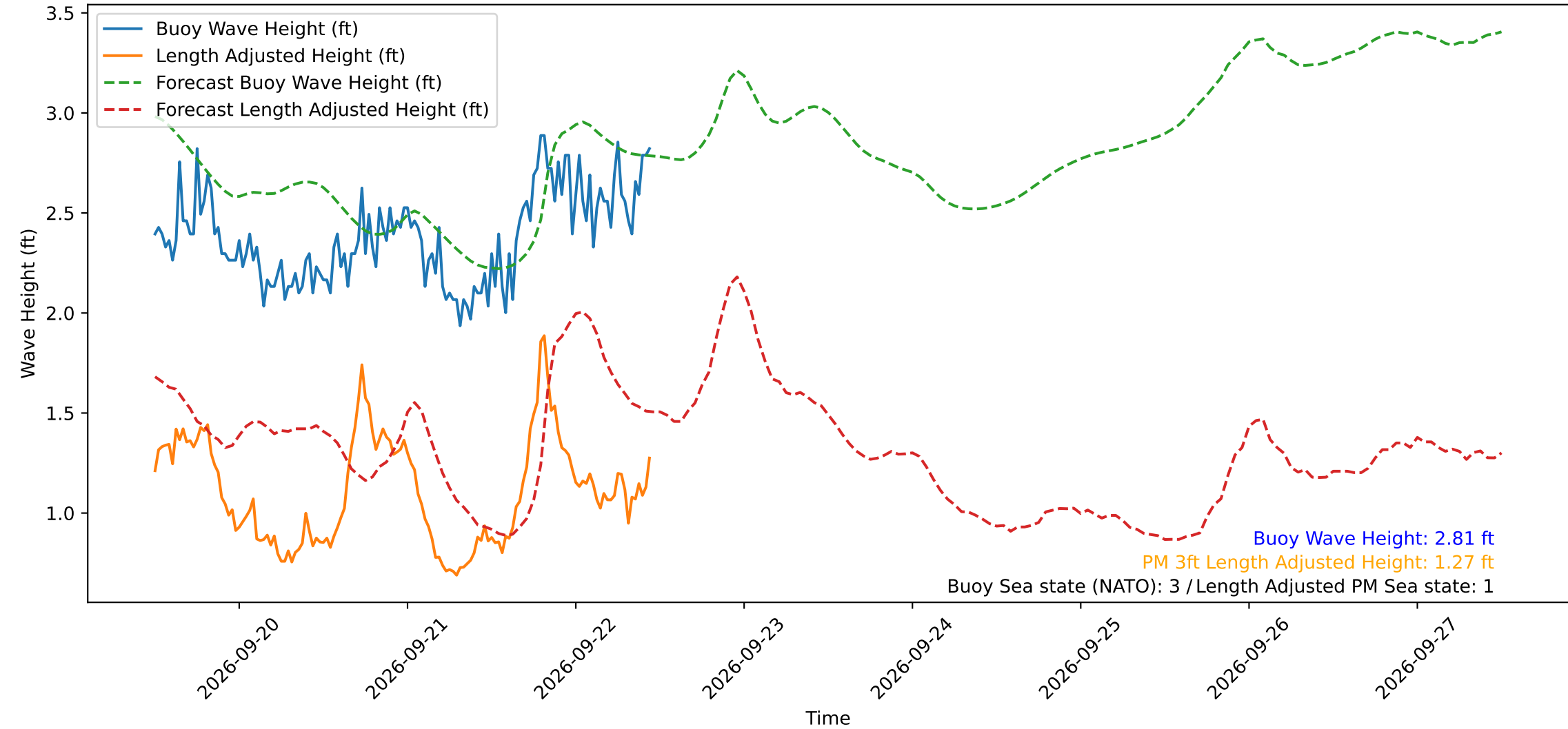
Wave Heights over Time for Red Beach at 2026-09-22 11:30:50
