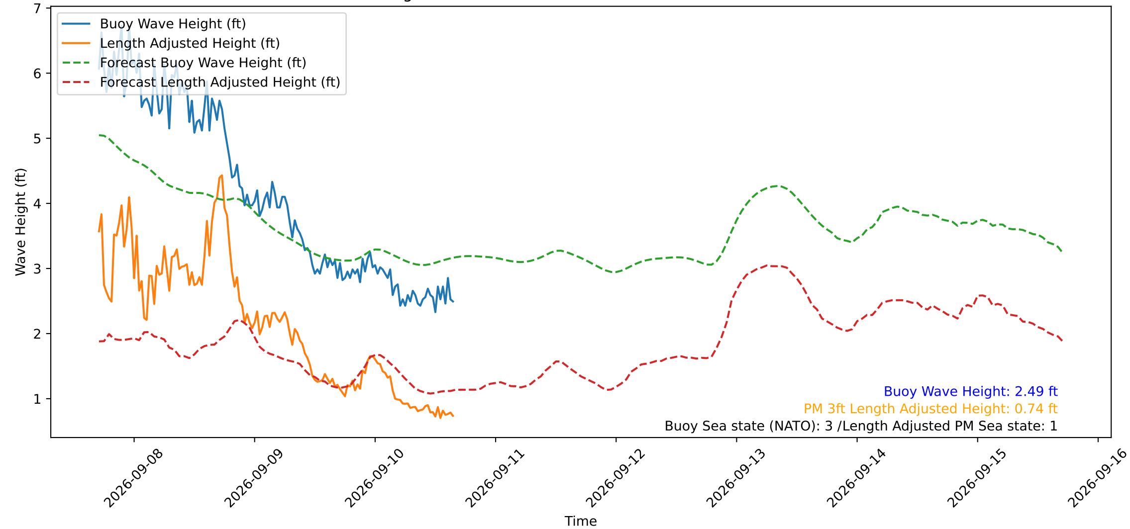
Wave Heights over Time for Red Beach at 2026-09-10 16:30:48
