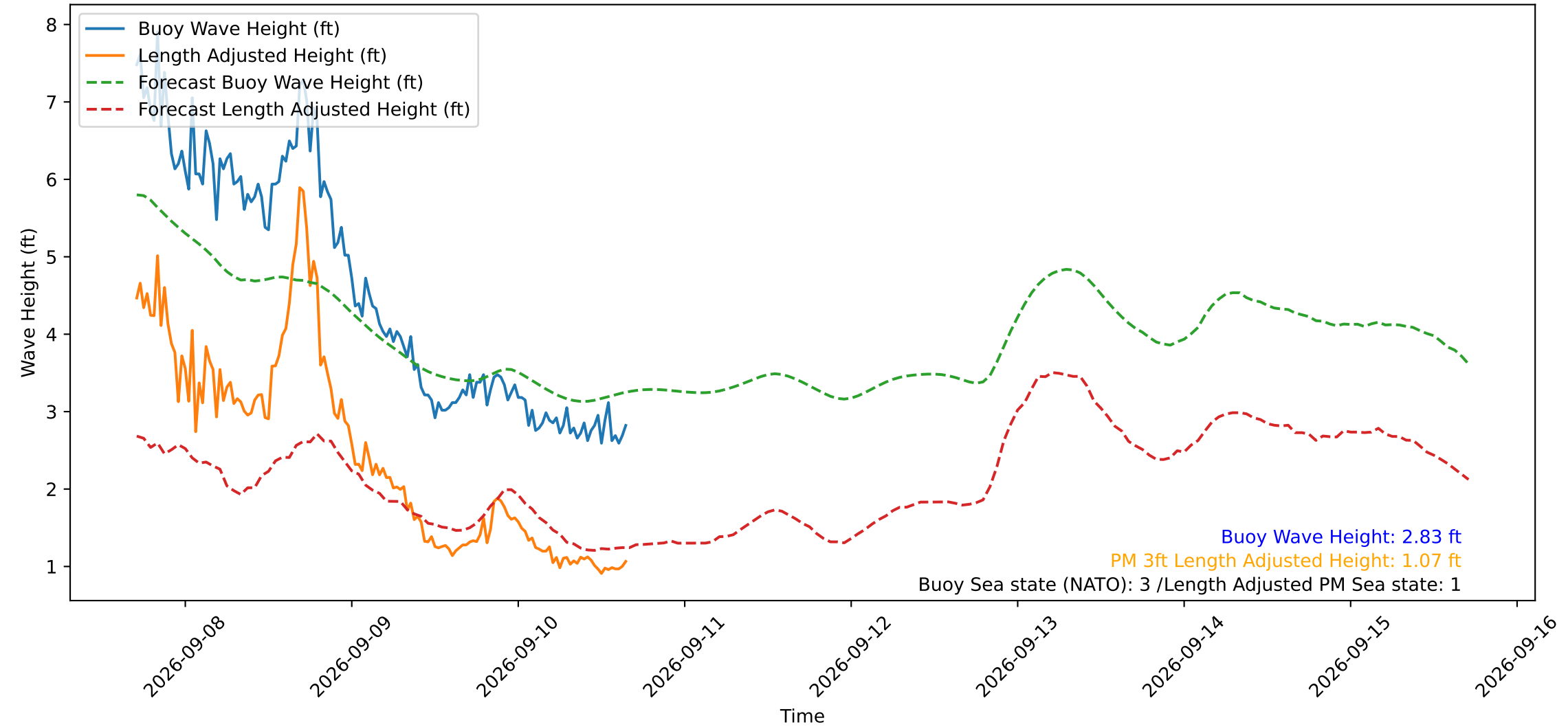
Wave Heights over Time for Green Beach at 2026-09-10 16:31:10
