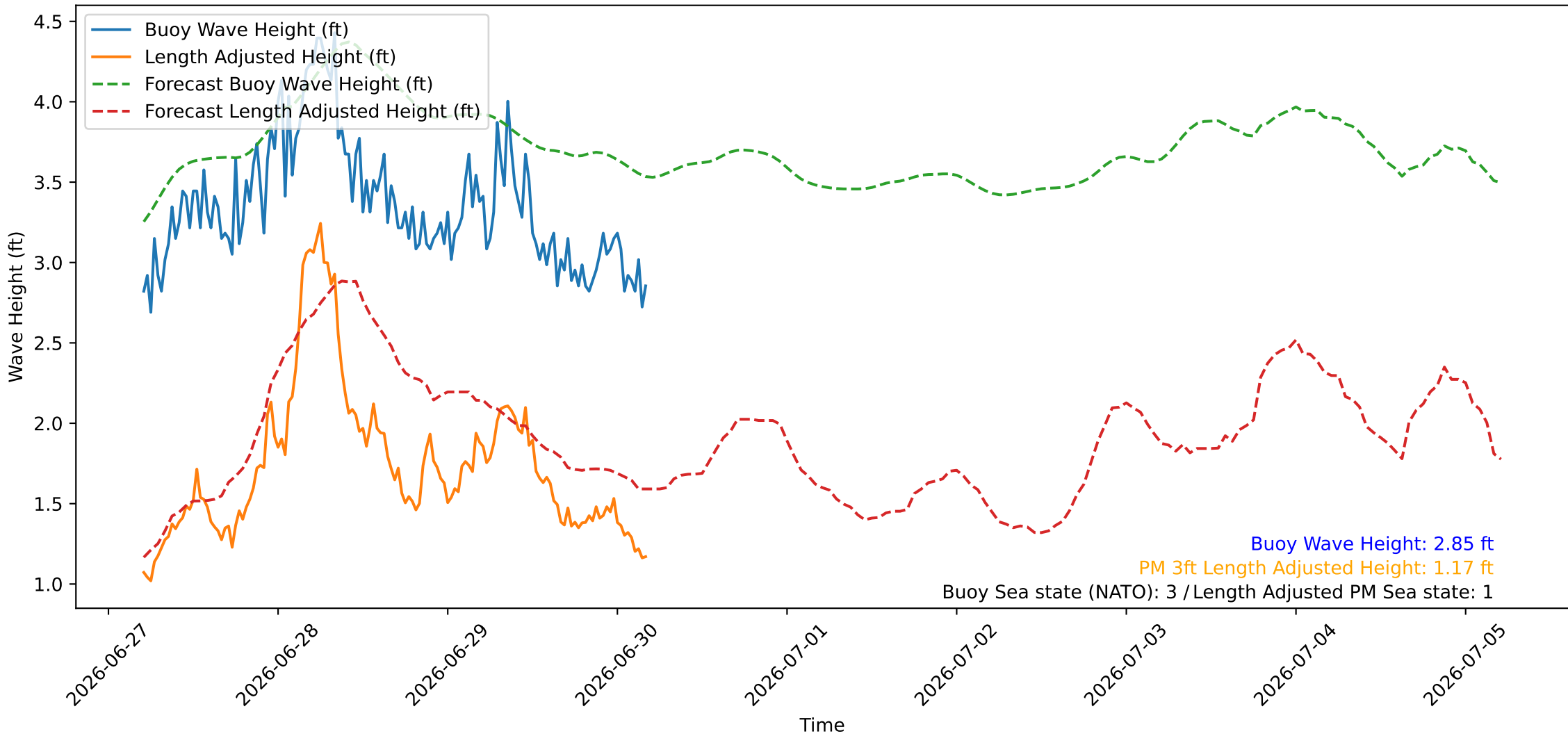
Wave Heights over Time for Oceanside Harbor at 2026-06-30 05:00:26
