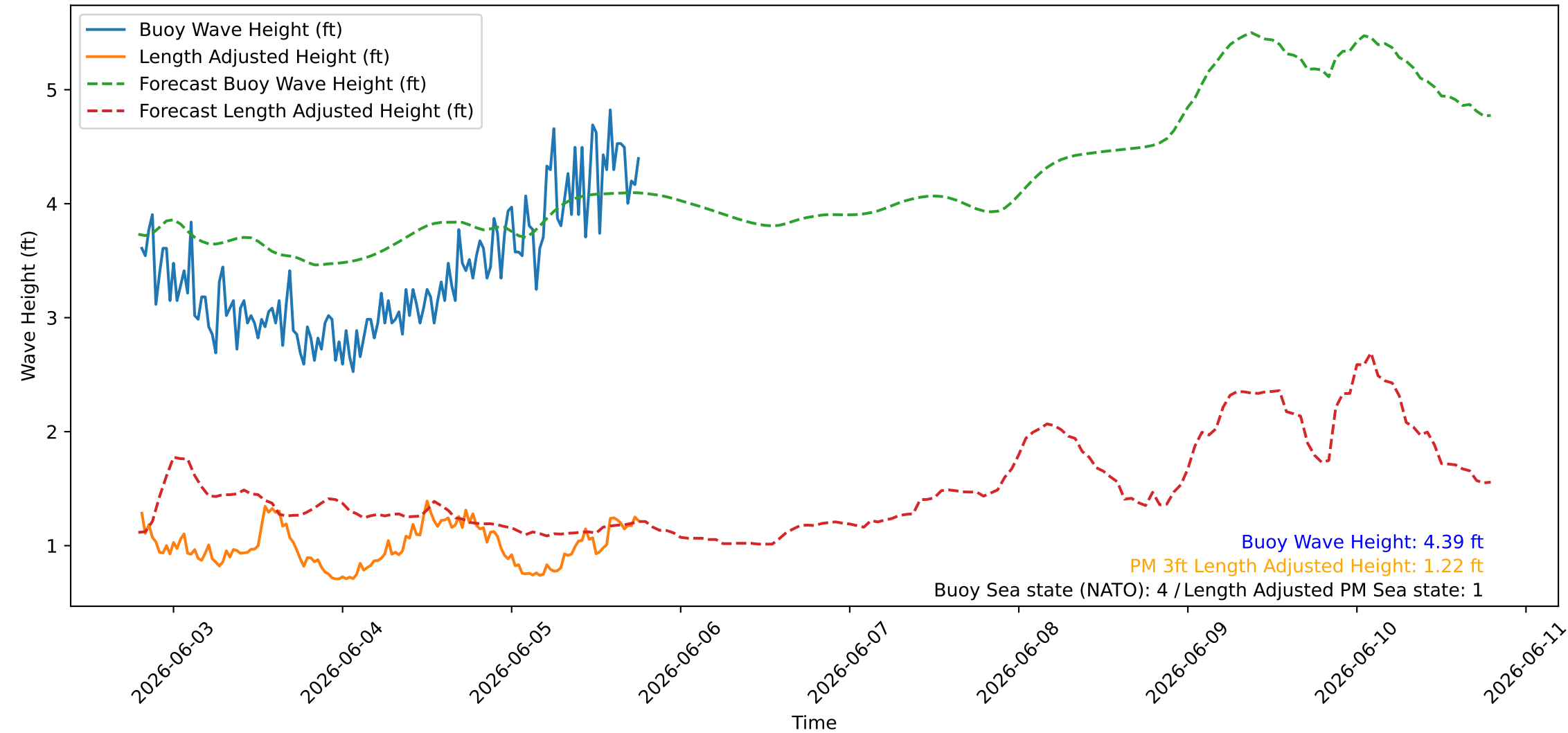
Wave Heights over Time for Red Beach at 2026-06-05 19:00:45
