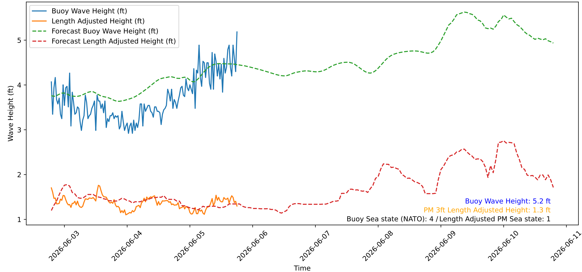
Wave Heights over Time for Oceanside Harbor at 2026-06-05 19:00:26
