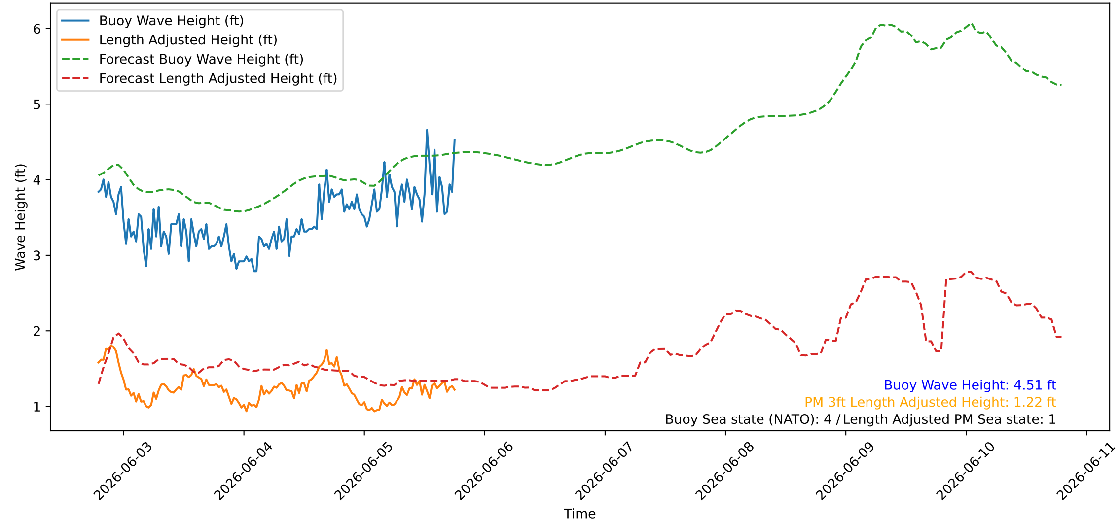
Wave Heights over Time for Green Beach at 2026-06-05 19:01:07
