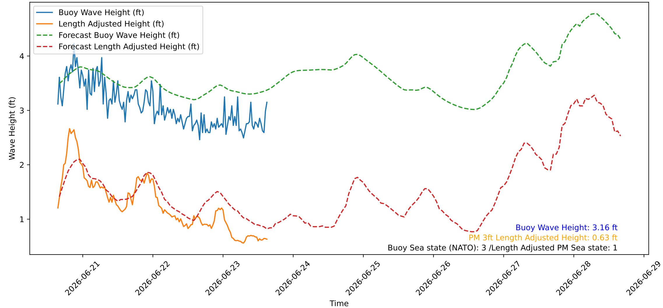
Wave Heights over Time for Green Beach at 2026-06-23 15:41:06
