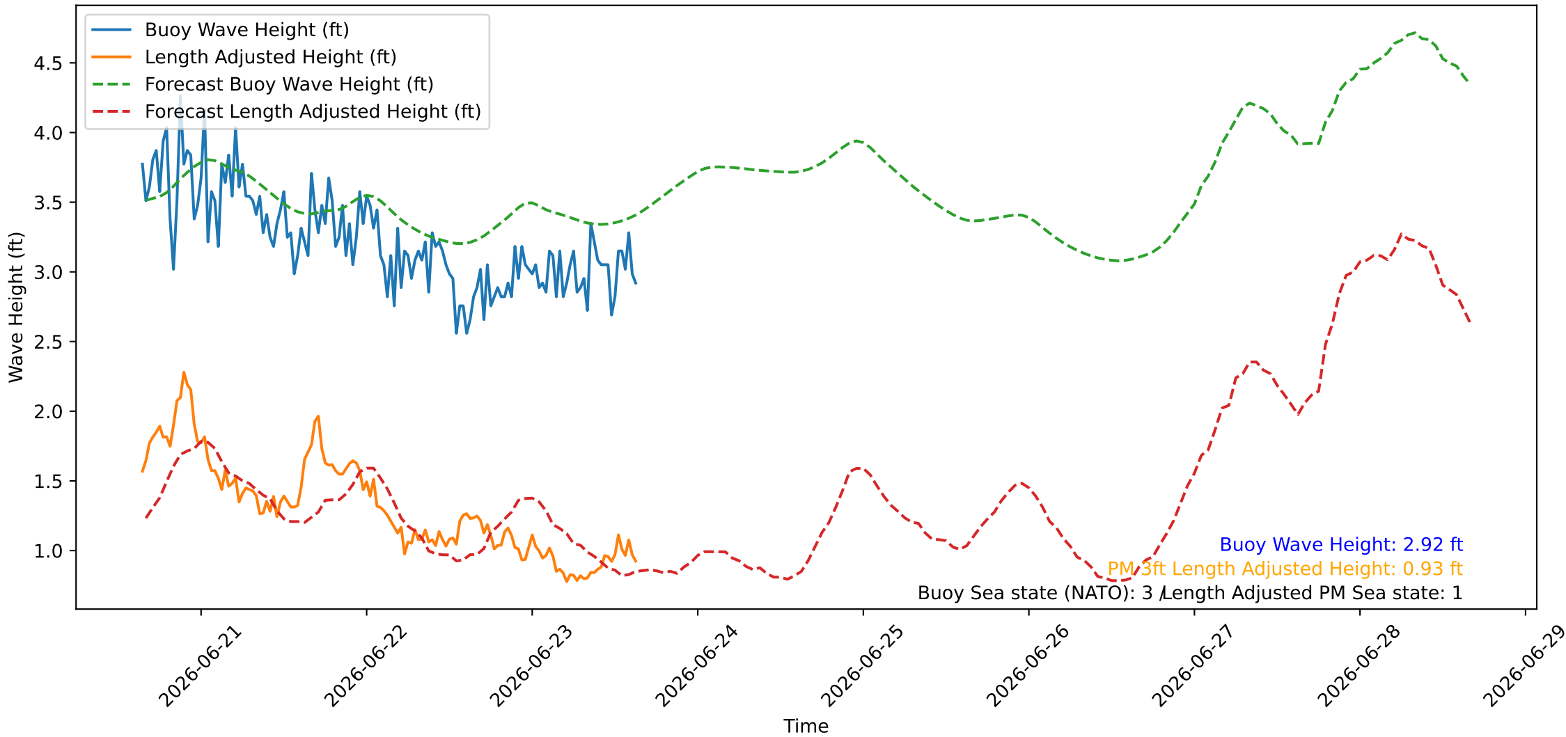
Wave Heights over Time for Oceanside Harbor at 2026-06-23 15:40:25
