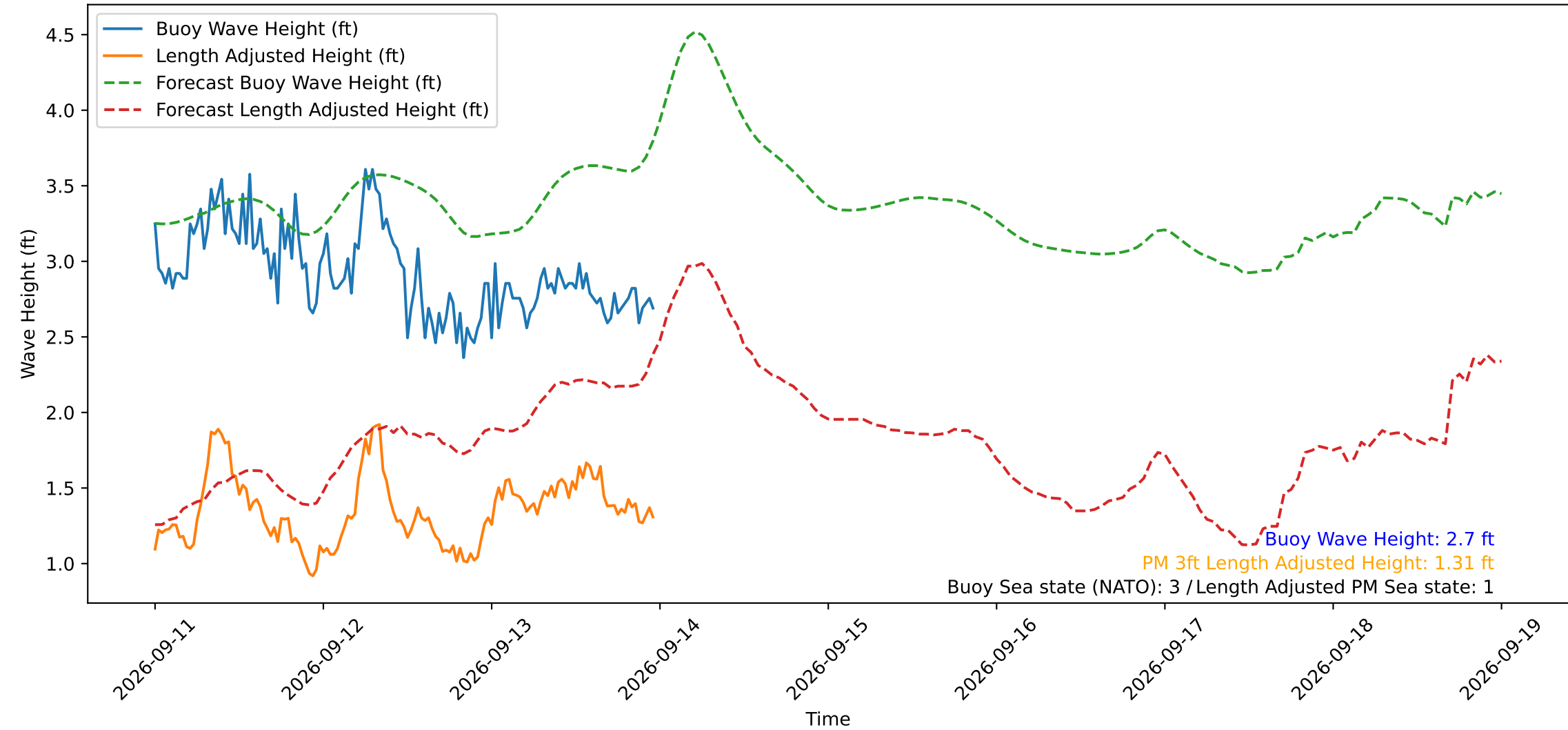
Wave Heights over Time for Green Beach at 2026-09-13 23:41:10
