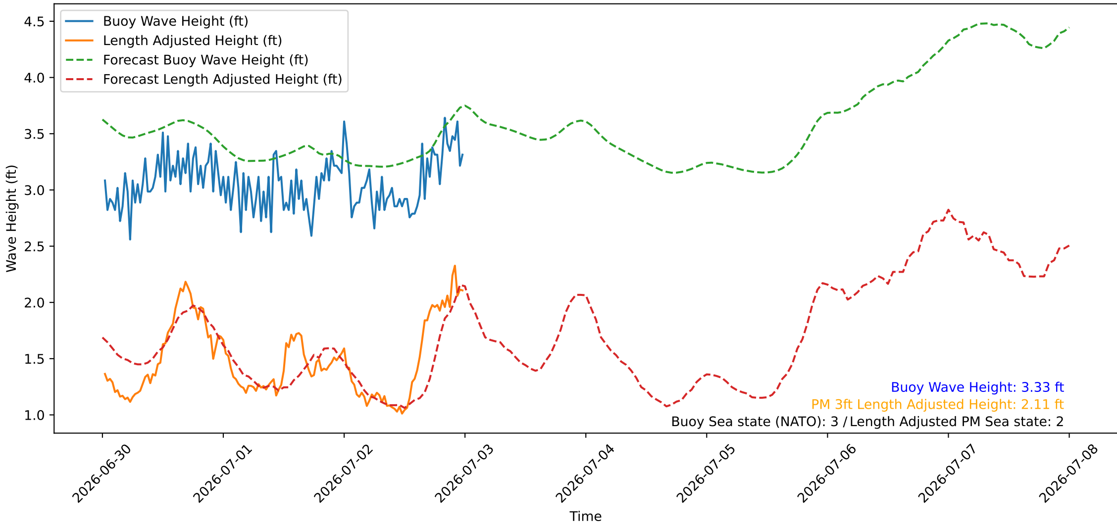
Wave Heights over Time for Oceanside Harbor at 2026-07-03 00:20:26
