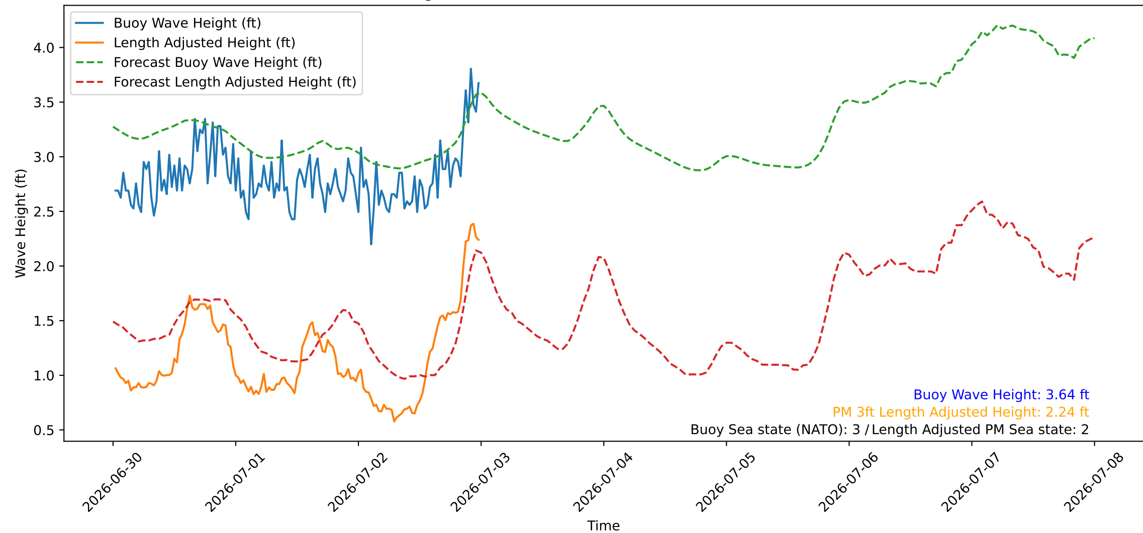
Wave Heights over Time for Red Beach at 2026-07-03 00:20:46
