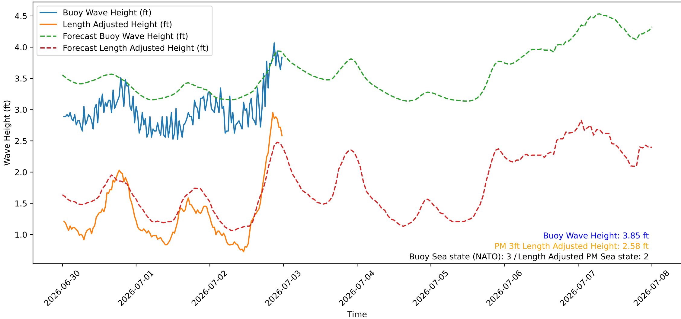
Wave Heights over Time for Green Beach at 2026-07-03 00:21:08
