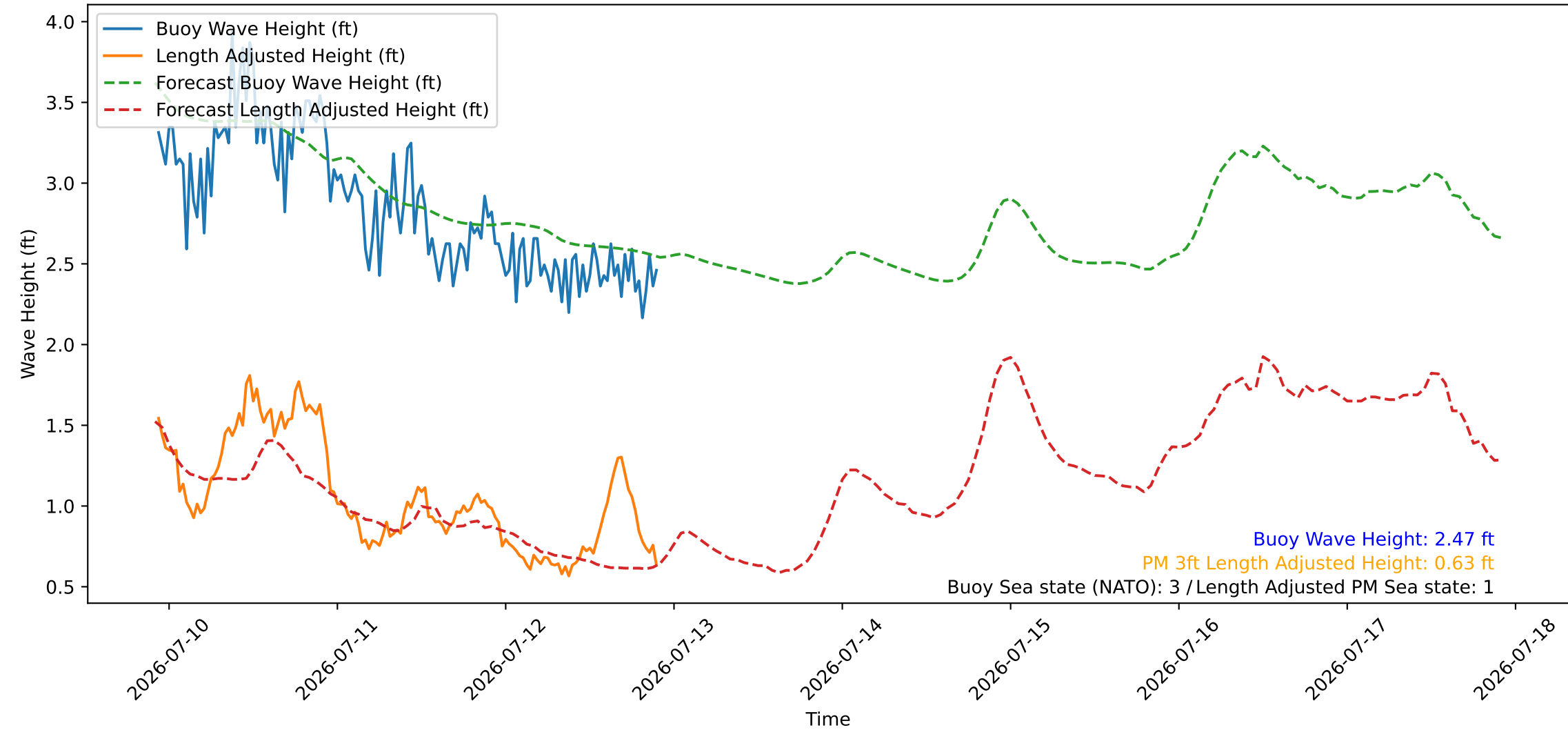
Wave Heights over Time for Red Beach at 2026-07-12 22:20:46
