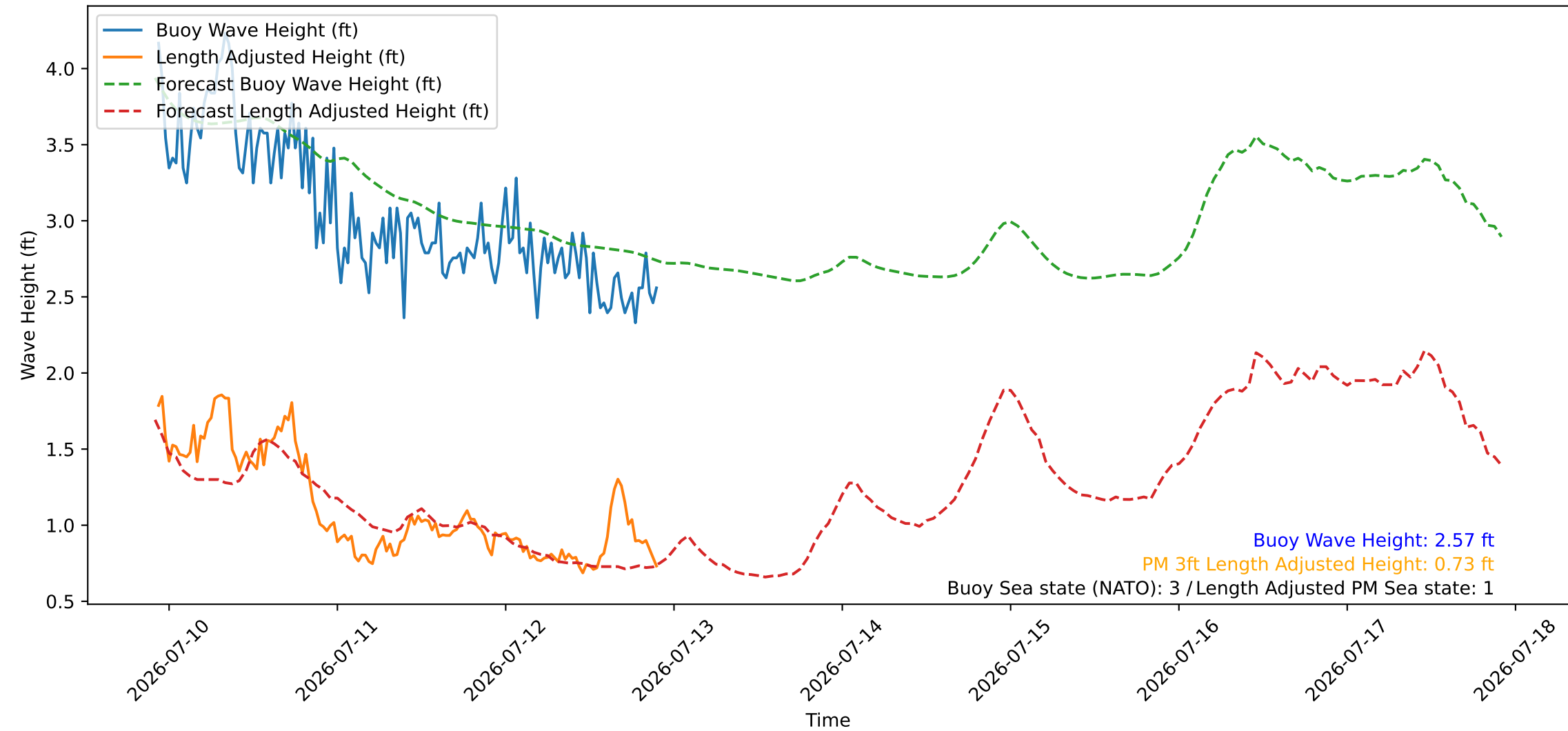
Wave Heights over Time for Oceanside Harbor at 2026-07-12 22:20:26
