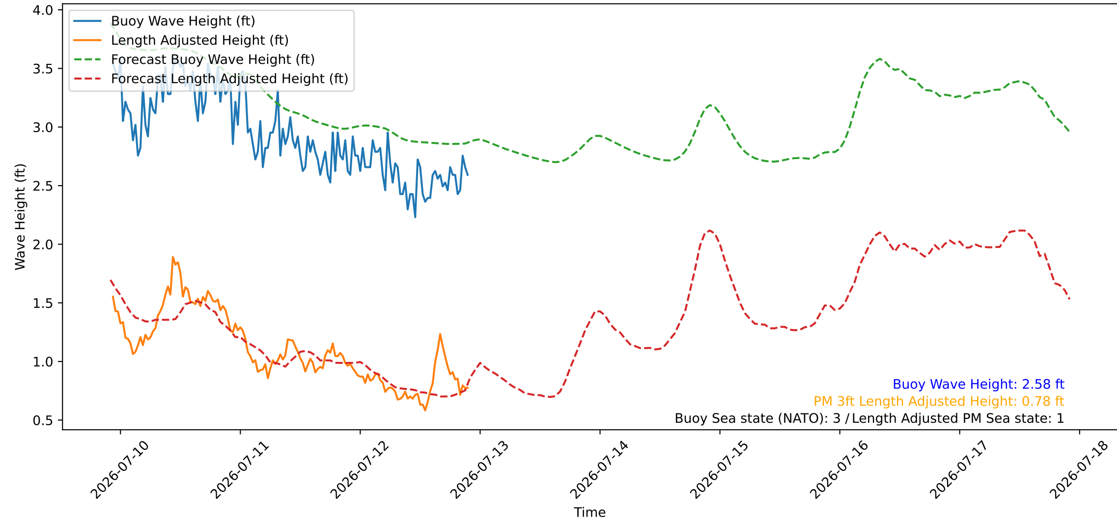
Wave Heights over Time for Green Beach at 2026-07-12 22:21:08
