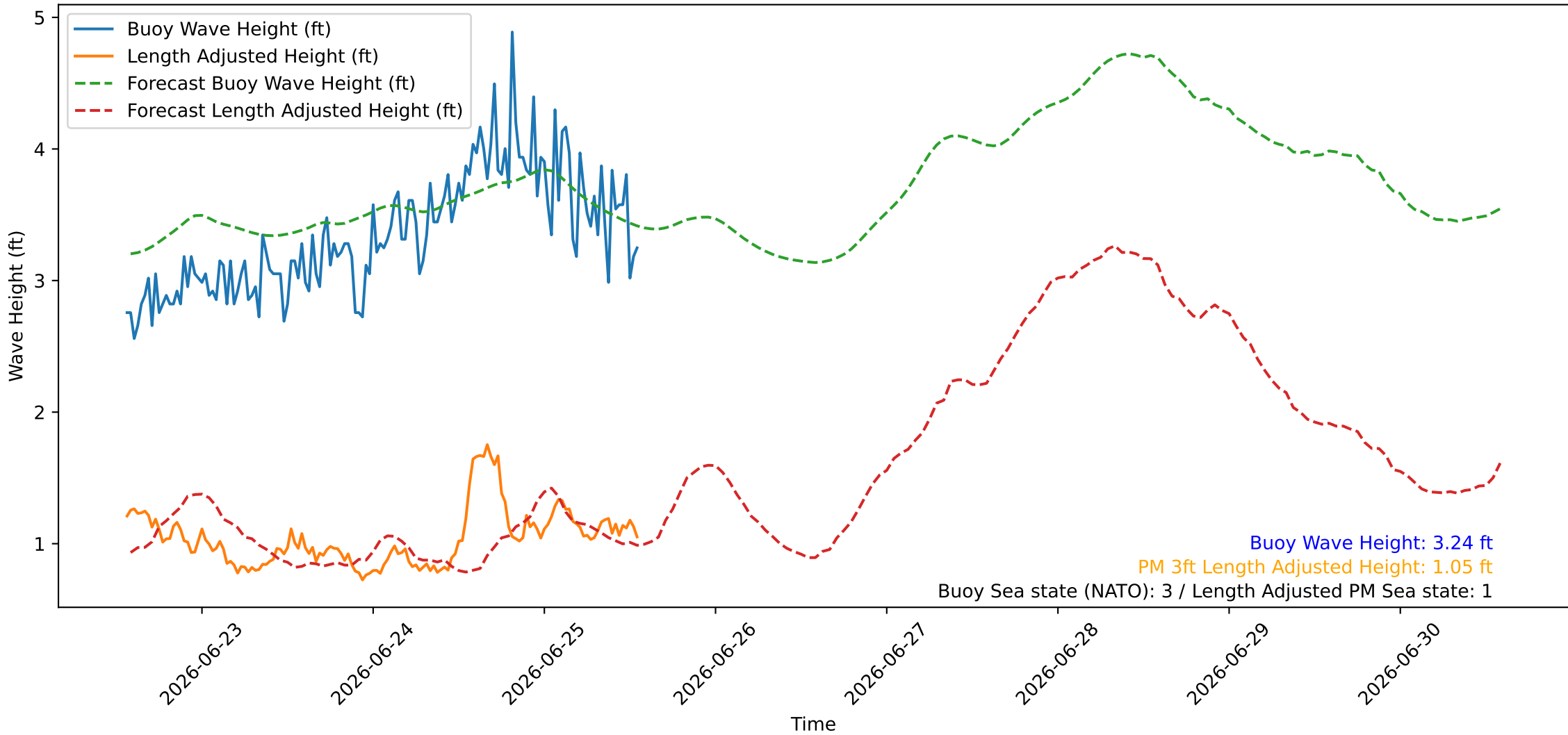
Wave Heights over Time for Oceanside Harbor at 2026-06-25 13:40:26
