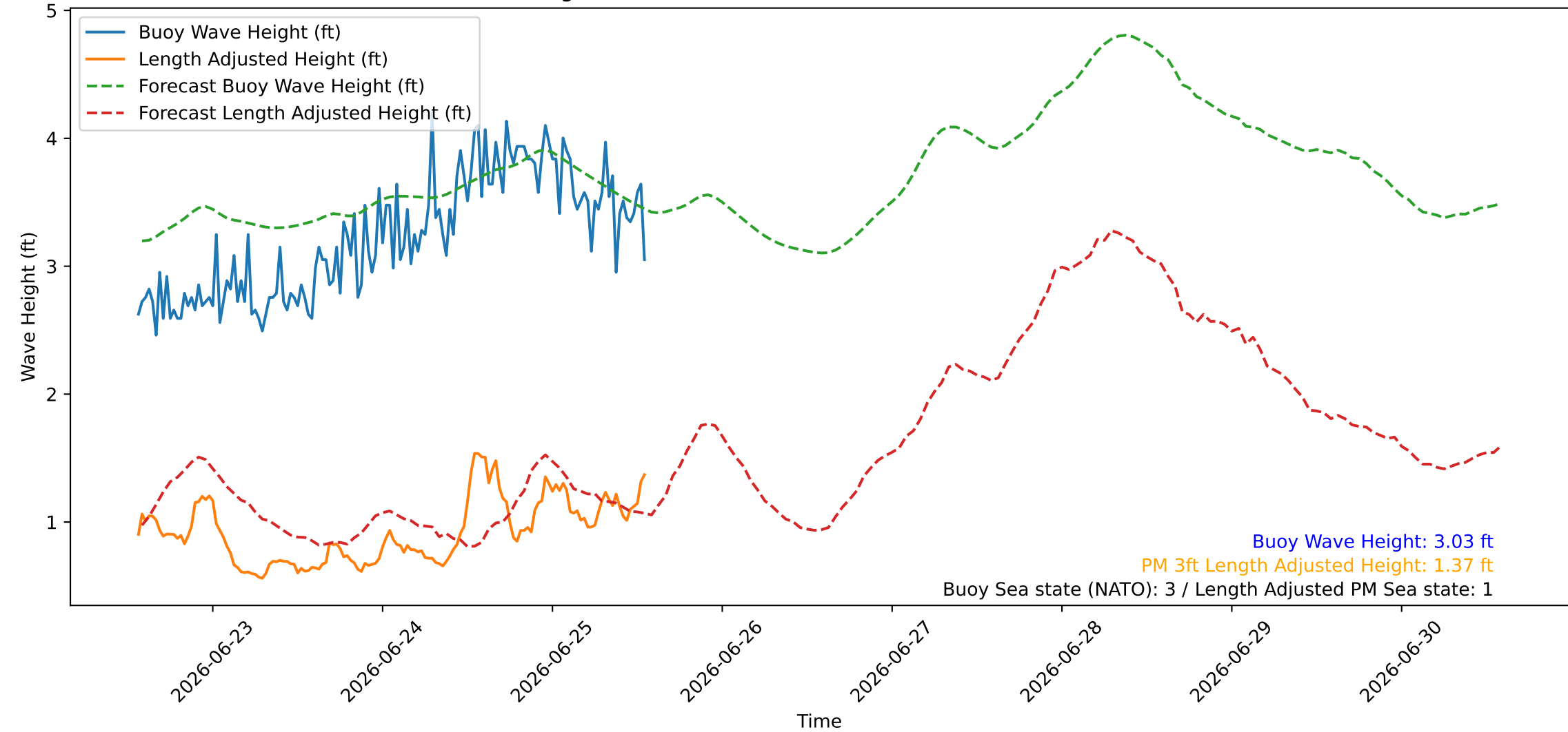
Wave Heights over Time for Green Beach at 2026-06-25 13:41:08
