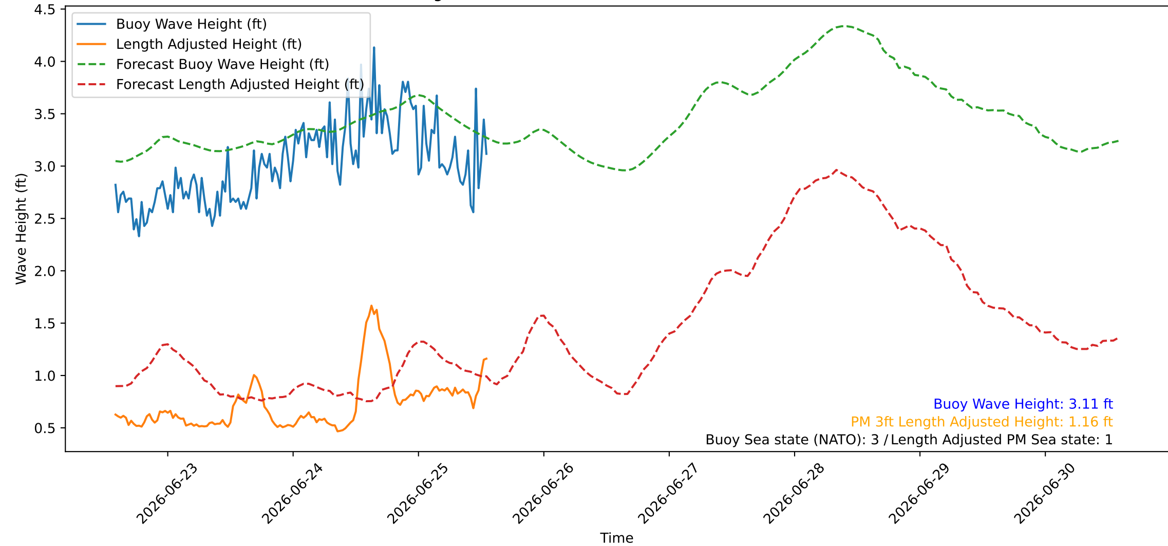
Wave Heights over Time for Red Beach at 2026-06-25 13:40:46
