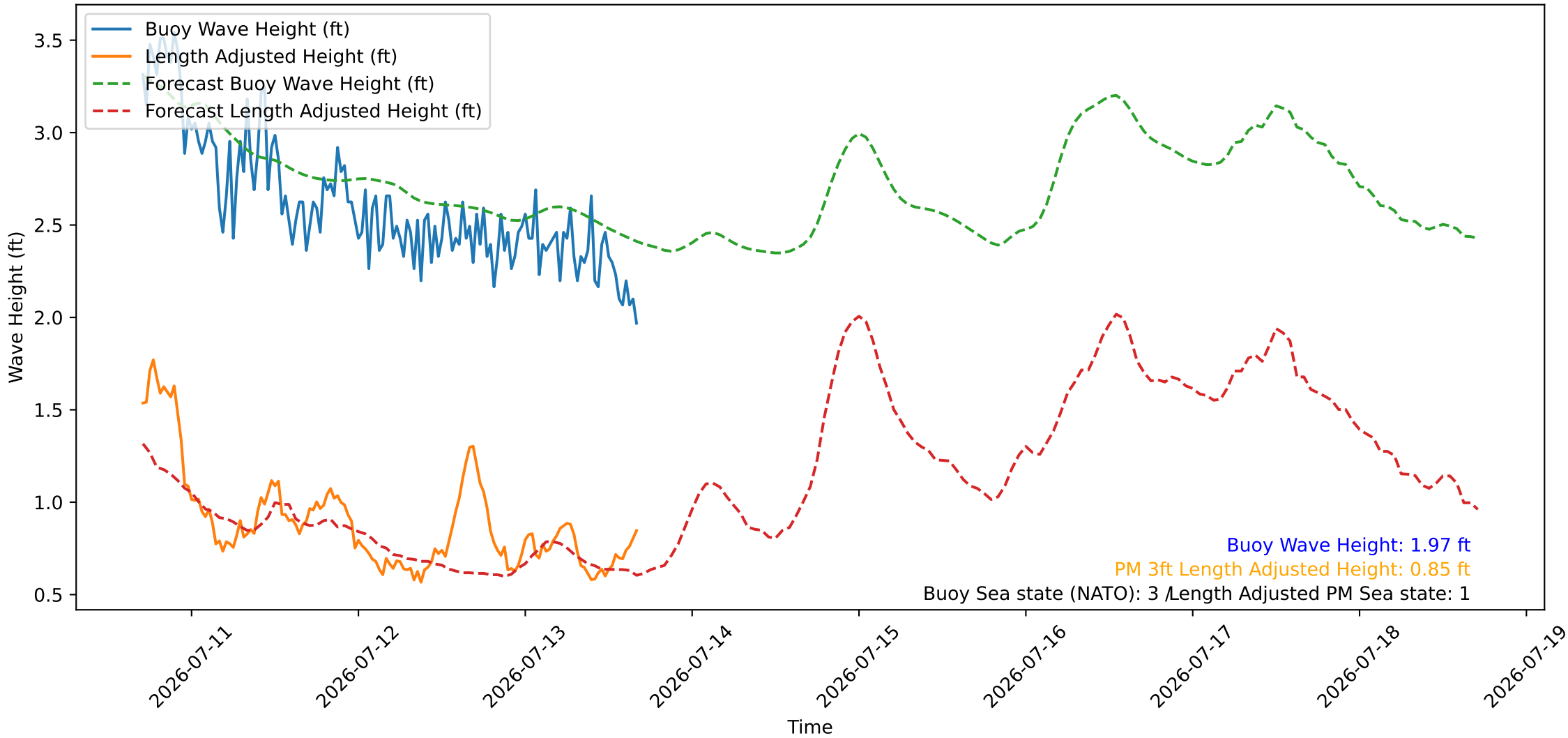
Wave Heights over Time for Red Beach at 2026-07-13 16:50:47
