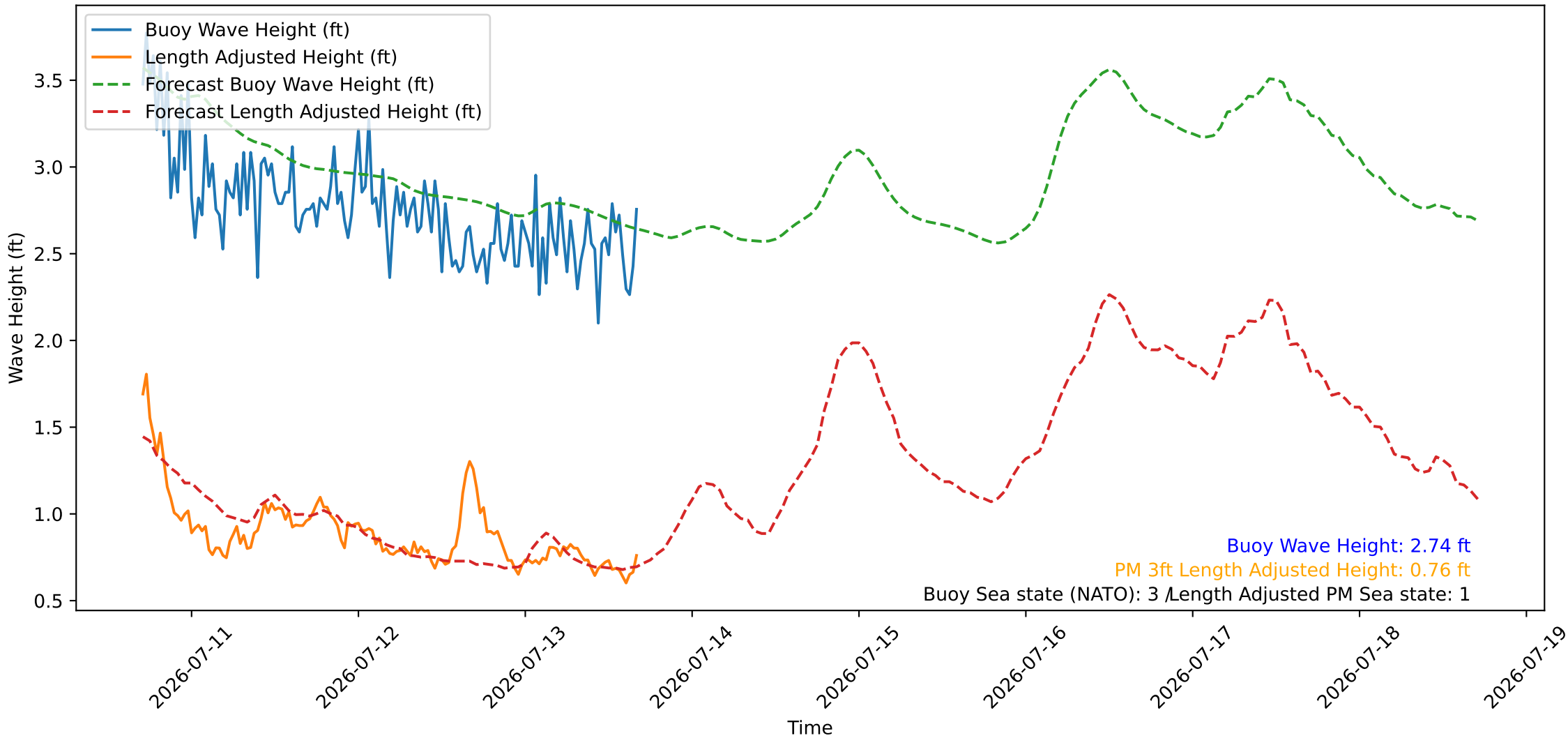
Wave Heights over Time for Oceanside Harbor at 2026-07-13 16:50:27
