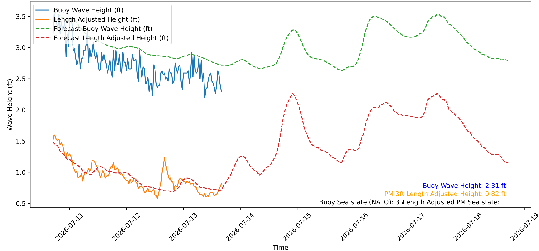
Wave Heights over Time for Green Beach at 2026-07-13 16:51:10
