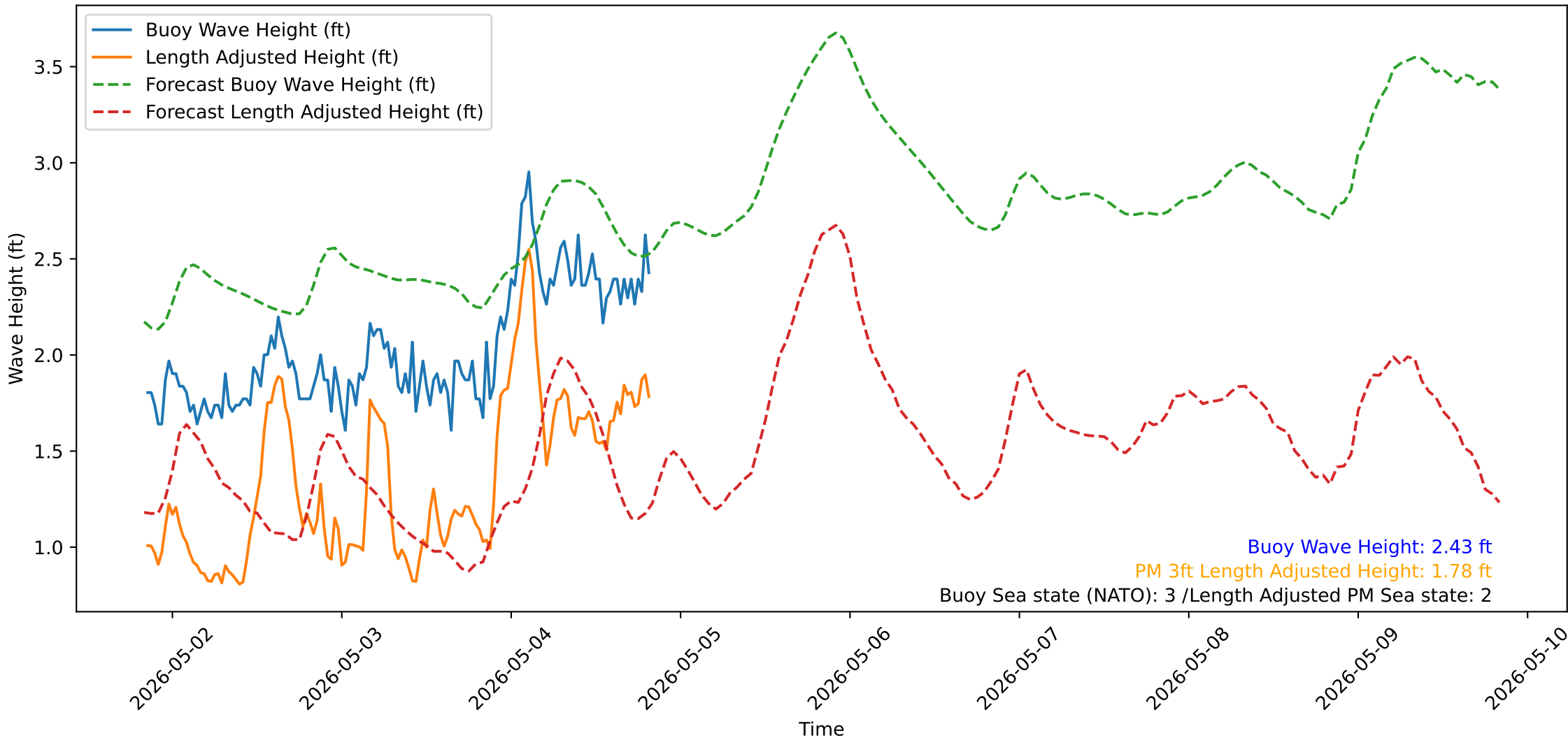
Wave Heights over Time for Red Beach at 2026-05-04 20:10:52
