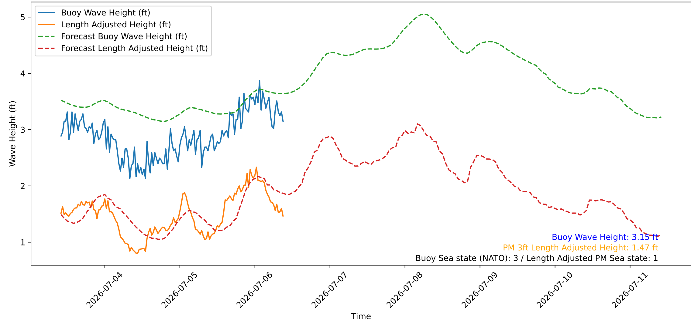
Wave Heights over Time for Oceanside Harbor at 2026-07-06 09:50:26
