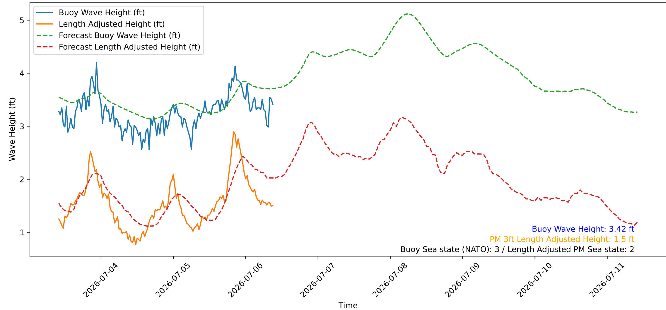
Wave Heights over Time for Green Beach at 2026-07-06 09:51:10
