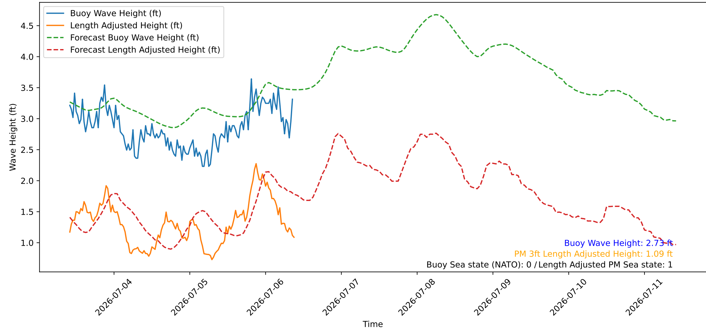
Wave Heights over Time for Red Beach at 2026-07-06 09:50:47
