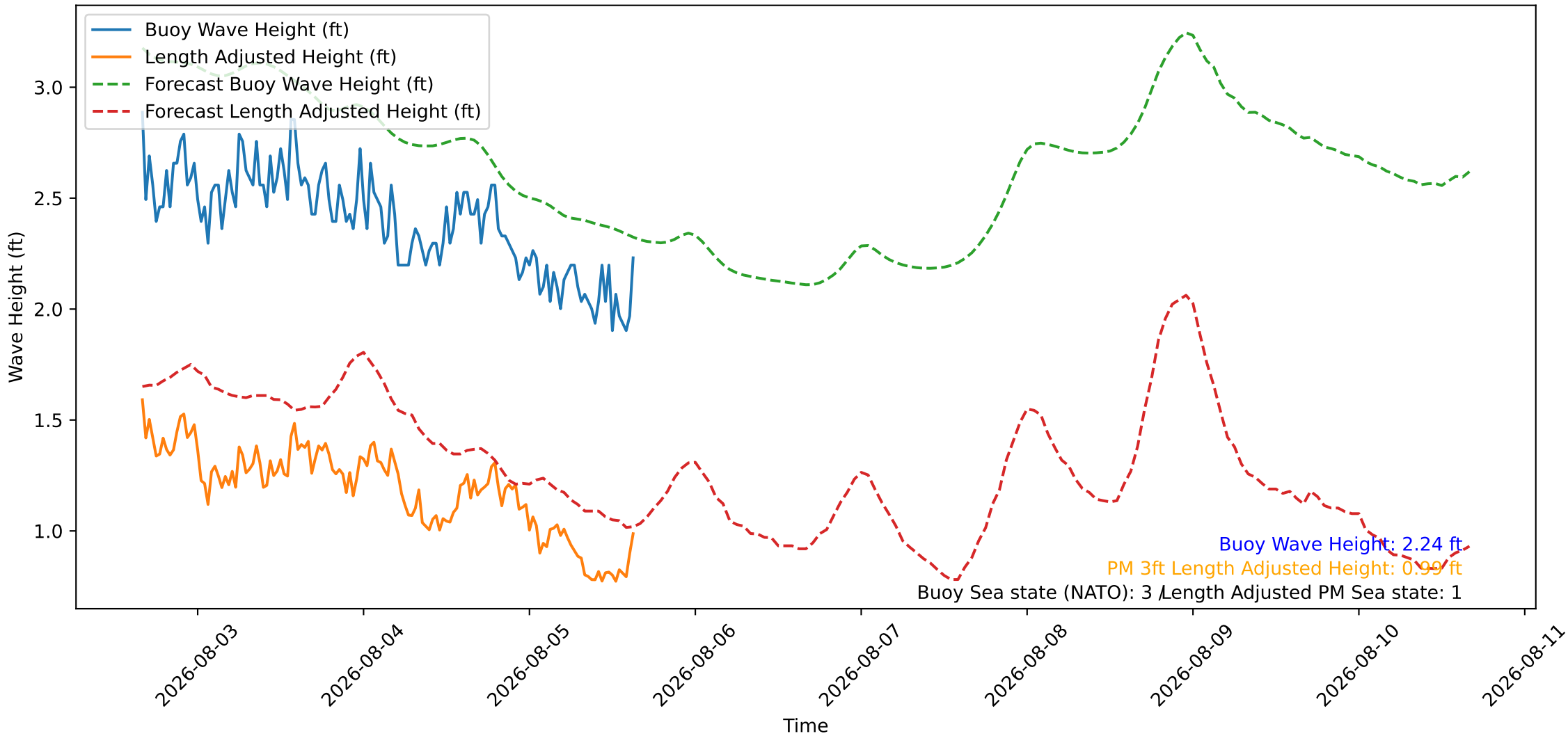
Wave Heights over Time for Oceanside Harbor at 2026-08-05 16:00:26
