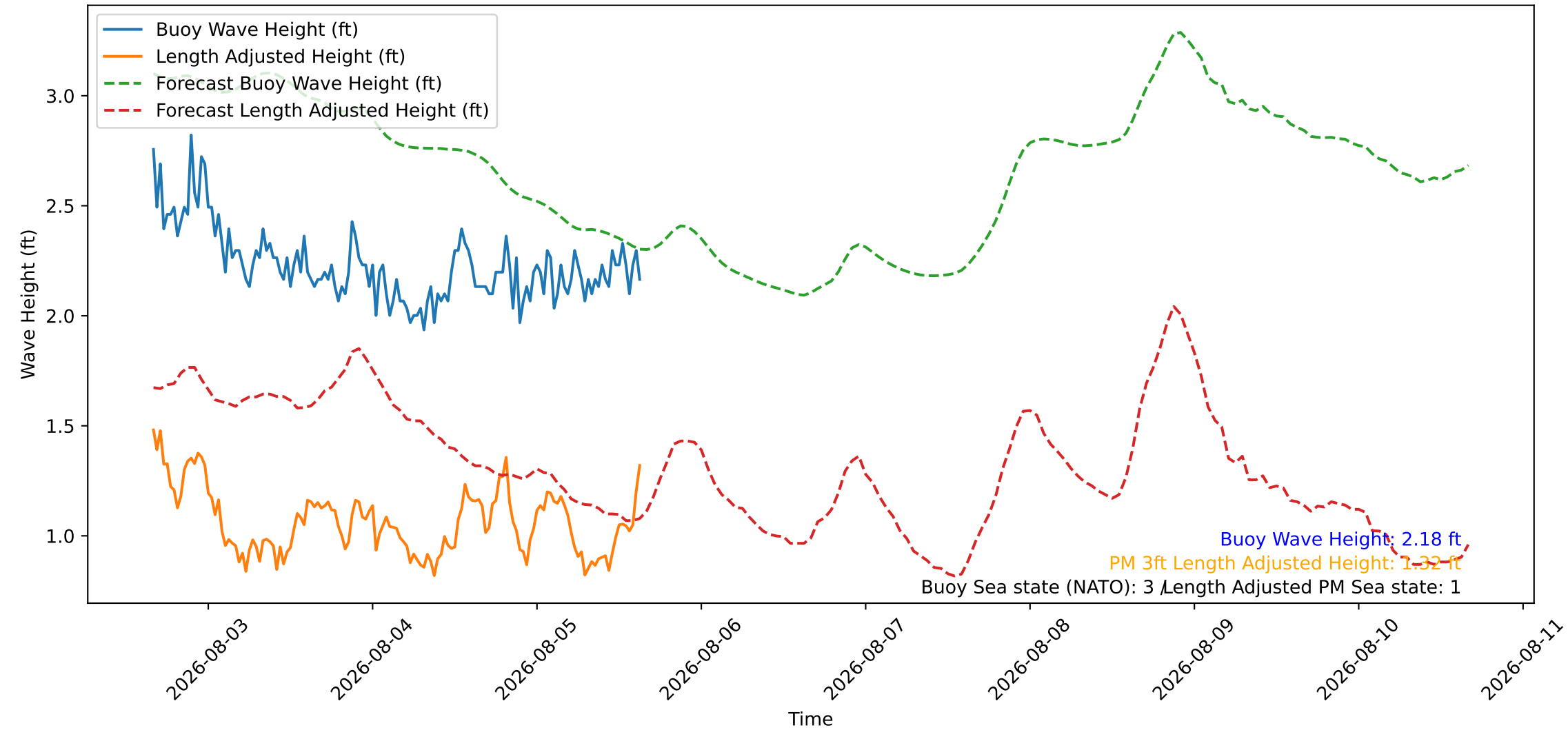
Wave Heights over Time for Green Beach at 2026-08-05 16:01:08
