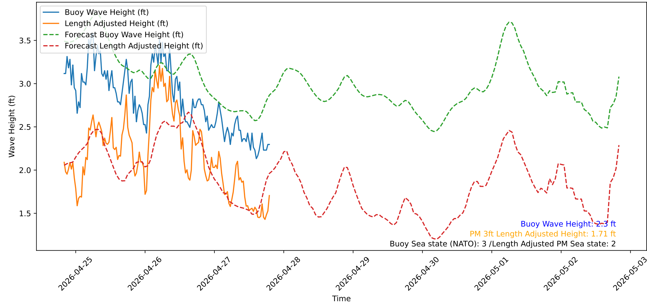
Wave Heights over Time for Green Beach at 2026-04-27 19:51:13
