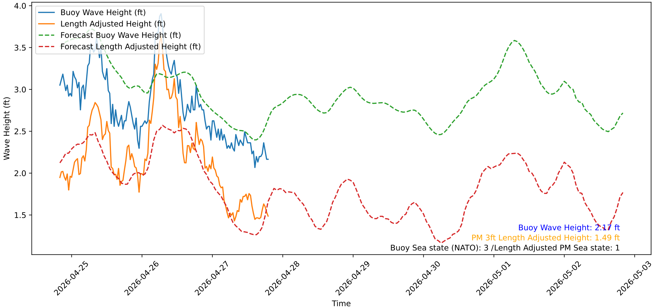
Wave Heights over Time for Oceanside Harbor at 2026-04-27 19:50:31
