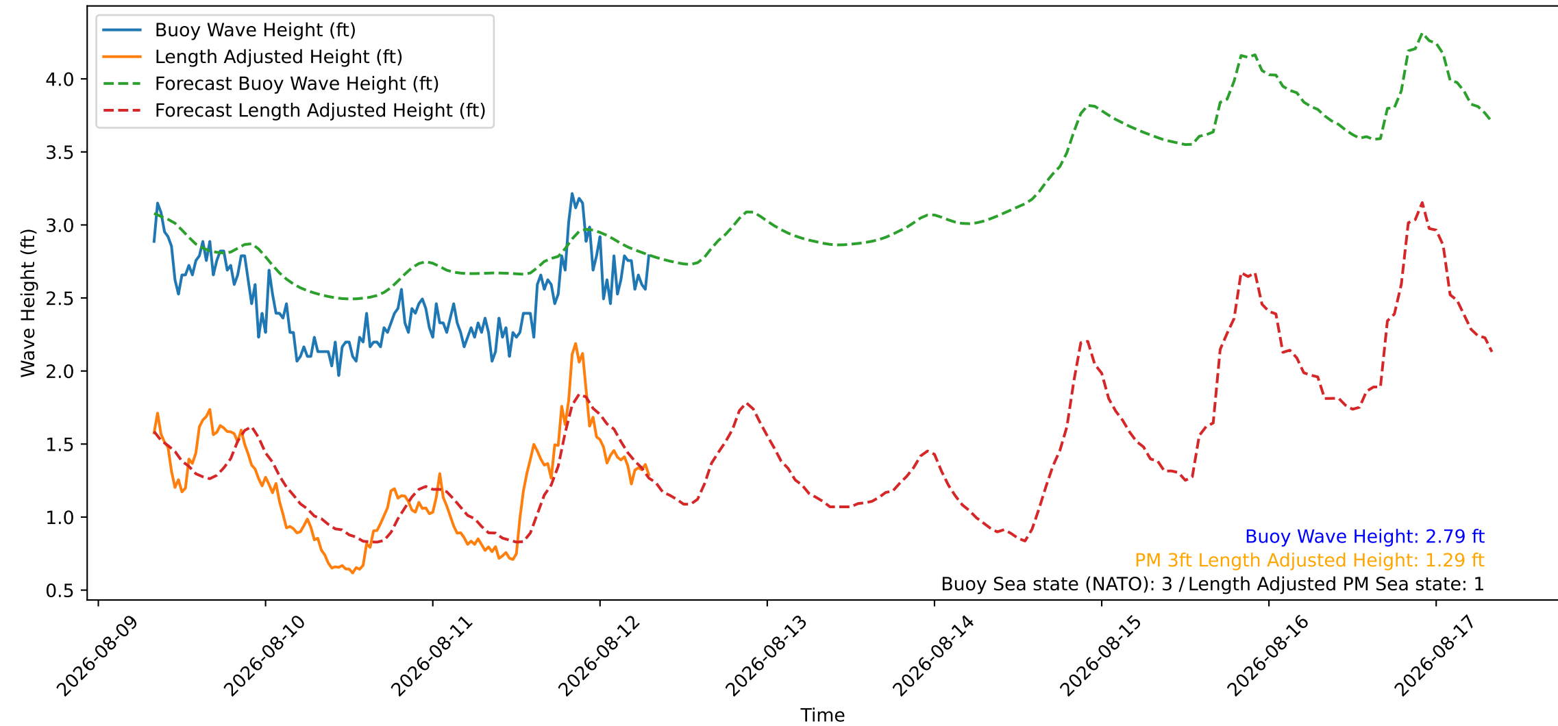
Wave Heights over Time for Green Beach at 2026-08-12 08:01:09
