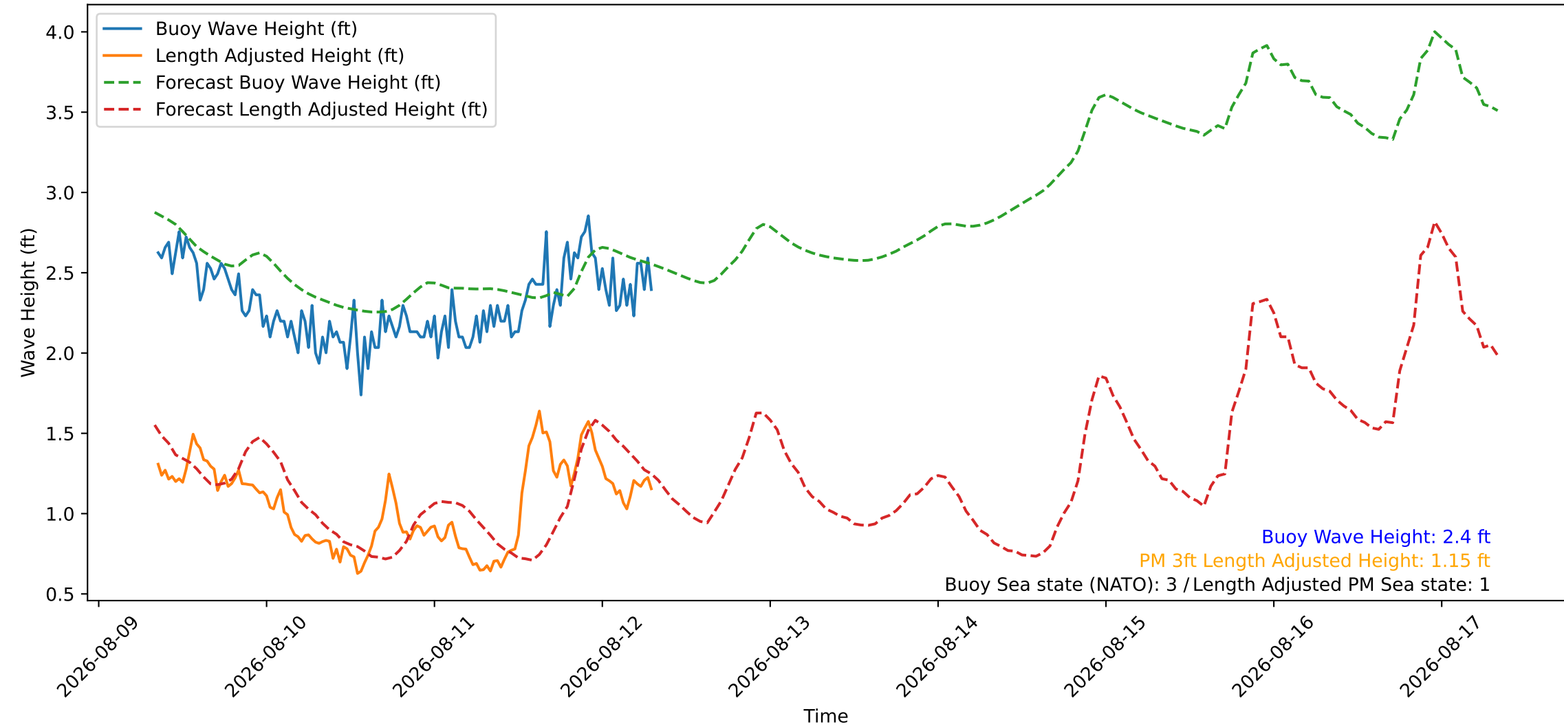
Wave Heights over Time for Red Beach at 2026-08-12 08:00:46
