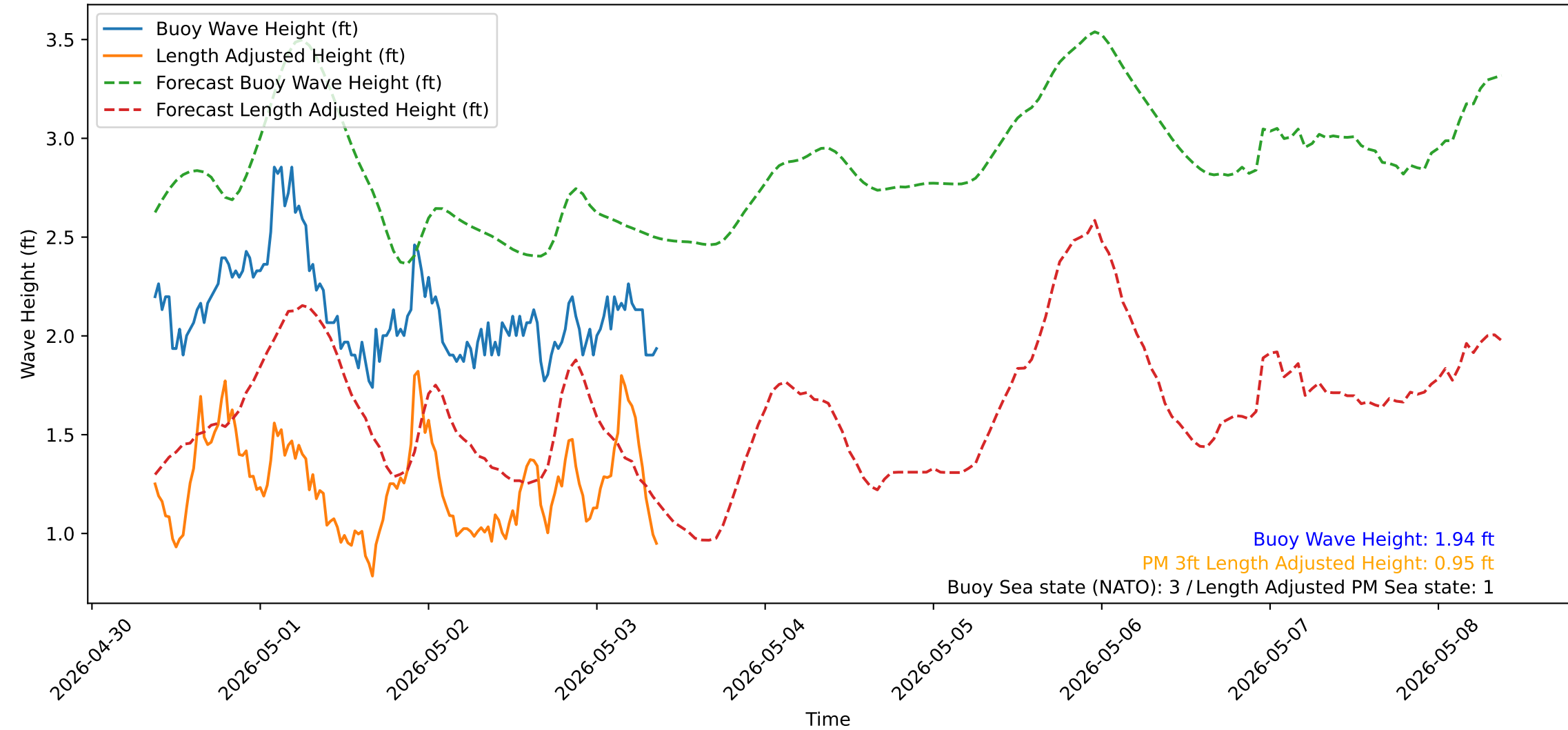
Wave Heights over Time for Green Beach at 2026-05-03 09:11:12
