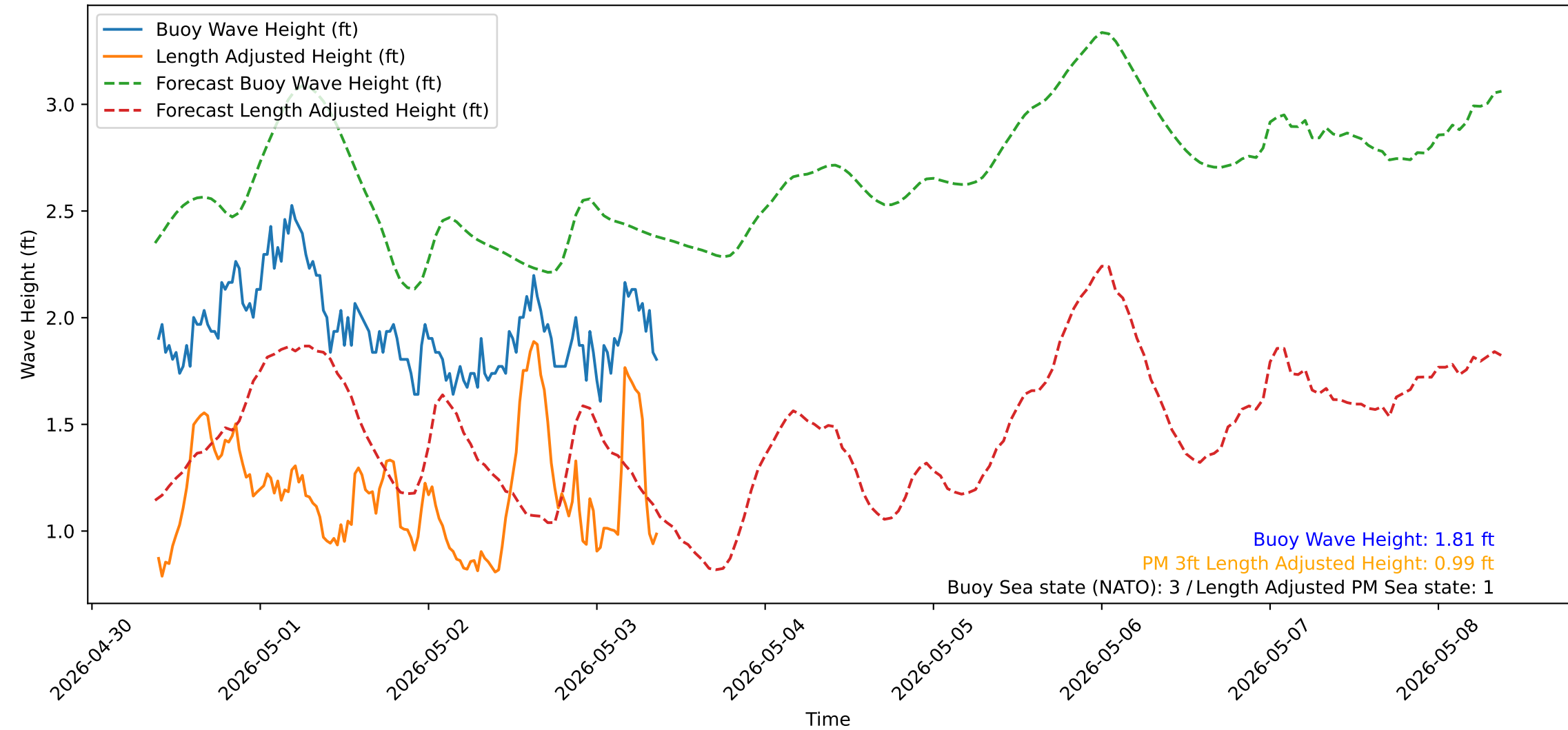
Wave Heights over Time for Red Beach at 2026-05-03 09:10:50
