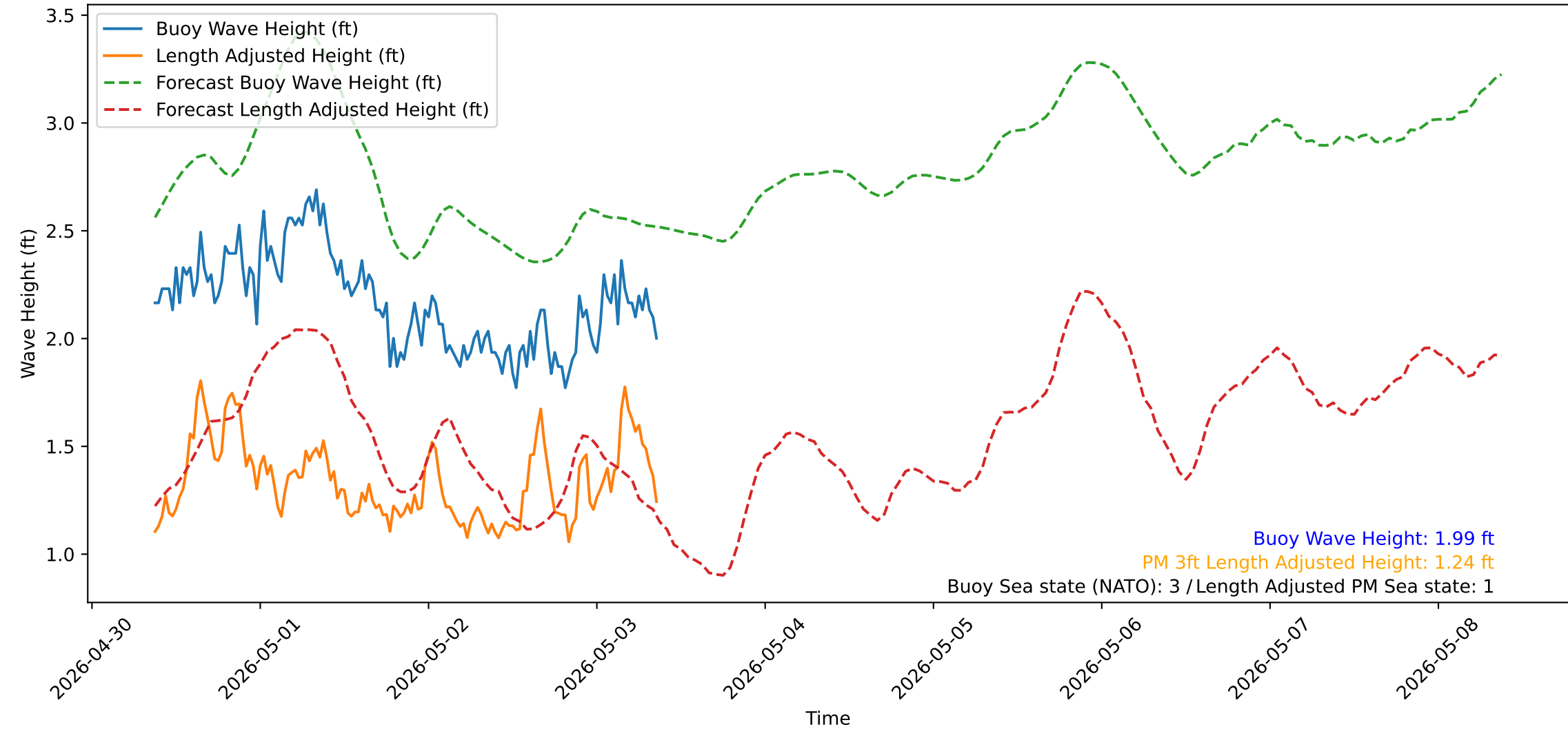
Wave Heights over Time for Oceanside Harbor at 2026-05-03 09:10:31
