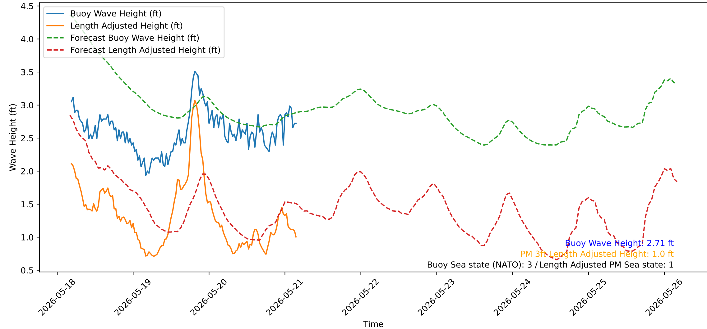
Wave Heights over Time for Red Beach at 2026-05-21 04:20:52
