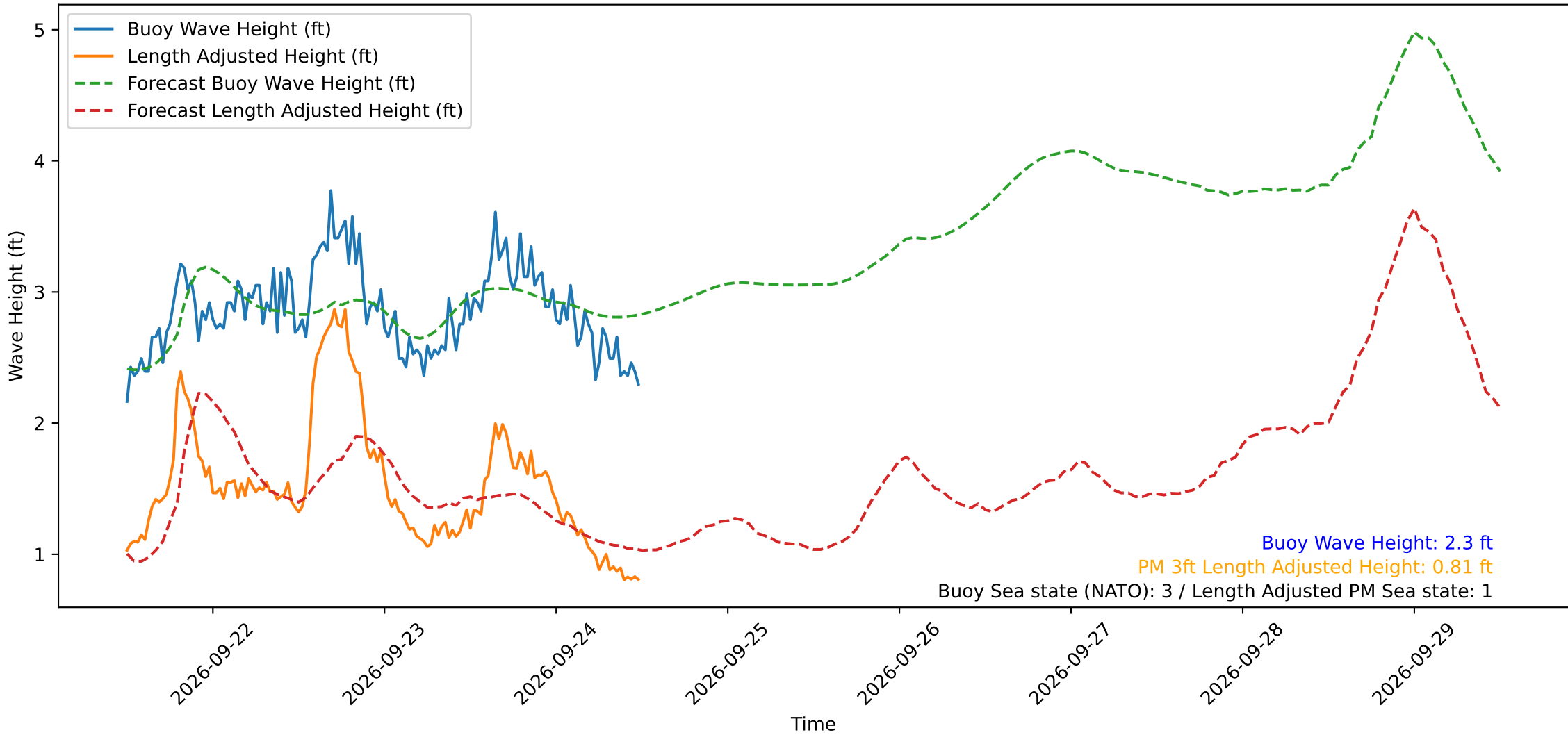
Wave Heights over Time for Oceanside Harbor at 2026-09-24 12:10:30
