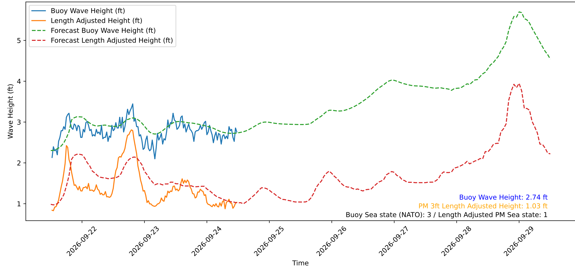
Wave Heights over Time for Green Beach at 2026-09-24 12:11:11
