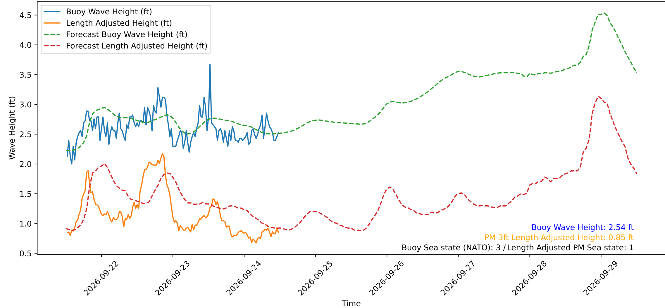
Wave Heights over Time for Red Beach at 2026-09-24 12:10:49
