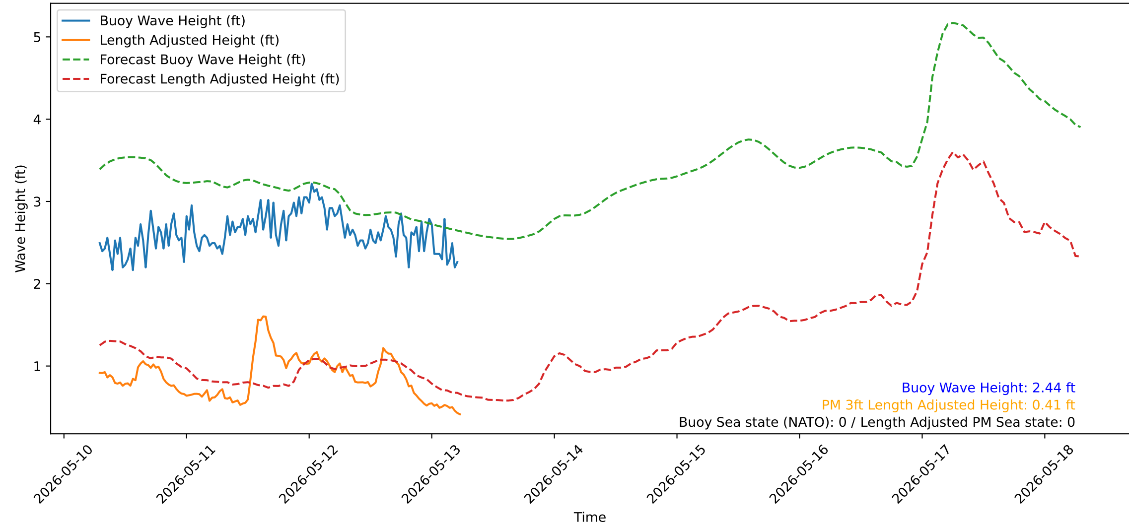
Wave Heights over Time for Red Beach at 2026-05-13 06:30:50
