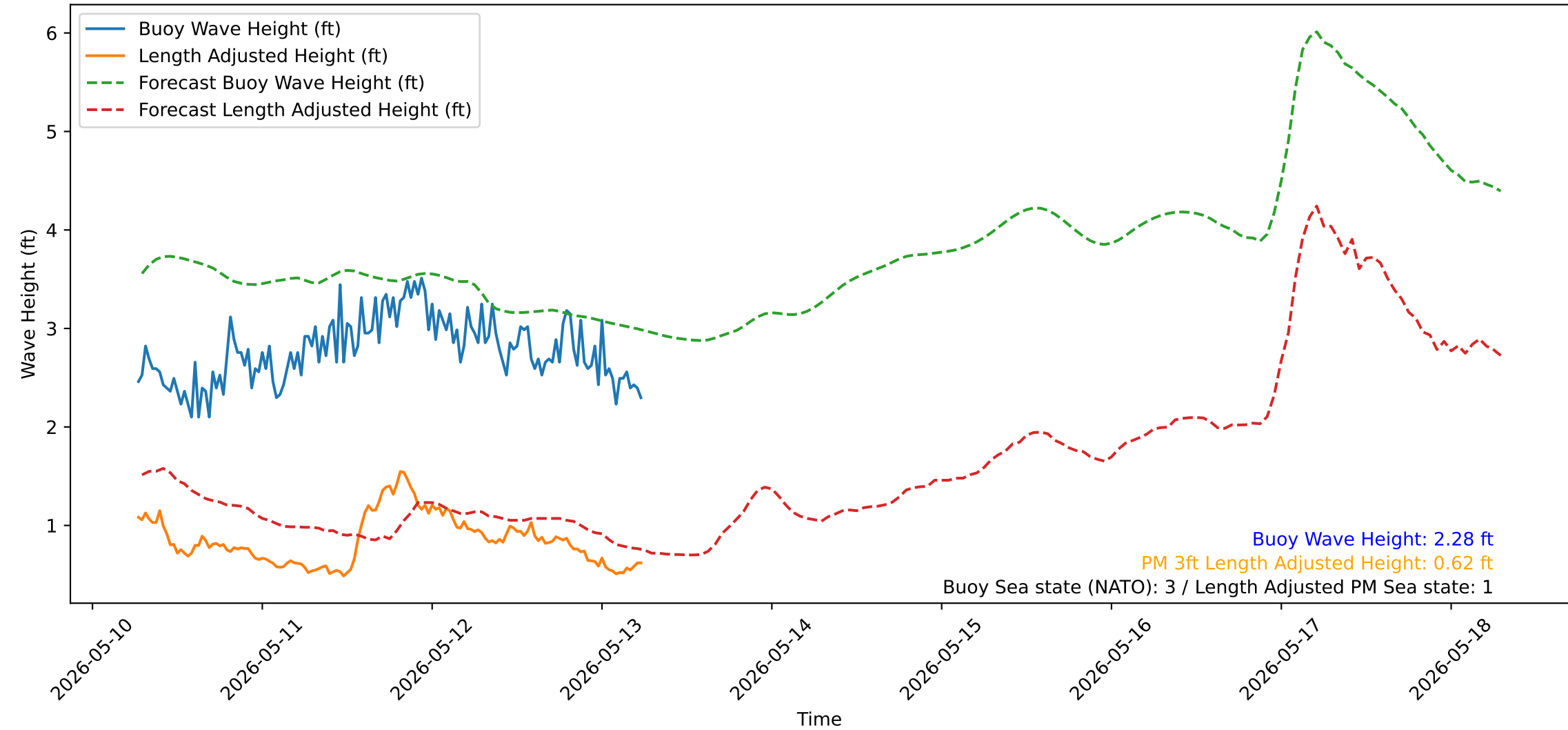
Wave Heights over Time for Green Beach at 2026-05-13 06:31:12
