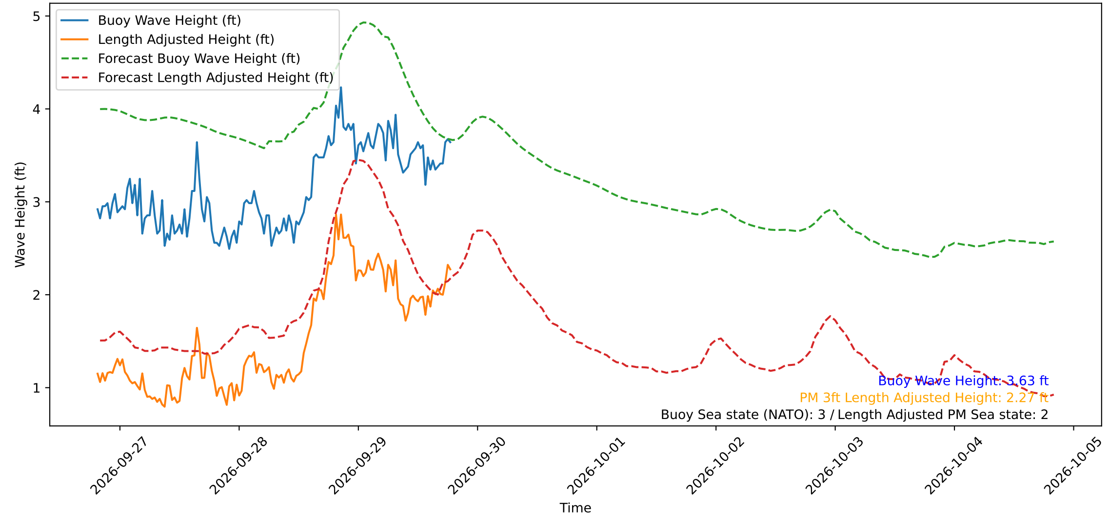
Wave Heights over Time for Oceanside Harbor at 2026-09-29 19:30:30
