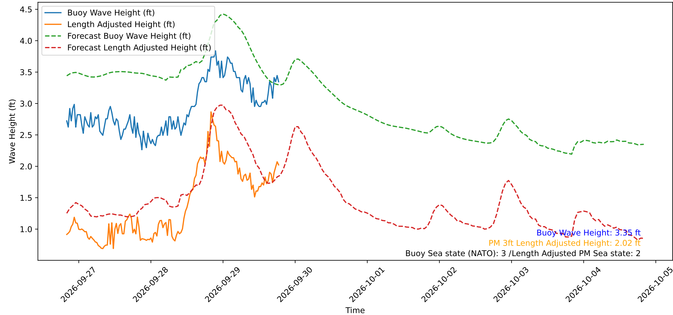
Wave Heights over Time for Red Beach at 2026-09-29 19:30:50
