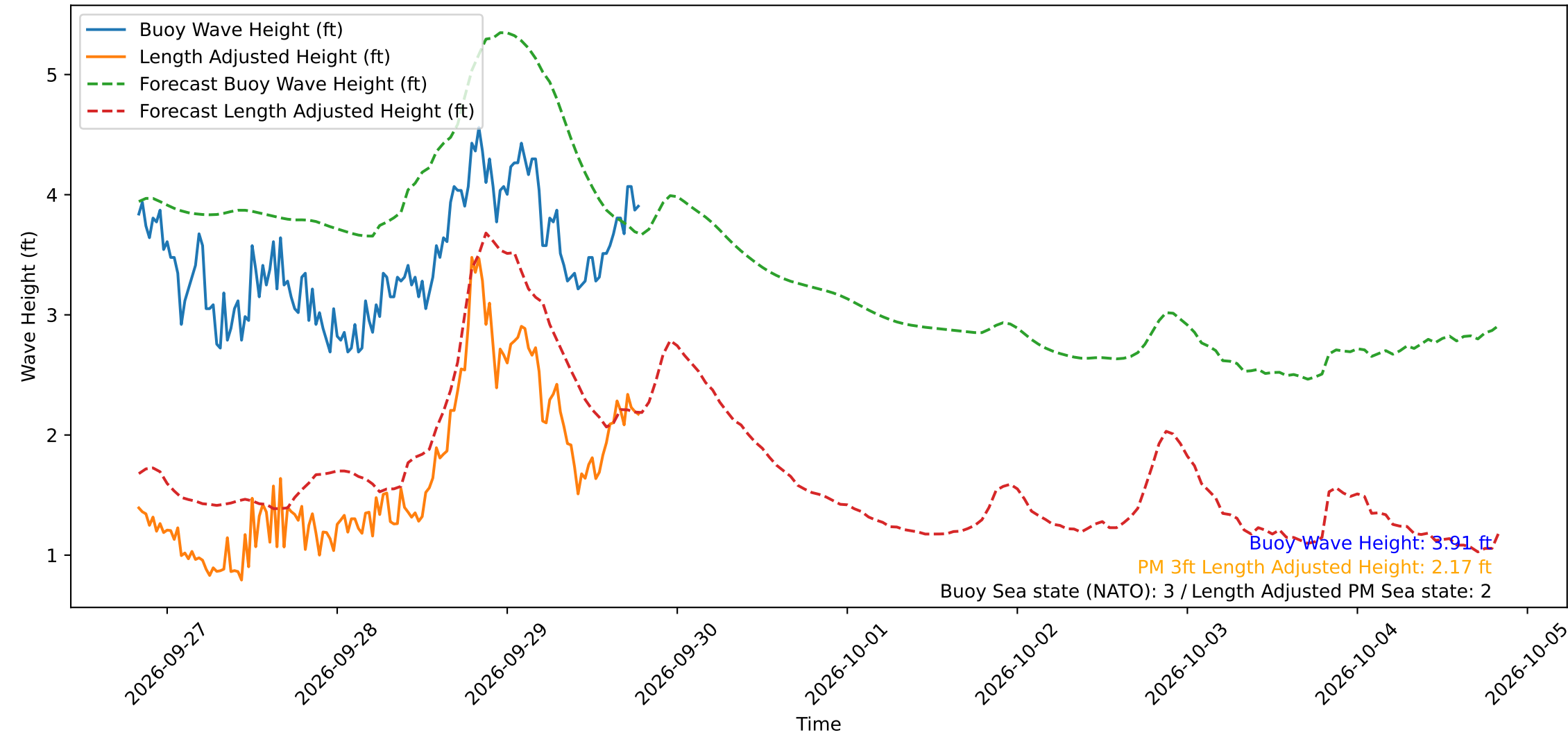
Wave Heights over Time for Green Beach at 2026-09-29 19:31:13
