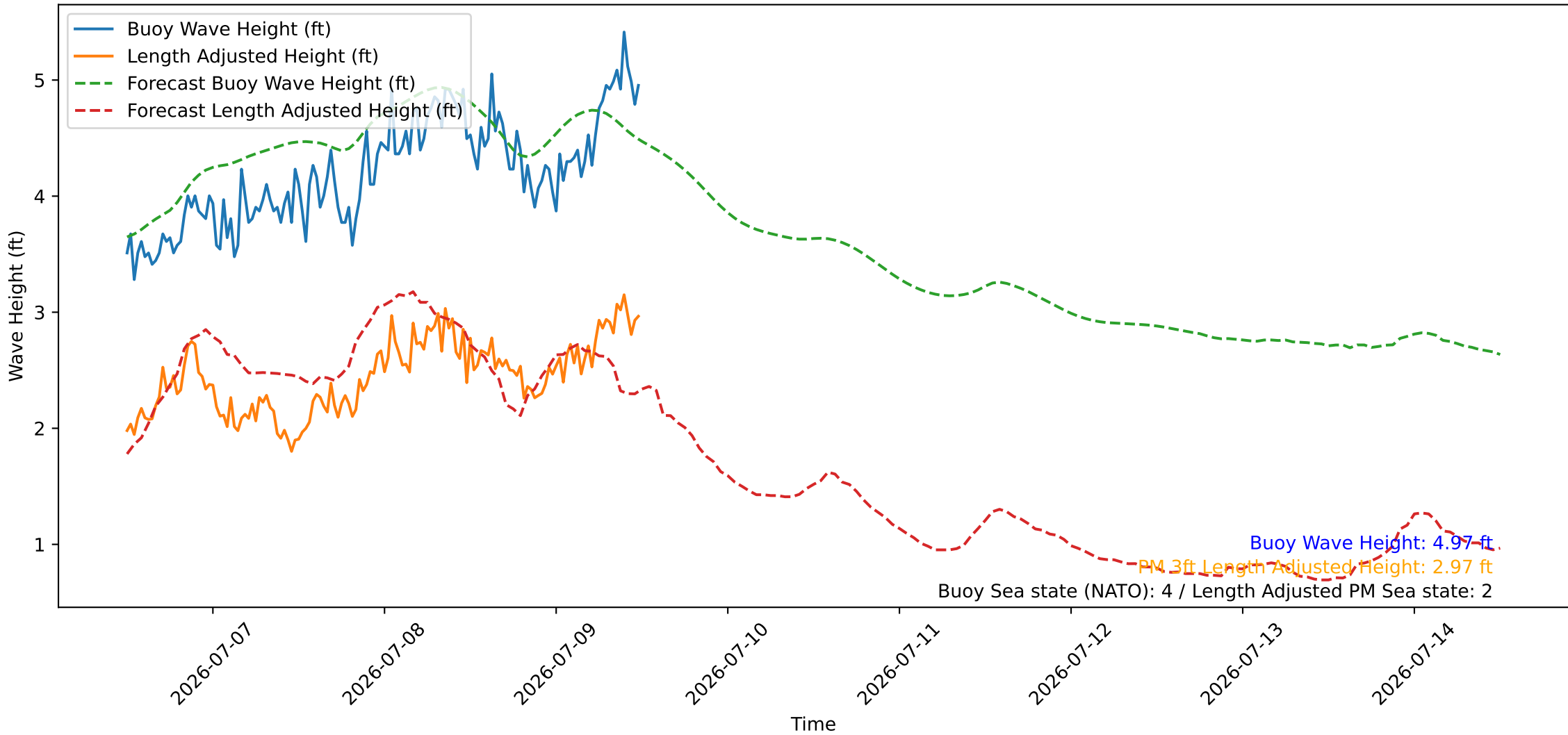
Wave Heights over Time for Oceanside Harbor at 2026-07-09 12:10:26
