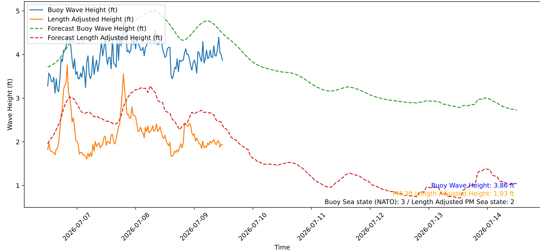
Wave Heights over Time for Green Beach at 2026-07-09 12:11:07
