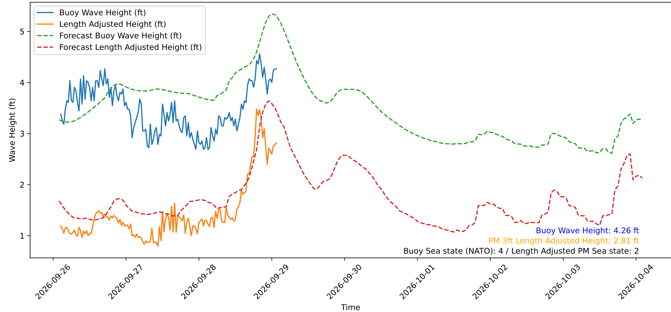
Wave Heights over Time for Green Beach at 2026-09-29 02:11:12
