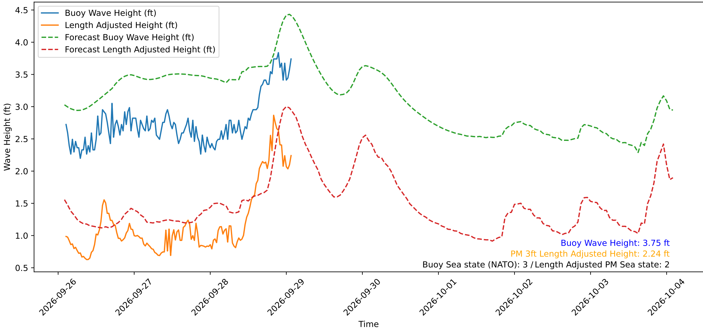
Wave Heights over Time for Red Beach at 2026-09-29 02:10:50
