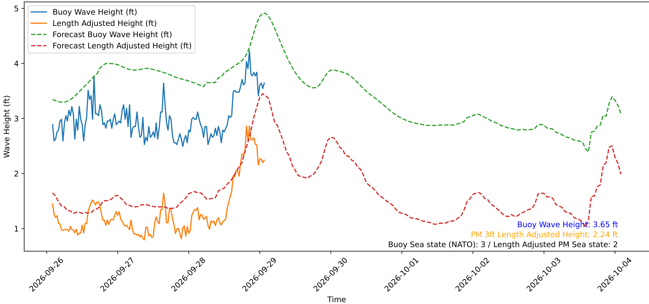
Wave Heights over Time for Oceanside Harbor at 2026-09-29 02:10:30
