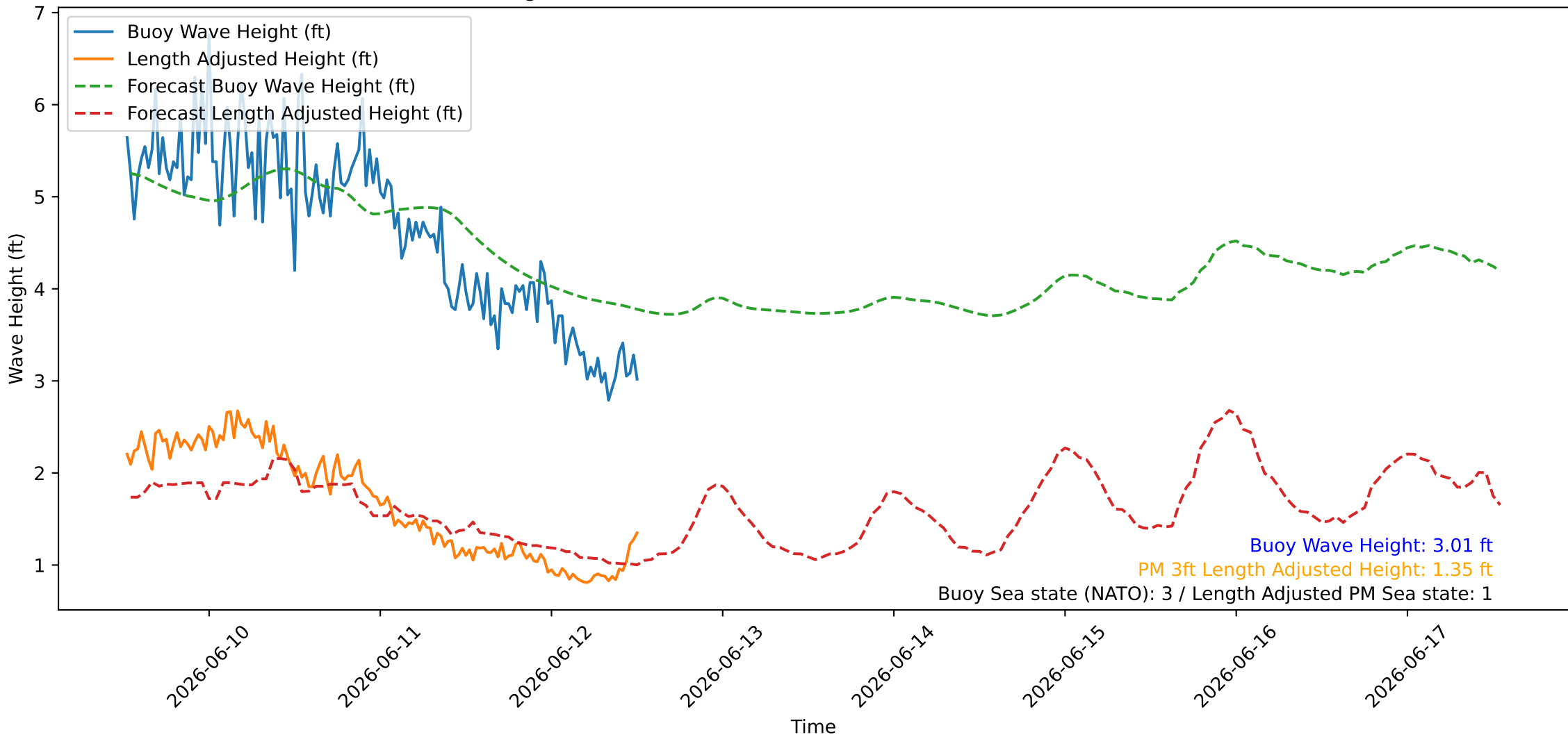
Wave Heights over Time for Oceanside Harbor at 2026-06-12 12:40:26
