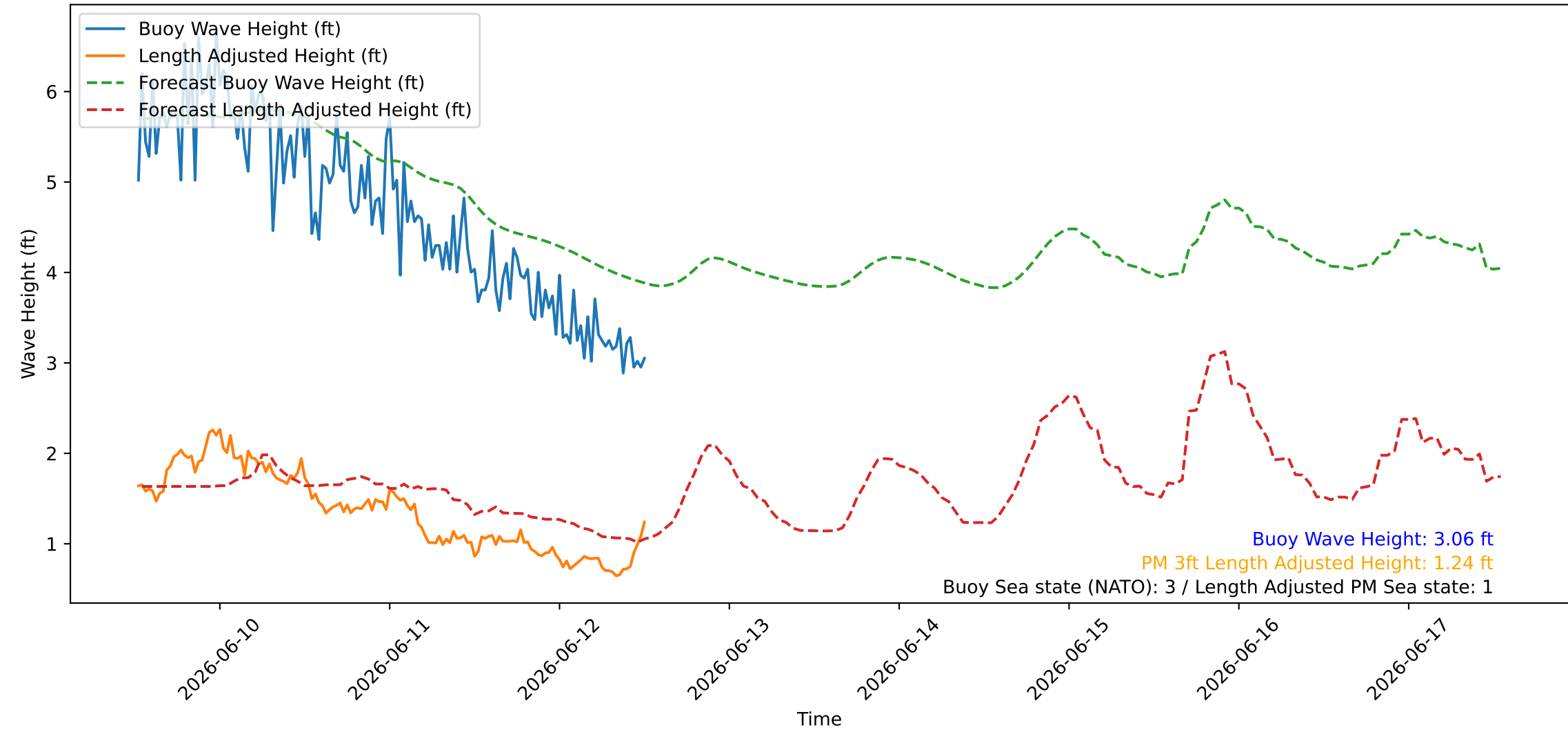
Wave Heights over Time for Green Beach at 2026-06-12 12:41:09
