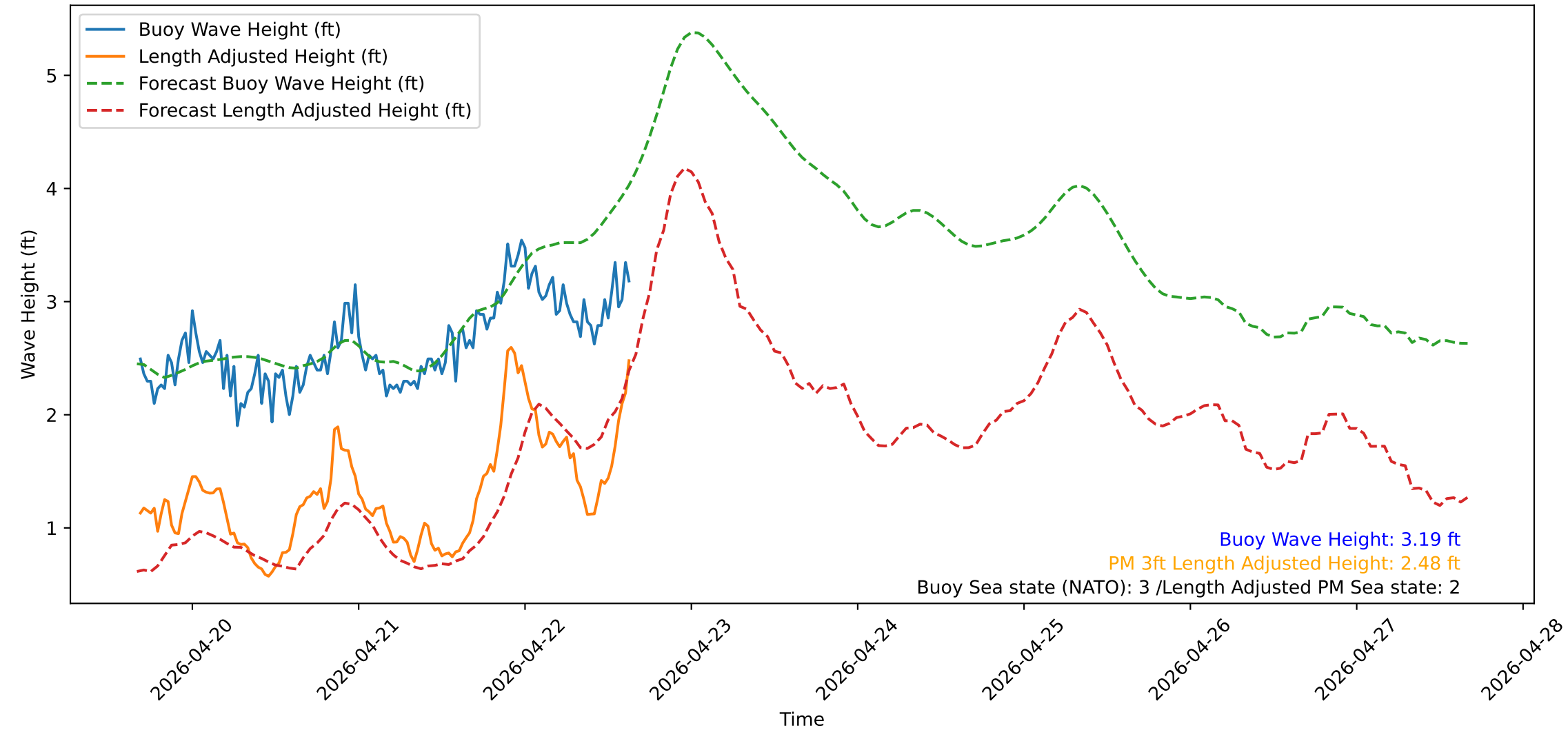
Wave Heights over Time for Green Beach at 2026-04-22 16:21:14
