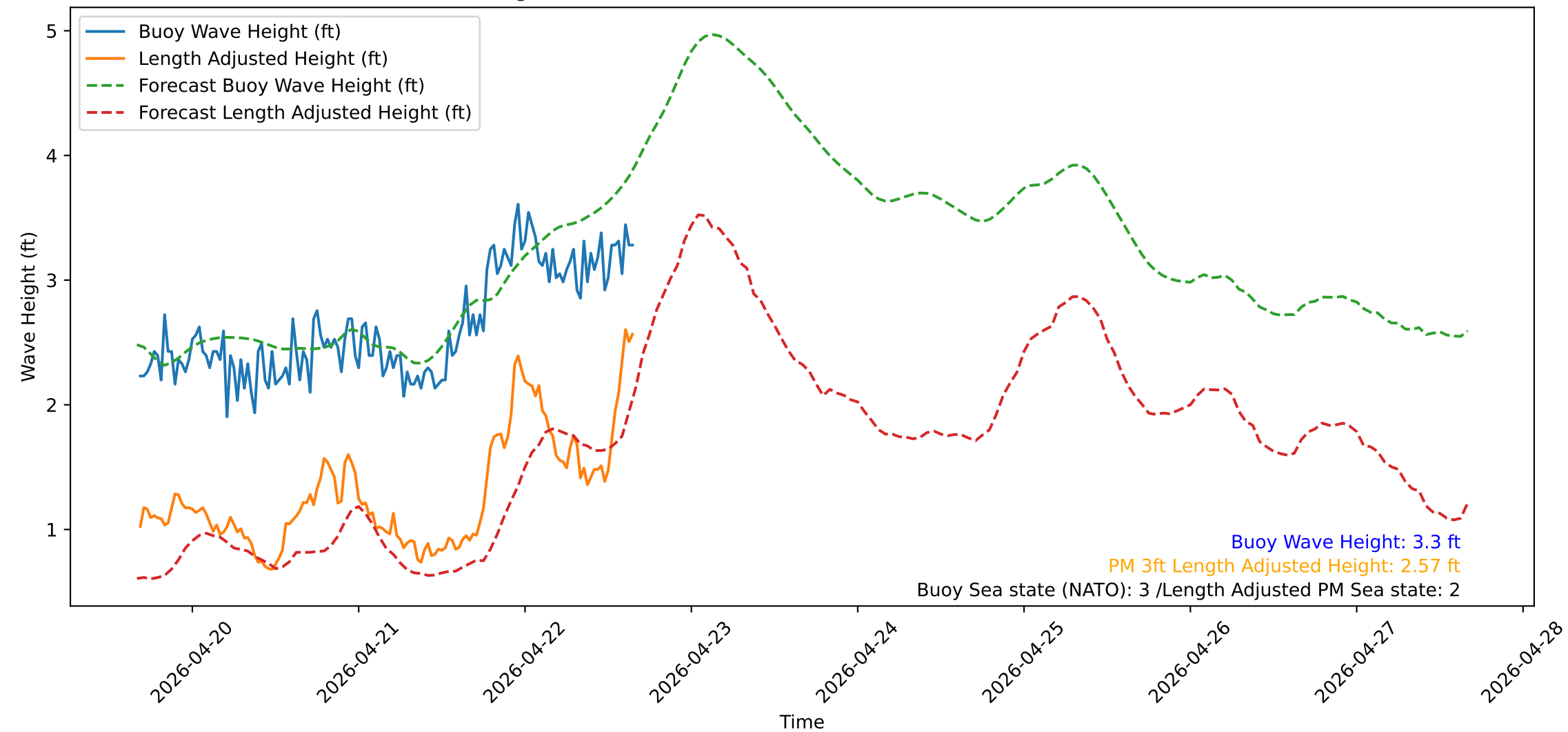
Wave Heights over Time for Oceanside Harbor at 2026-04-22 16:20:31
