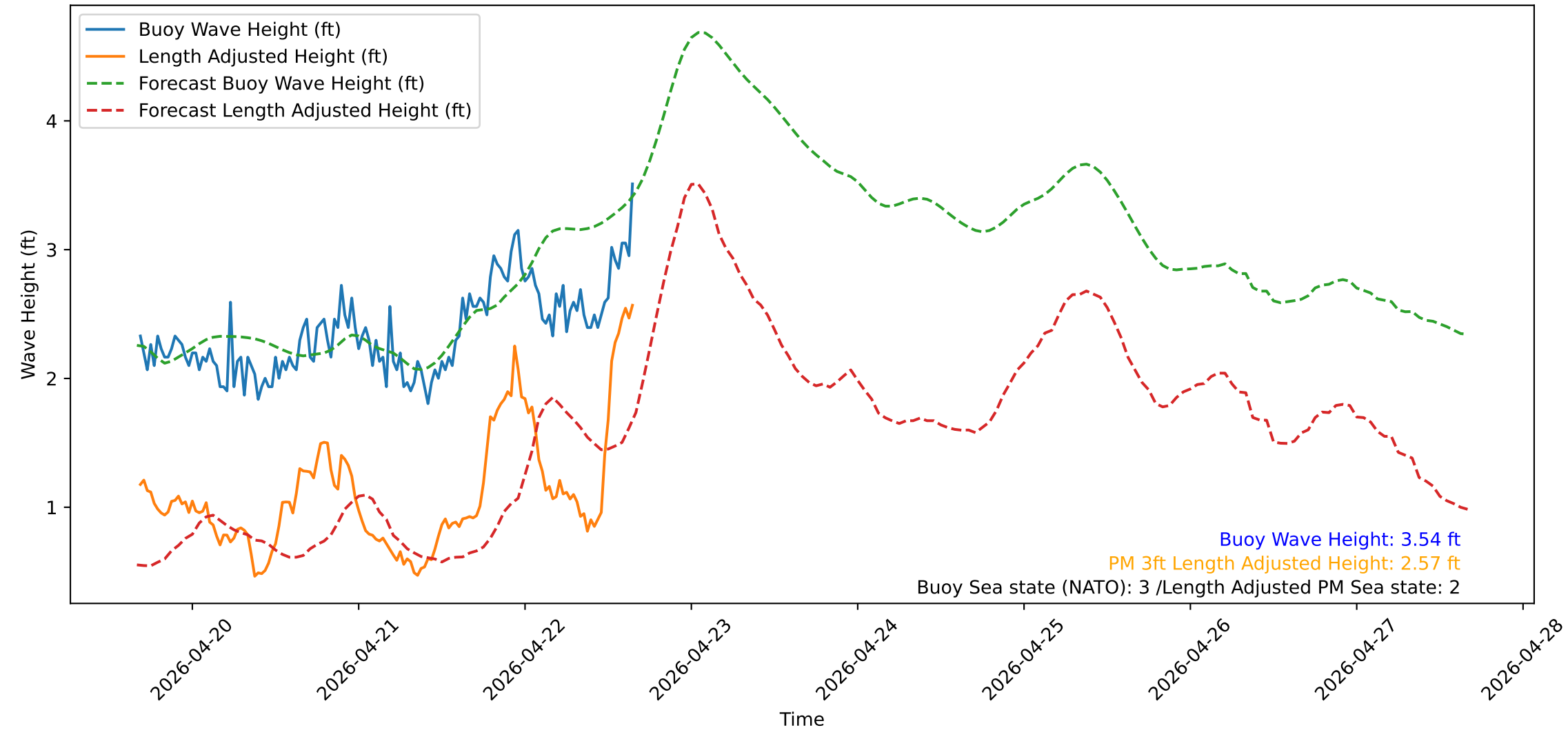
Wave Heights over Time for Red Beach at 2026-04-22 16:20:51
