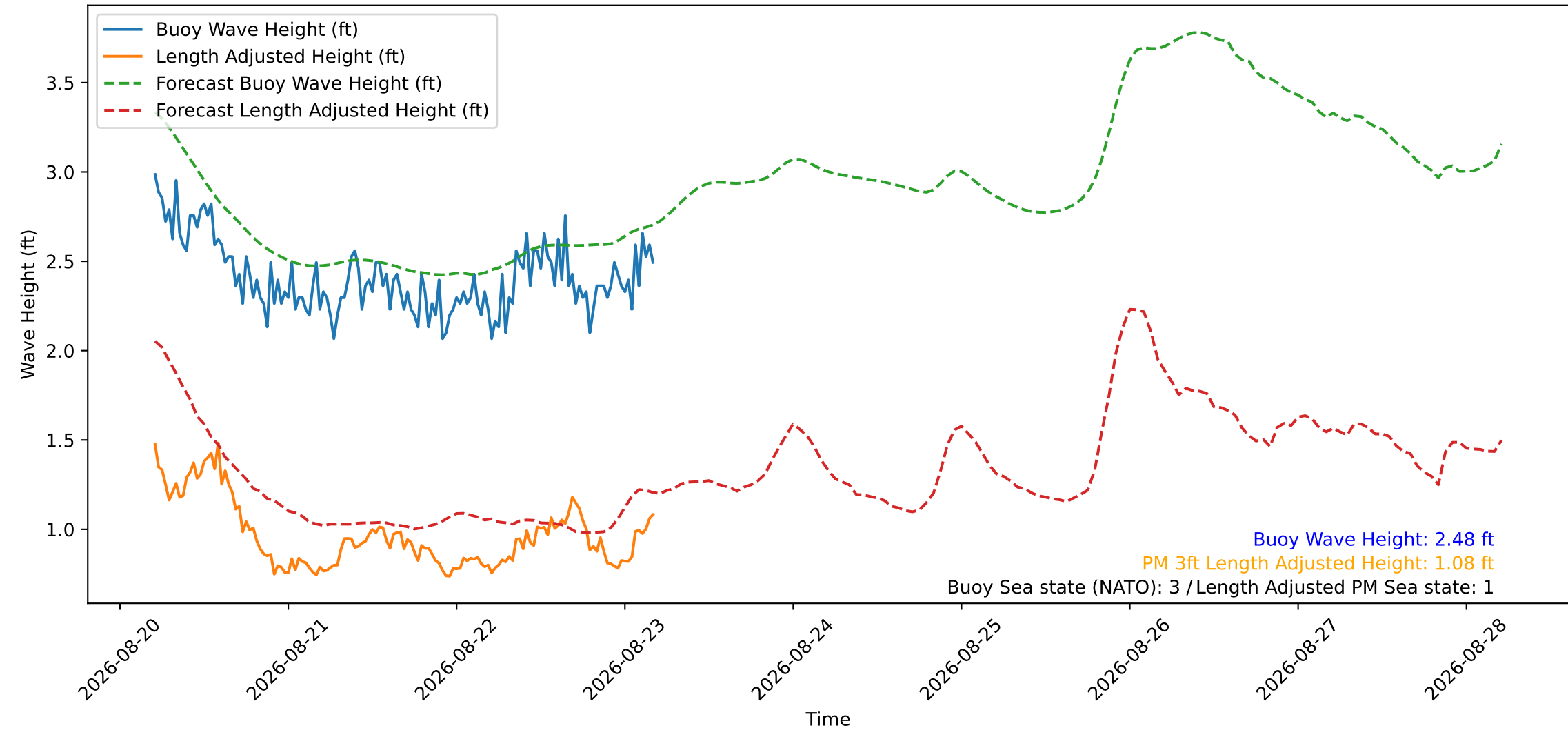
Wave Heights over Time for Red Beach at 2026-08-23 04:50:50
