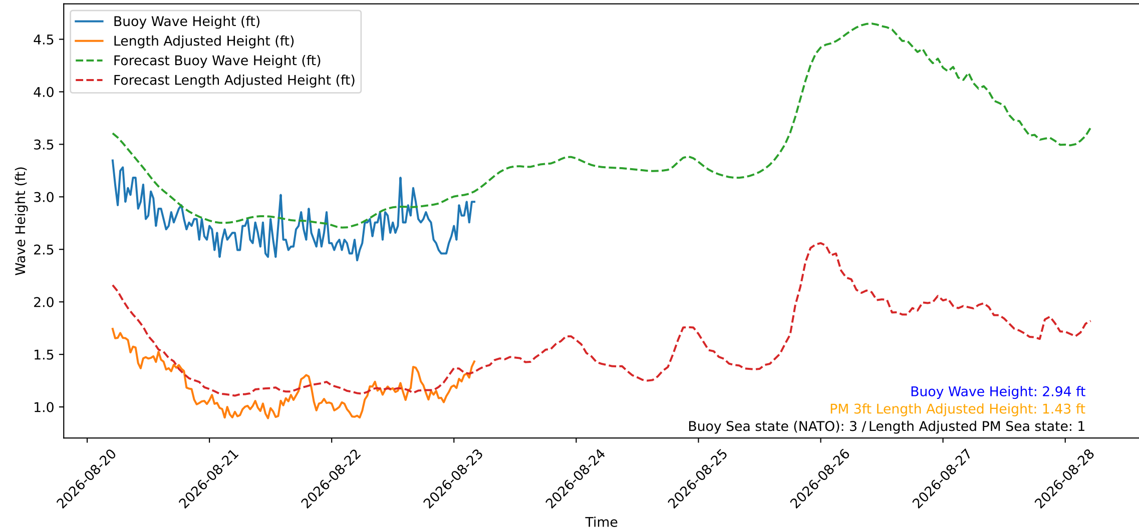
Wave Heights over Time for Green Beach at 2026-08-23 04:51:14
