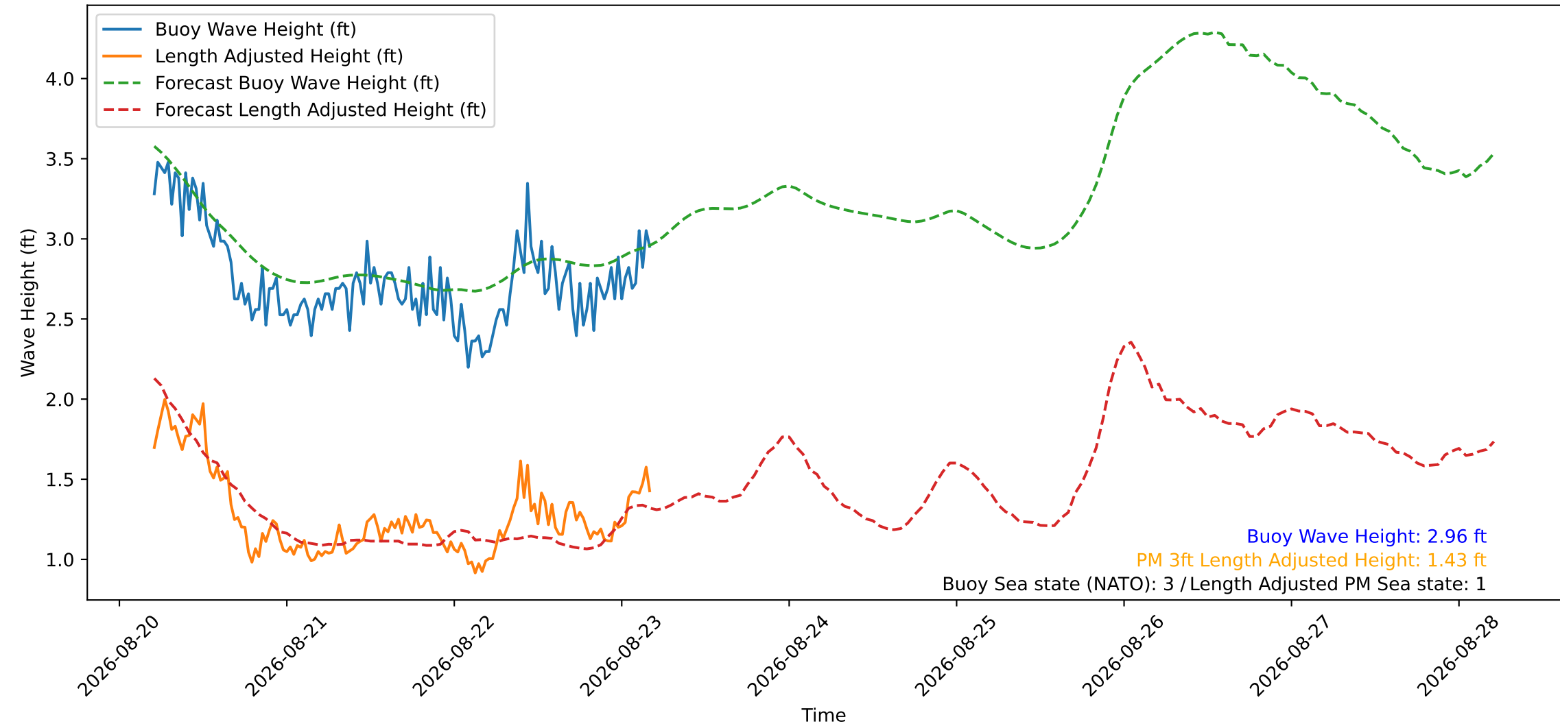
Wave Heights over Time for Oceanside Harbor at 2026-08-23 04:50:30
