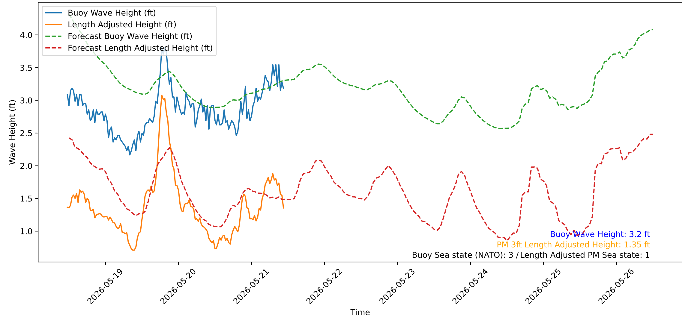
Wave Heights over Time for Green Beach at 2026-05-21 11:31:14
