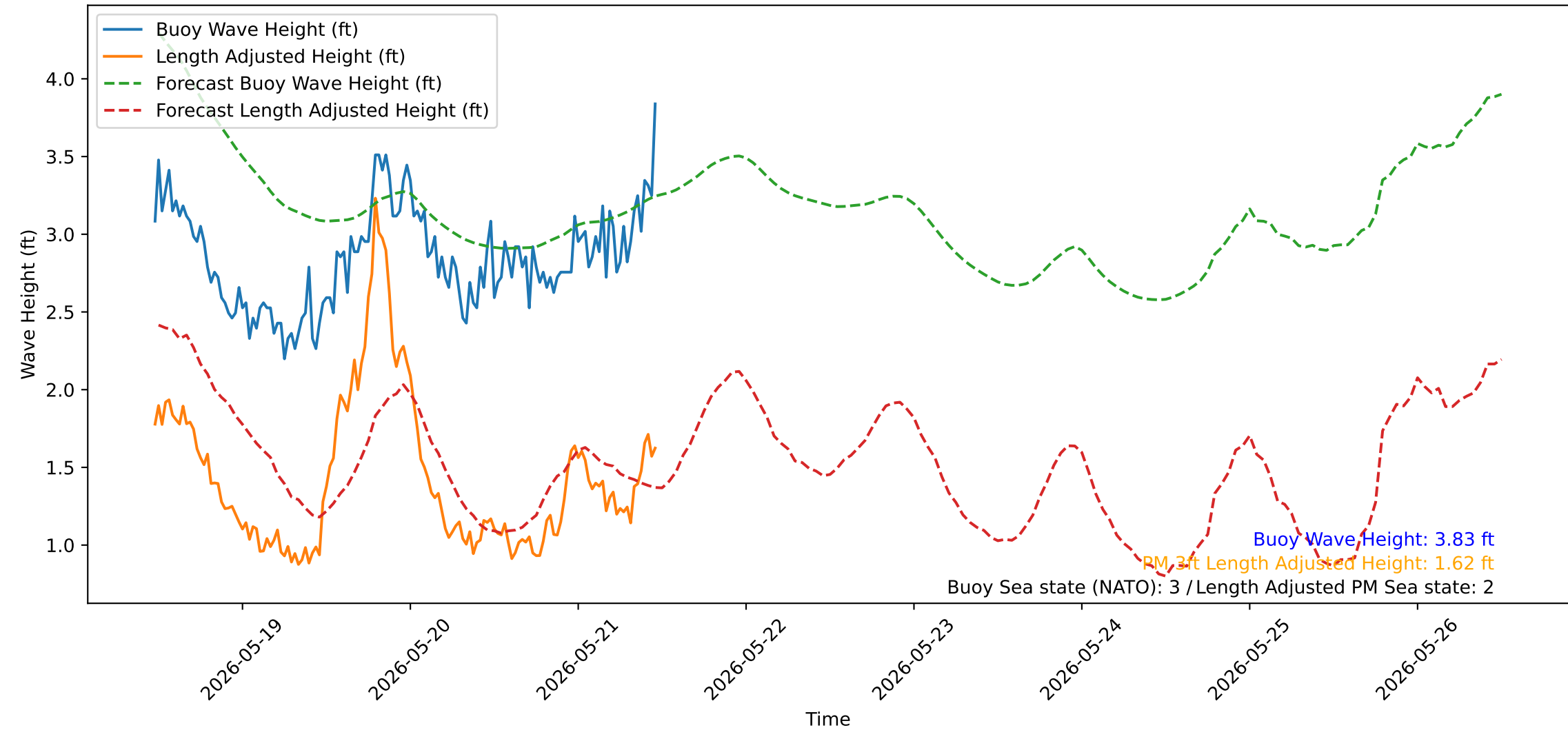
Wave Heights over Time for Oceanside Harbor at 2026-05-21 11:30:31
