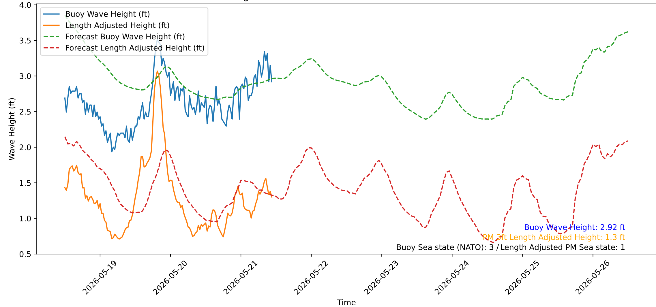
Wave Heights over Time for Red Beach at 2026-05-21 11:30:51
