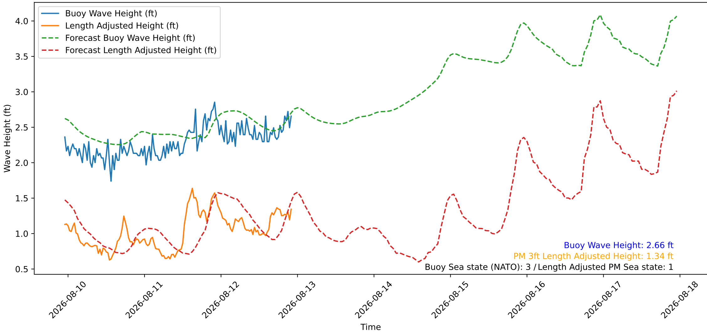
Wave Heights over Time for Red Beach at 2026-08-12 22:50:47
