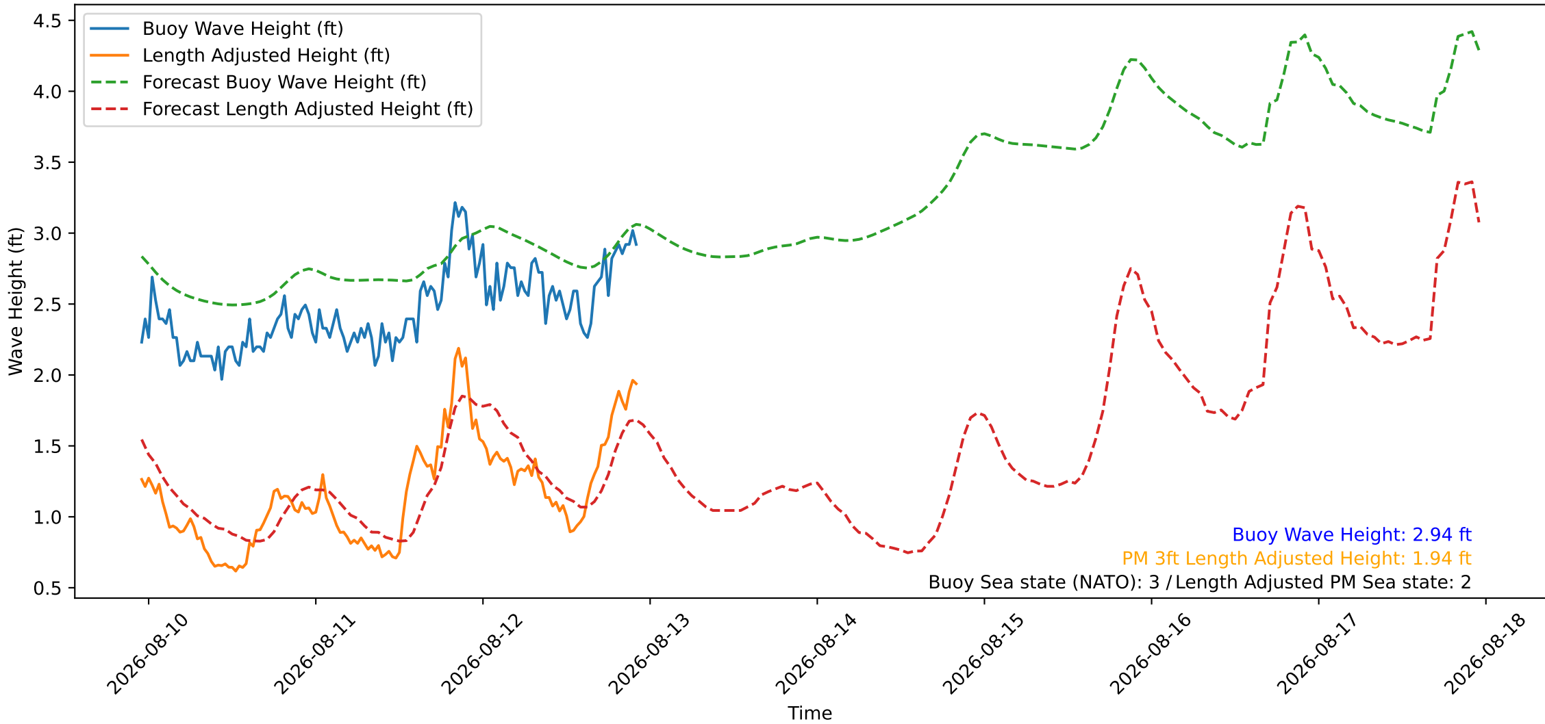
Wave Heights over Time for Green Beach at 2026-08-12 22:51:09
