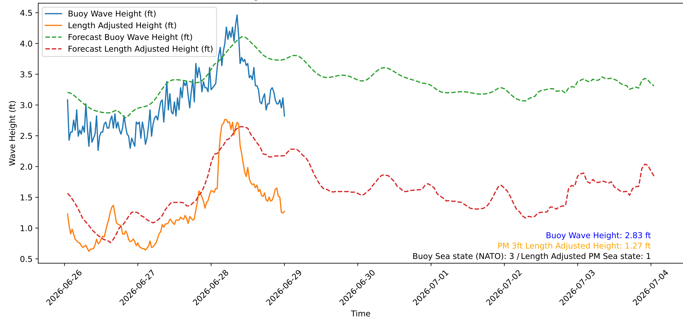
Wave Heights over Time for Red Beach at 2026-06-29 00:40:46
