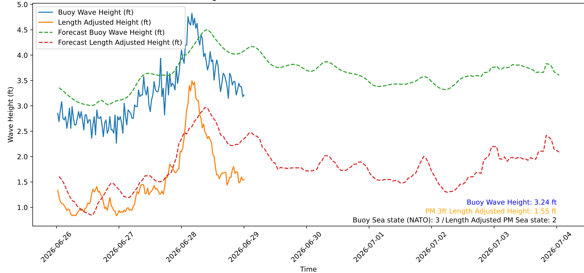
Wave Heights over Time for Green Beach at 2026-06-29 00:41:09
