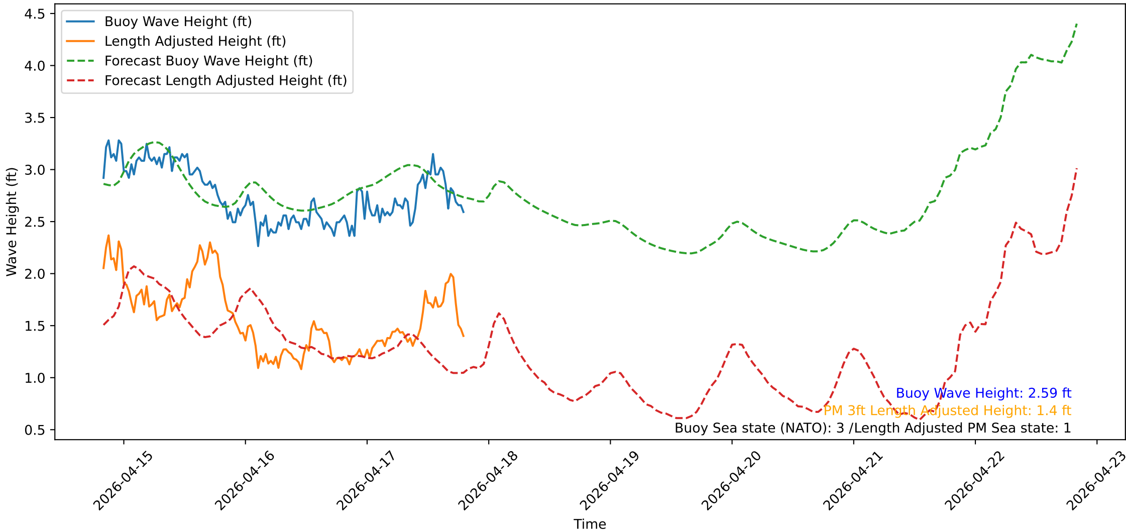
Wave Heights over Time for Red Beach at 2026-04-17 19:50:52
