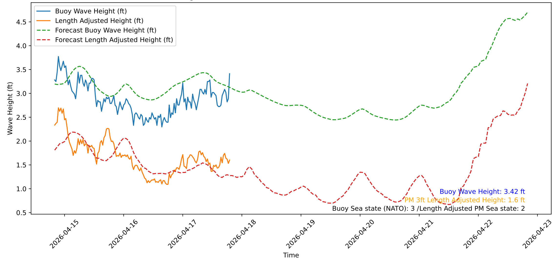
Wave Heights over Time for Oceanside Harbor at 2026-04-17 19:50:32
