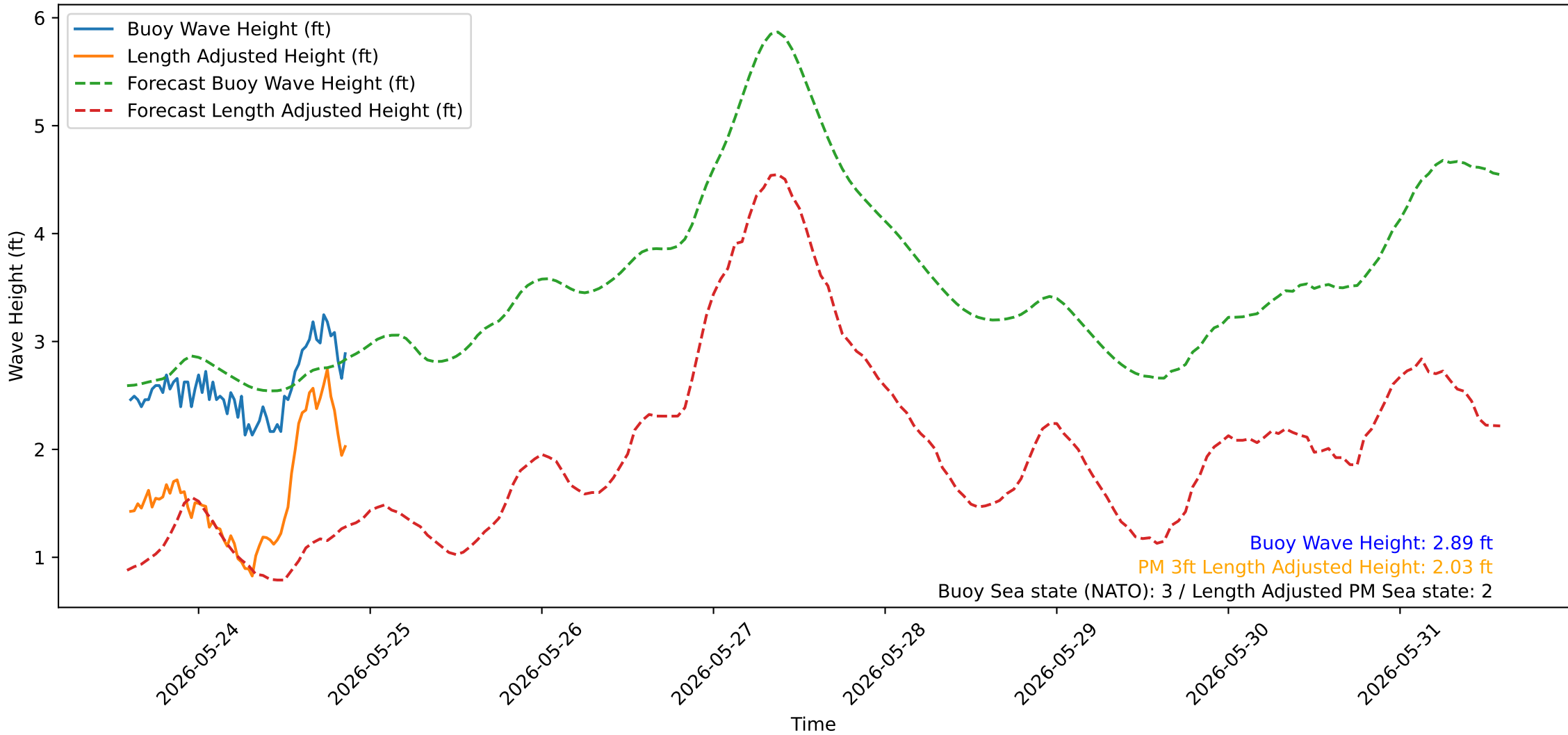
Wave Heights over Time for Oceanside Harbor at 2026-05-26 14:20:28
