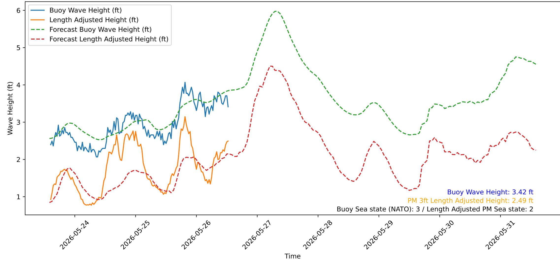
Wave Heights over Time for Green Beach at 2026-05-26 14:21:10
