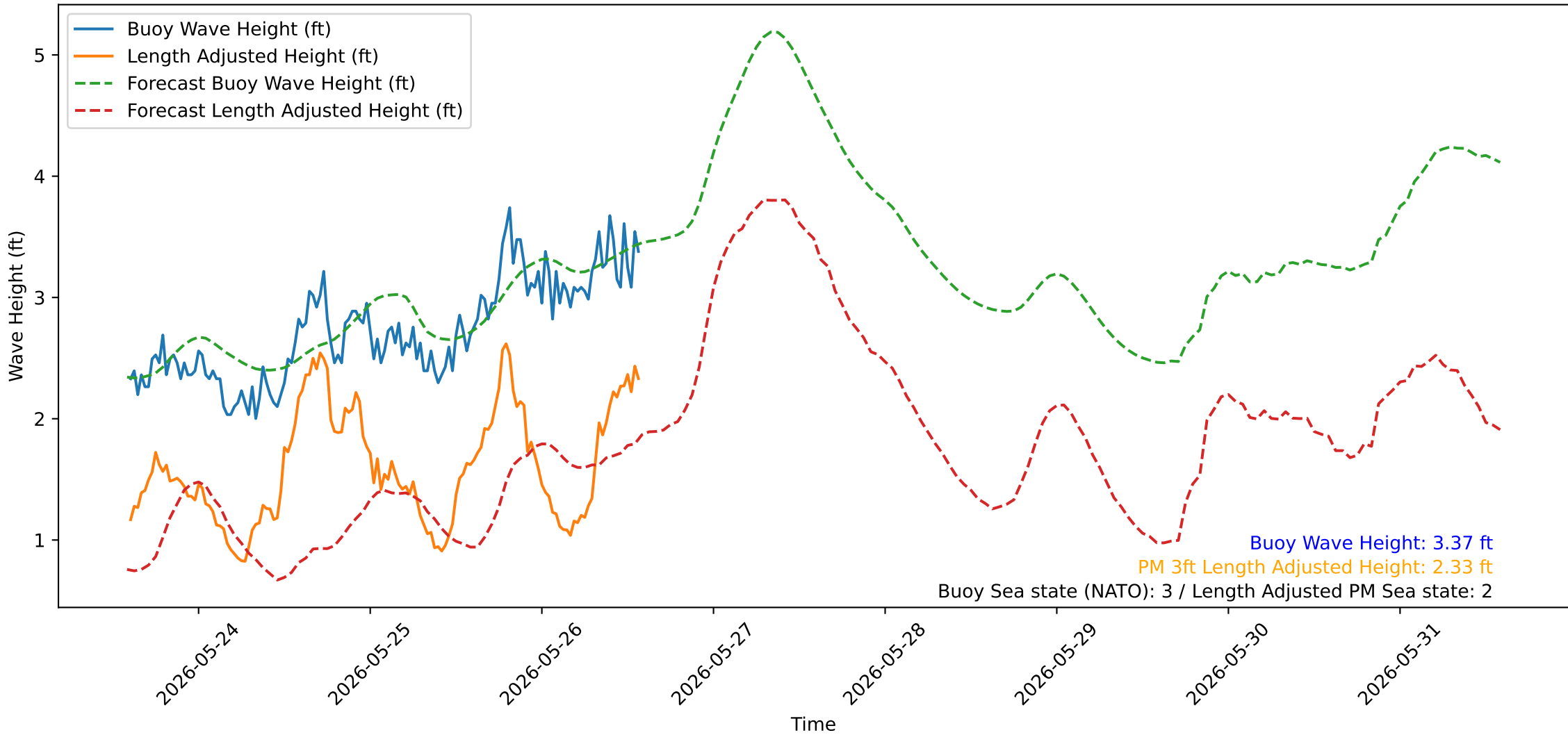
Wave Heights over Time for Red Beach at 2026-05-26 14:20:48
