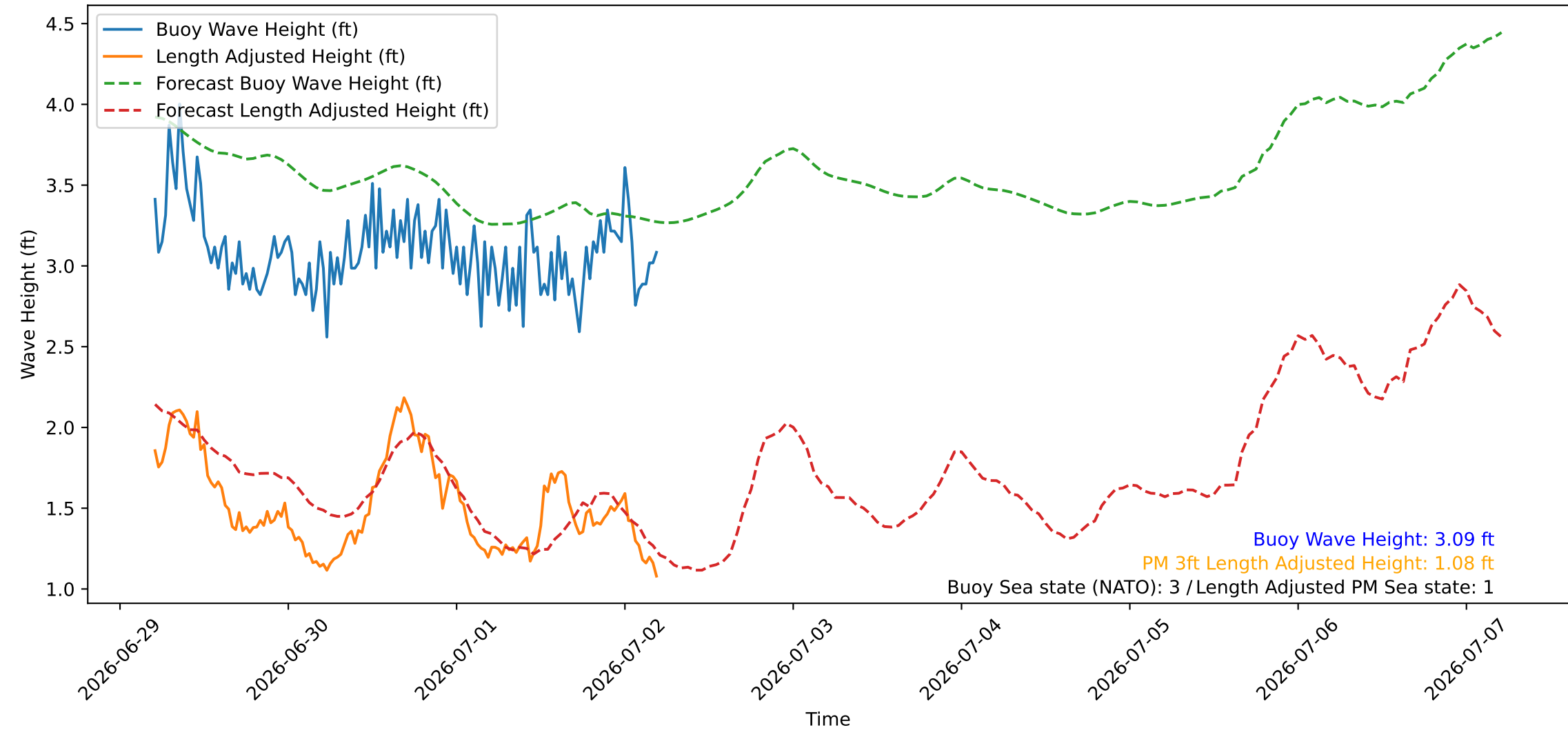
Wave Heights over Time for Oceanside Harbor at 2026-07-02 05:10:26
