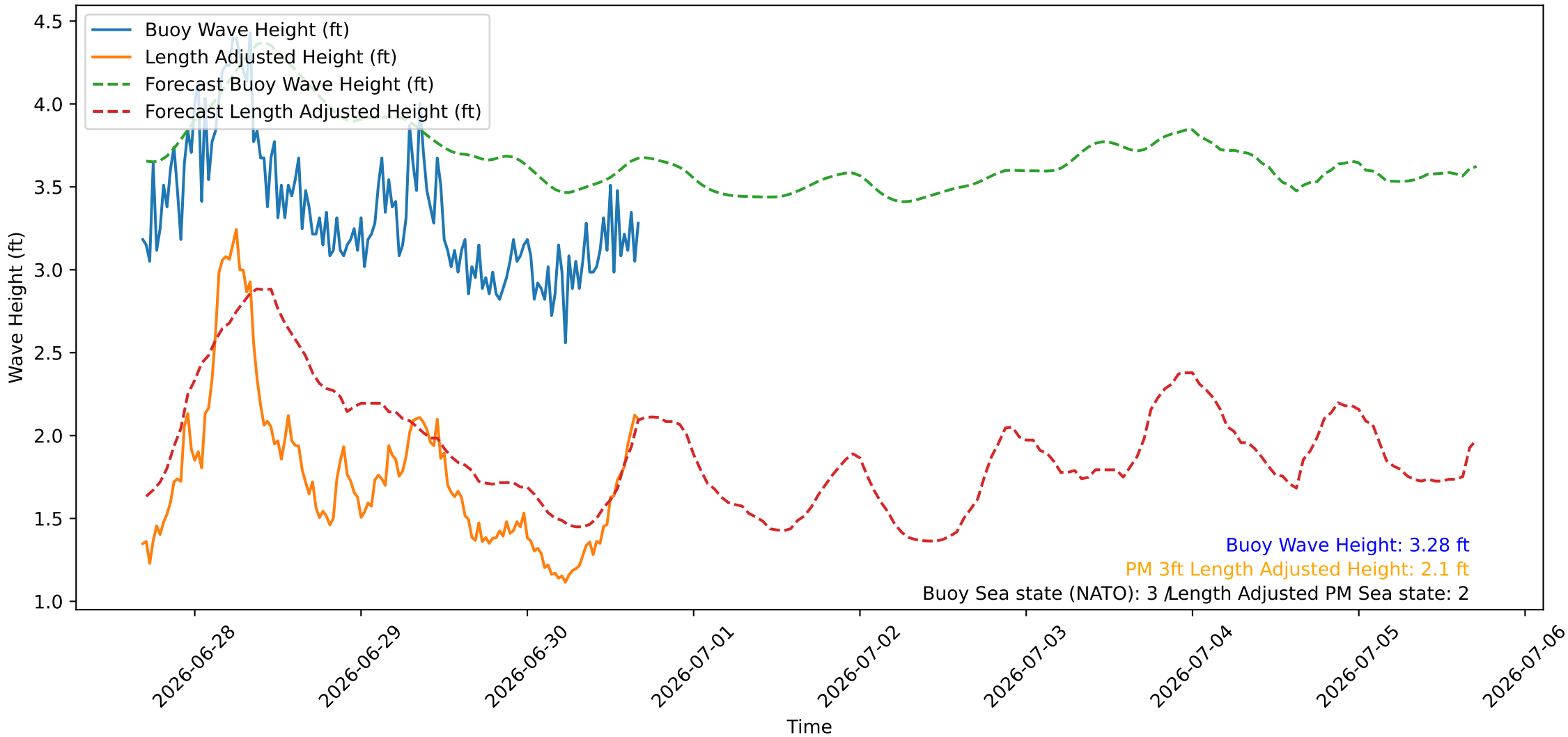
Wave Heights over Time for Oceanside Harbor at 2026-06-30 16:40:26
