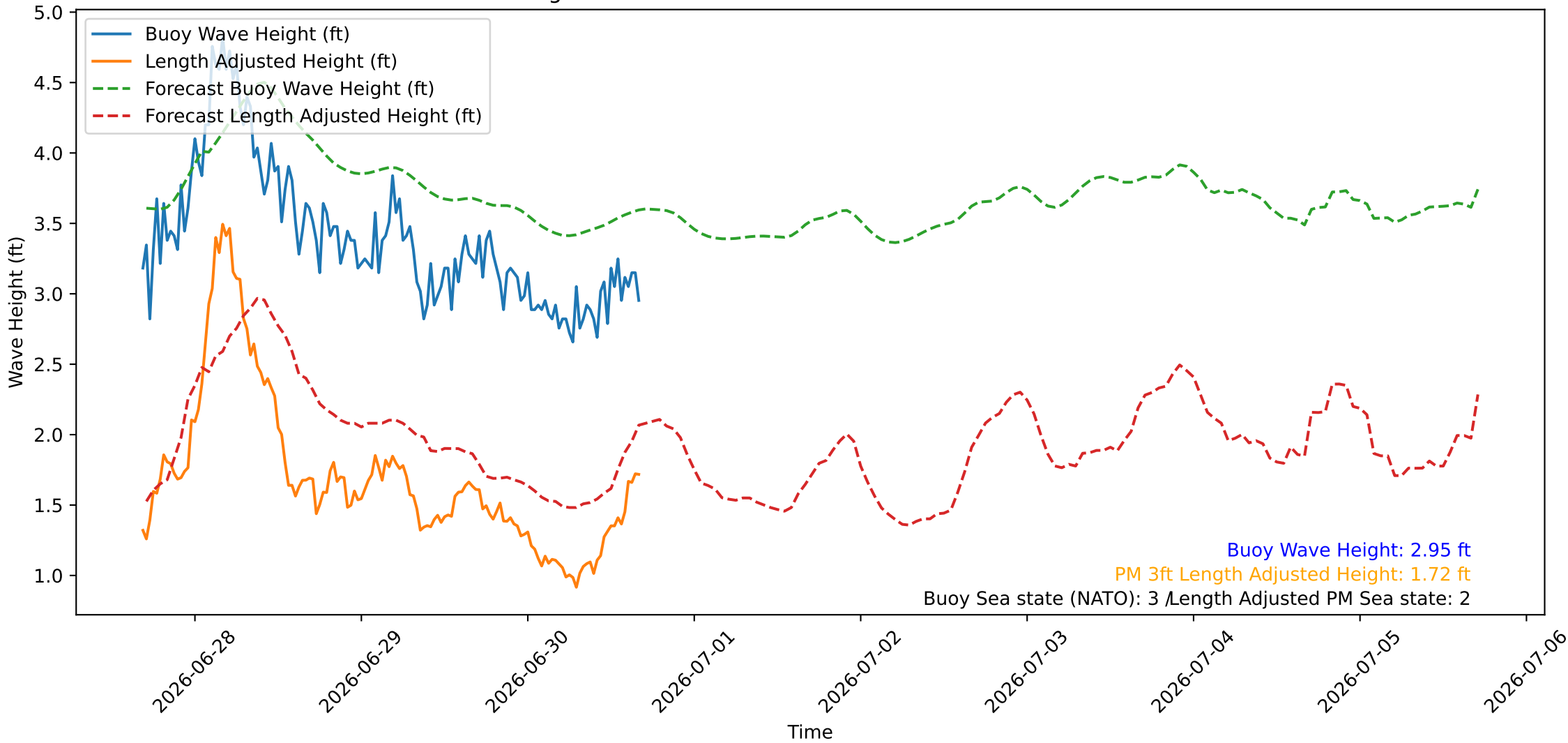
Wave Heights over Time for Green Beach at 2026-06-30 16:41:08
