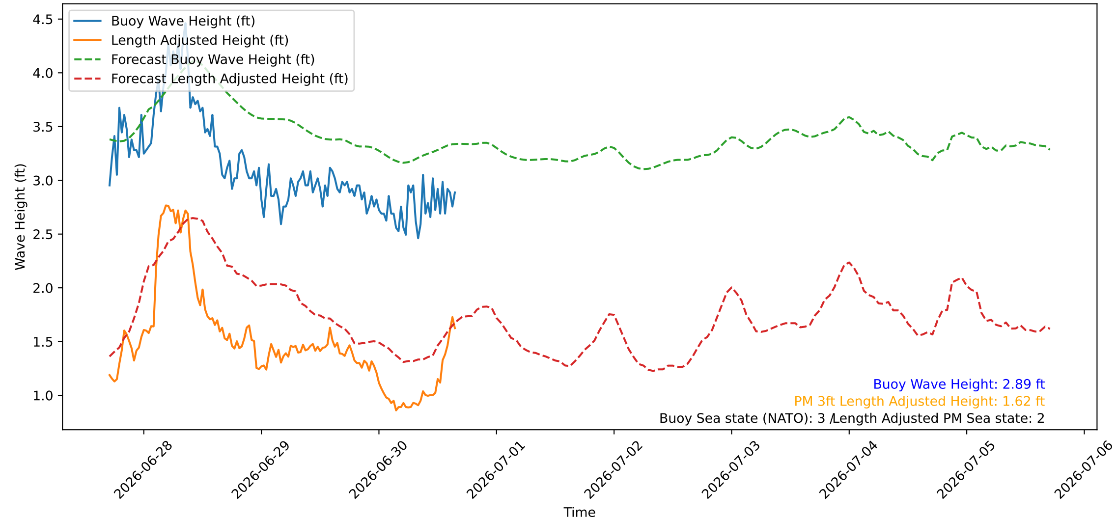
Wave Heights over Time for Red Beach at 2026-06-30 16:40:45
