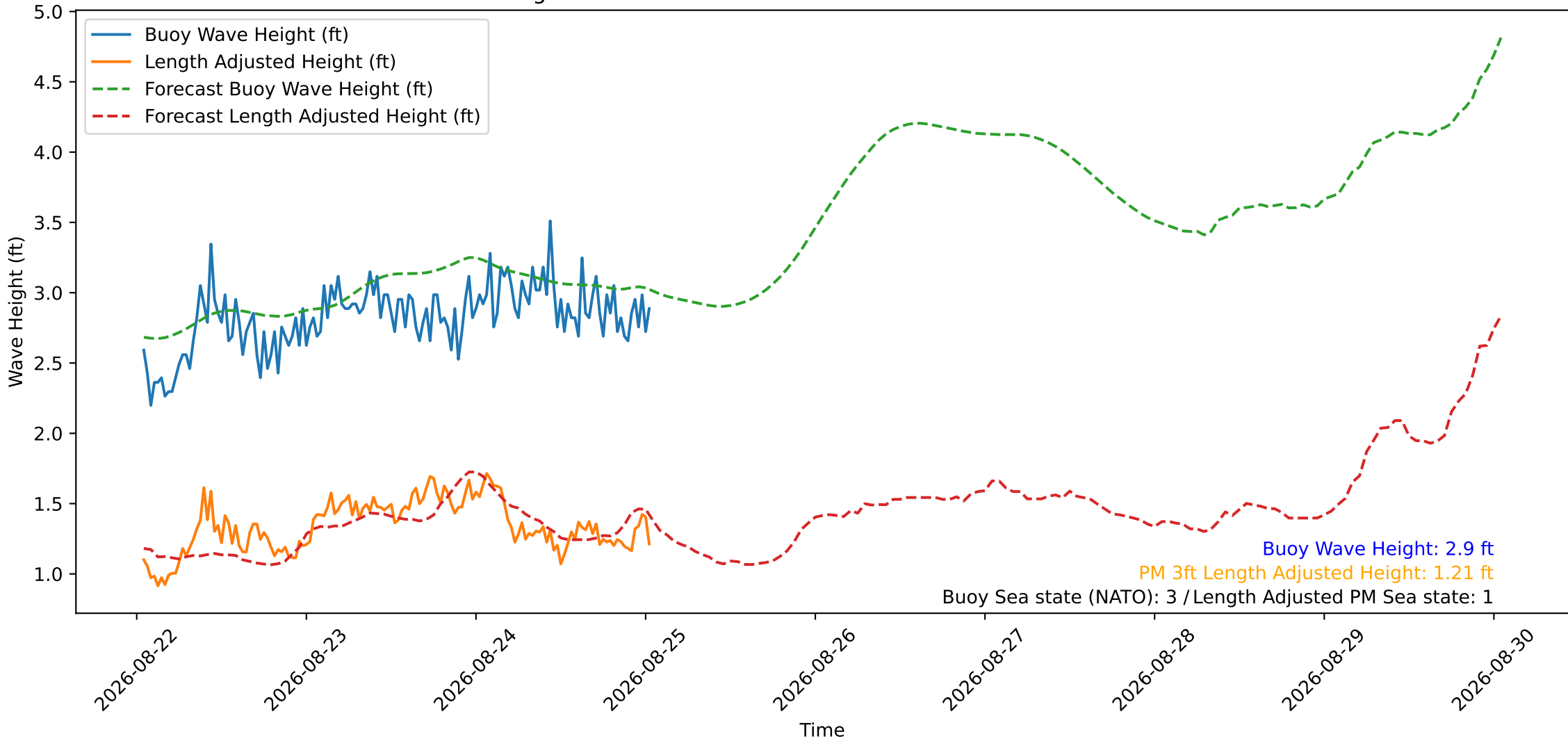
Wave Heights over Time for Oceanside Harbor at 2026-08-25 01:10:29
