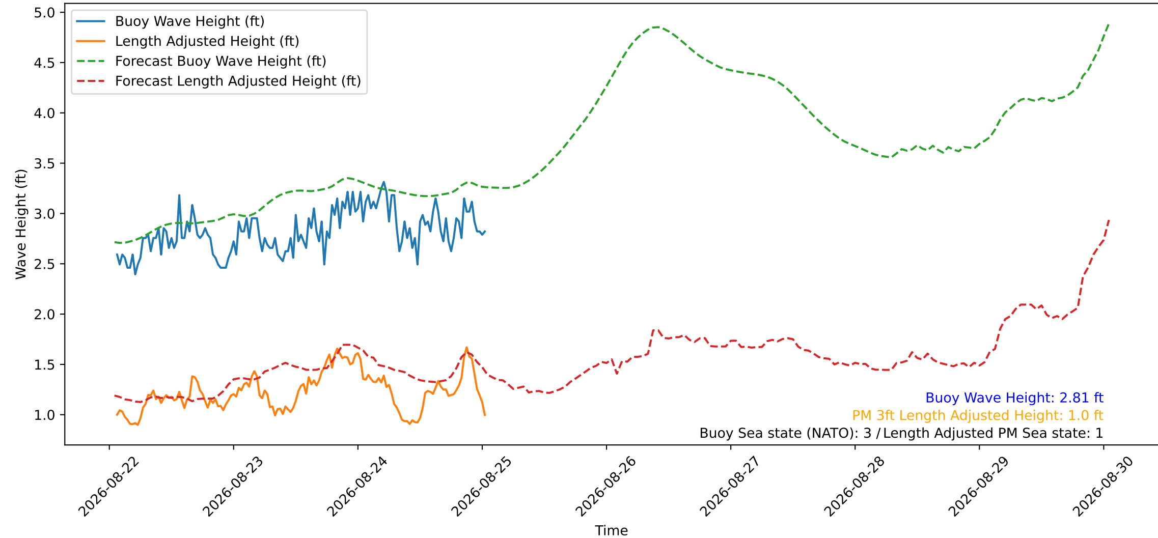
Wave Heights over Time for Green Beach at 2026-08-25 01:11:11
