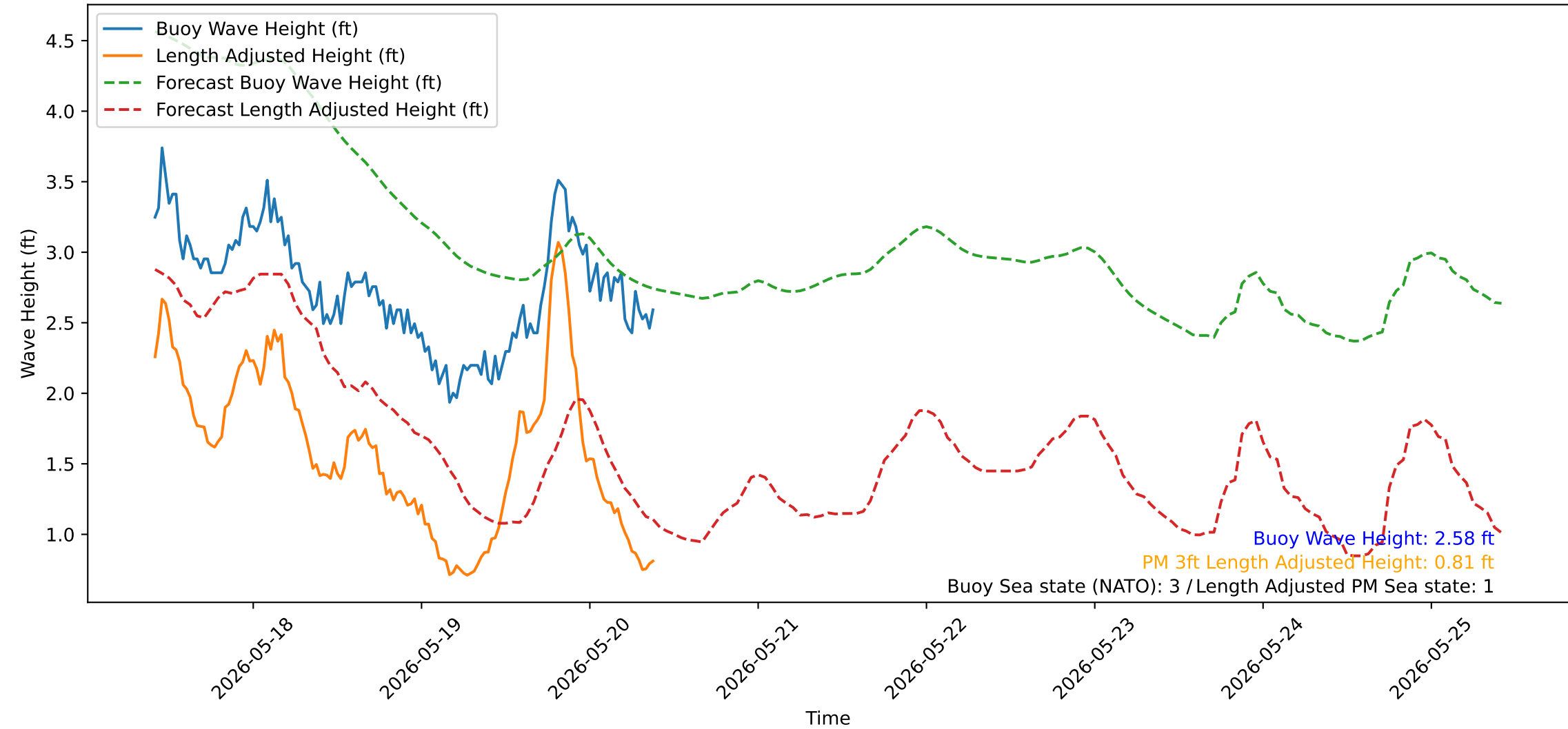
Wave Heights over Time for Red Beach at 2026-05-20 09:40:50
