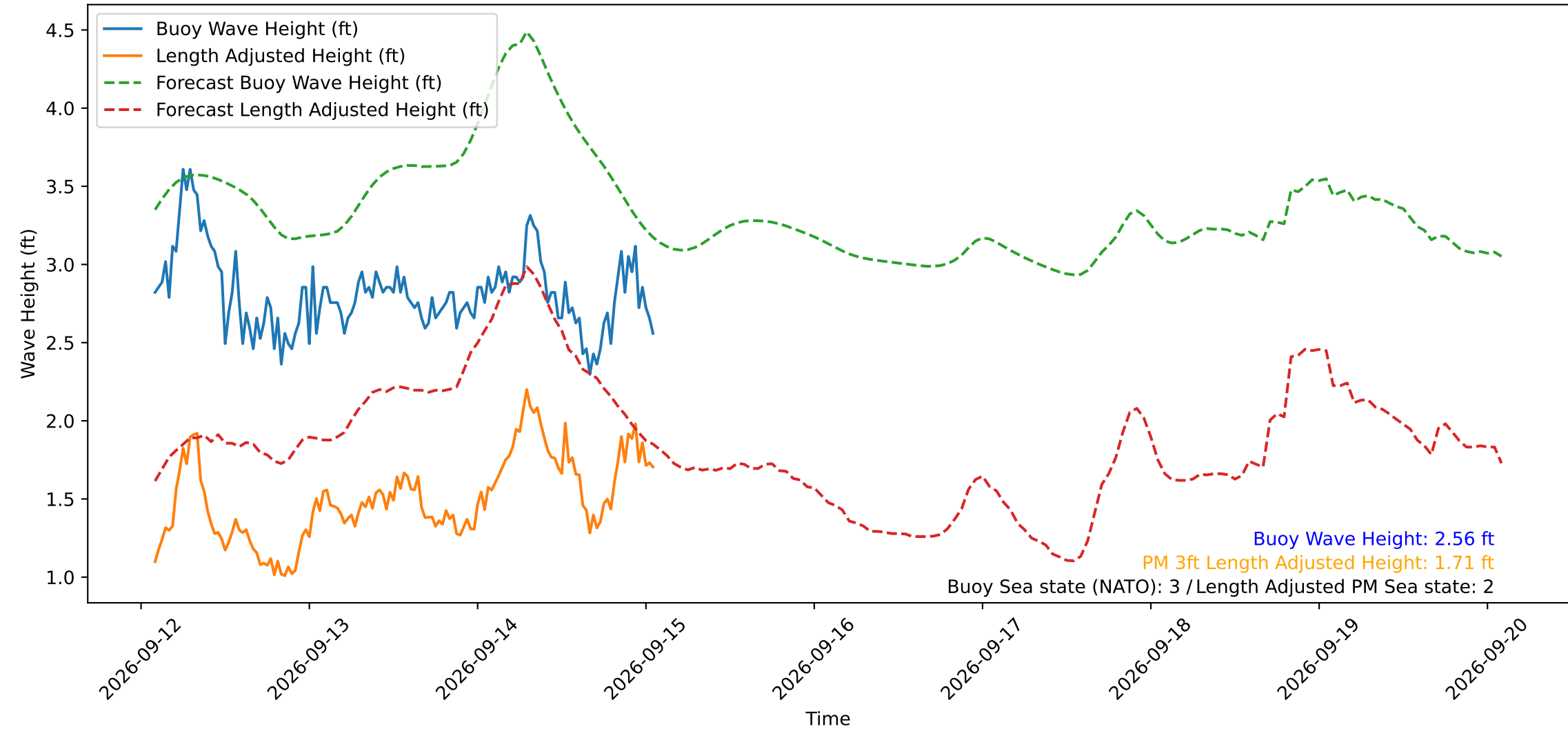
Wave Heights over Time for Green Beach at 2026-09-15 01:41:11
