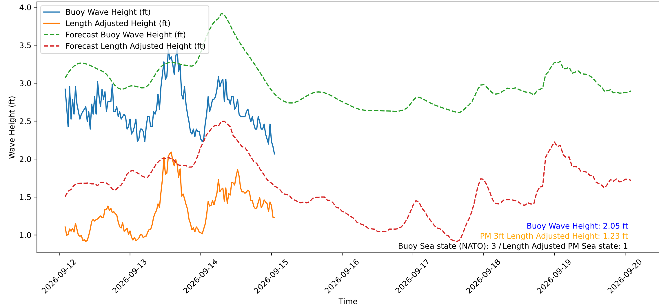
Wave Heights over Time for Red Beach at 2026-09-15 01:40:49
