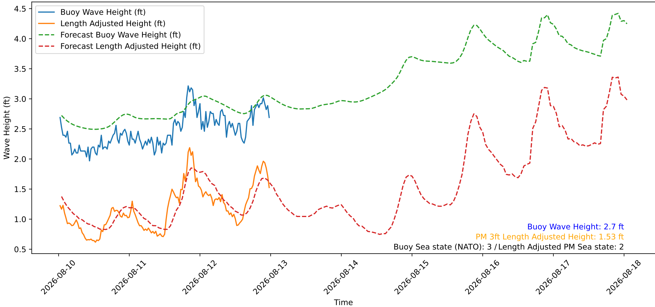
Wave Heights over Time for Green Beach at 2026-08-13 00:41:09
