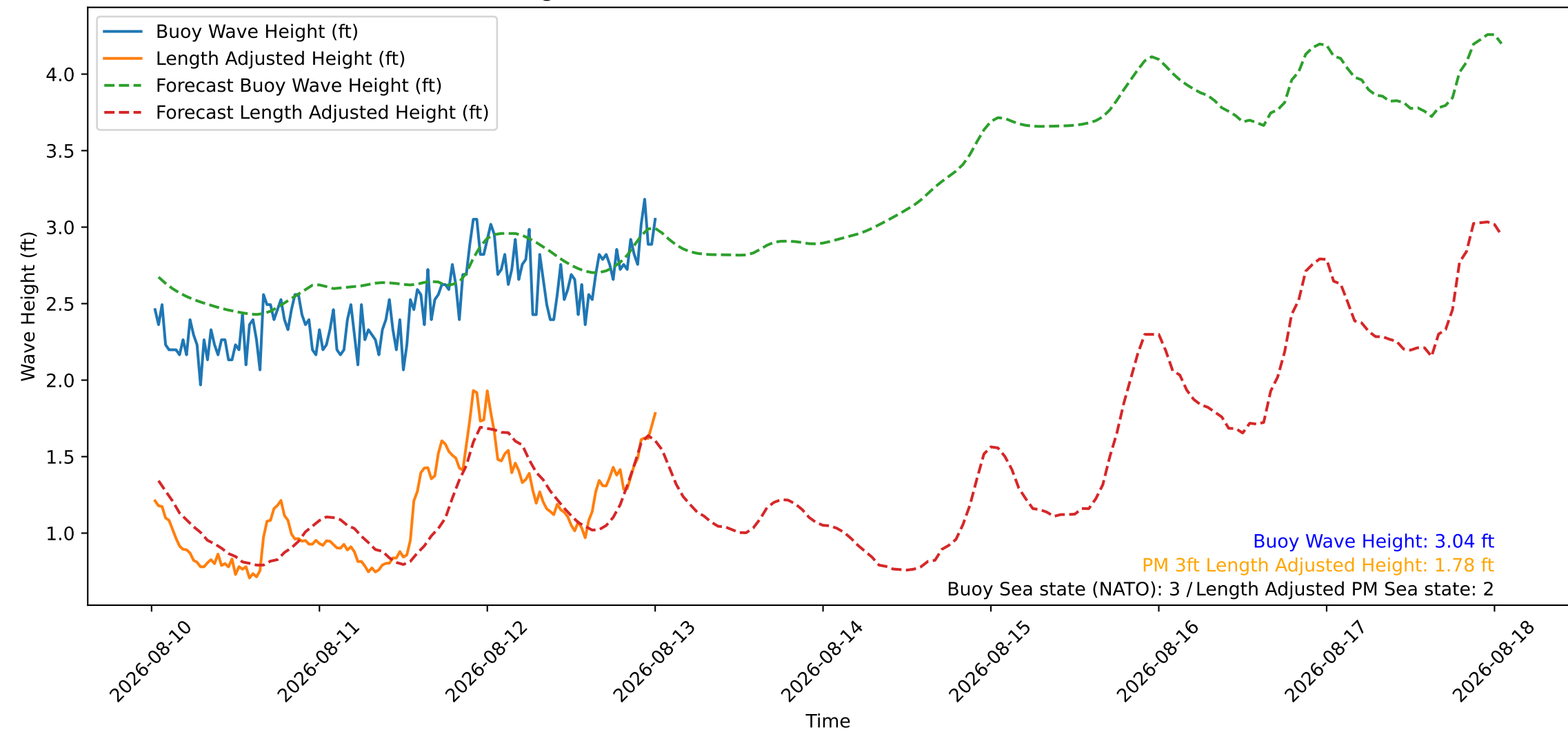
Wave Heights over Time for Oceanside Harbor at 2026-08-13 00:40:26
