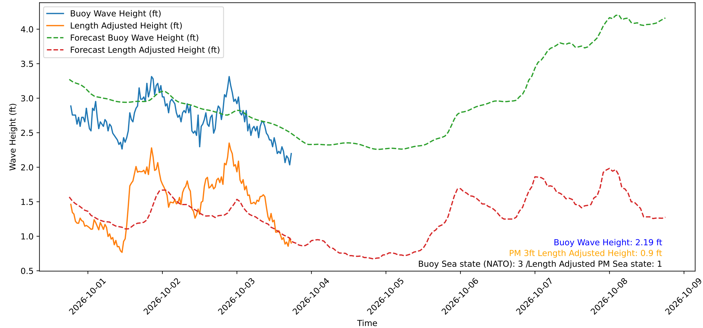
Wave Heights over Time for Oceanside Harbor at 2026-10-03 18:20:29
