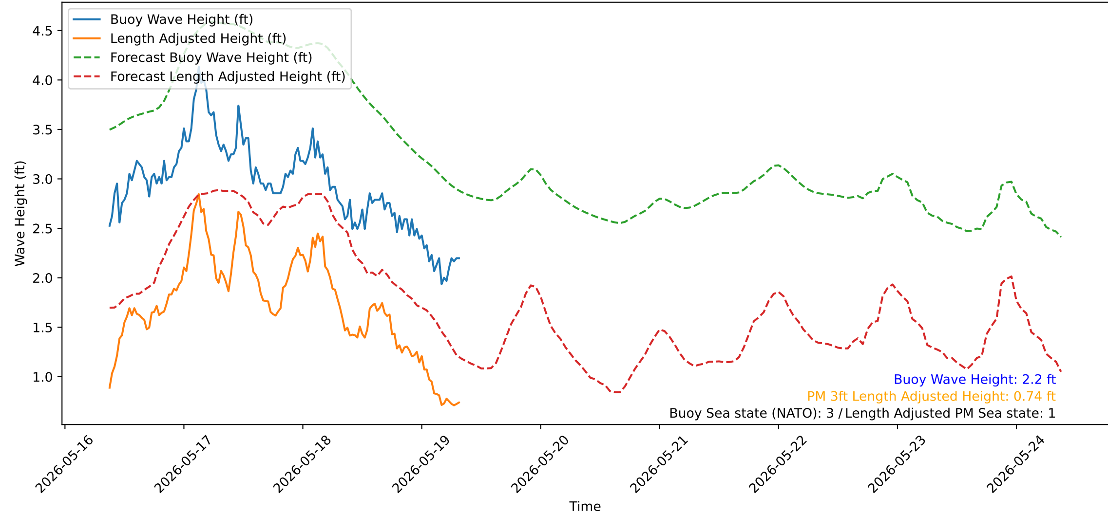
Wave Heights over Time for Red Beach at 2026-05-19 08:30:52
