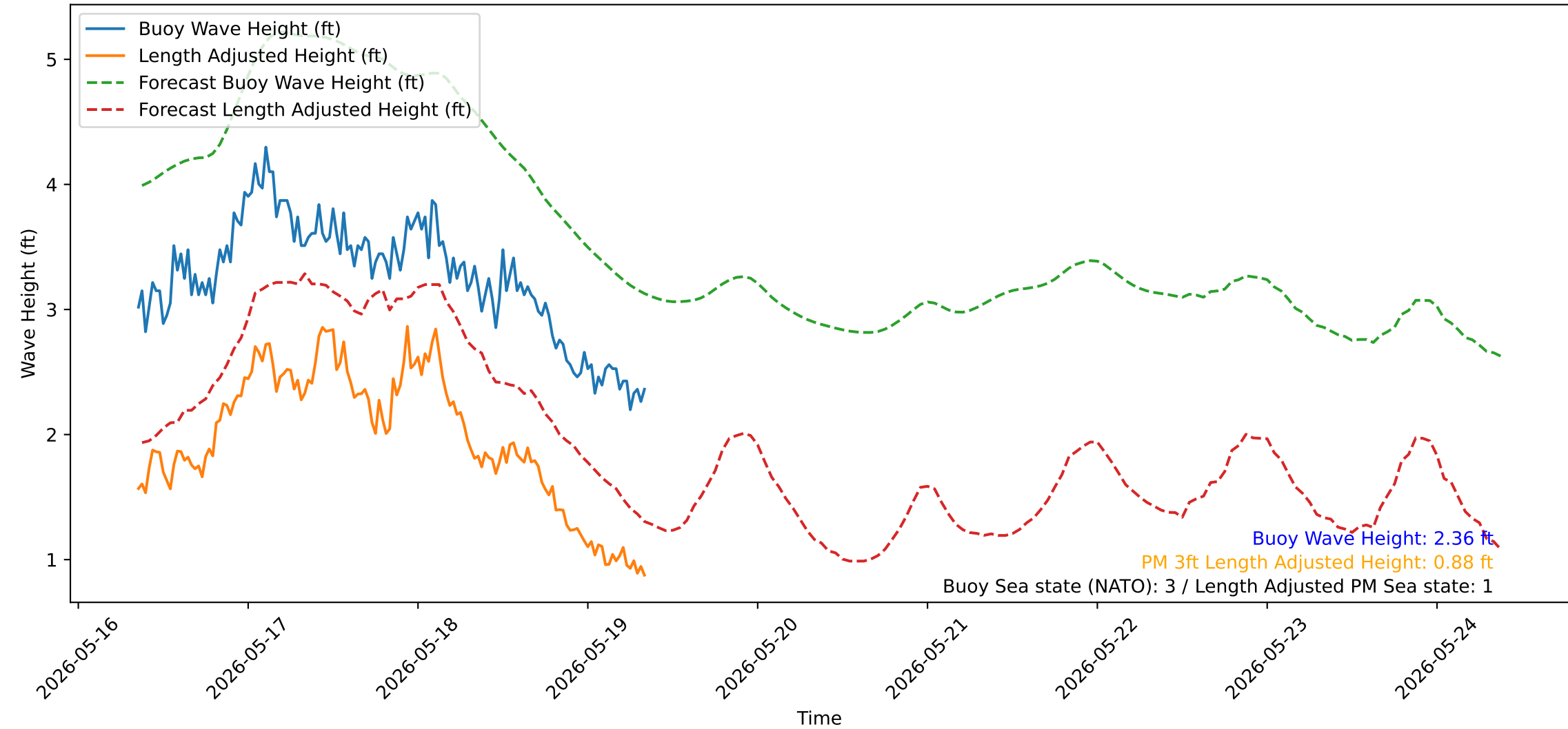
Wave Heights over Time for Oceanside Harbor at 2026-05-19 08:30:32
