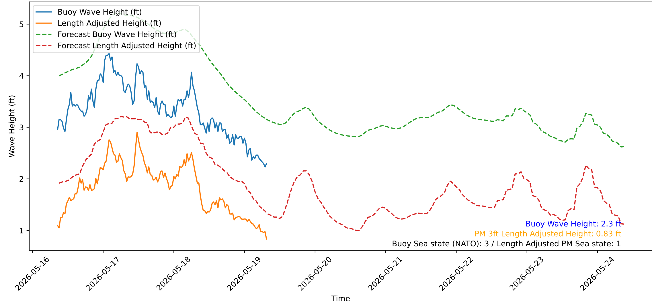
Wave Heights over Time for Green Beach at 2026-05-19 08:31:15
